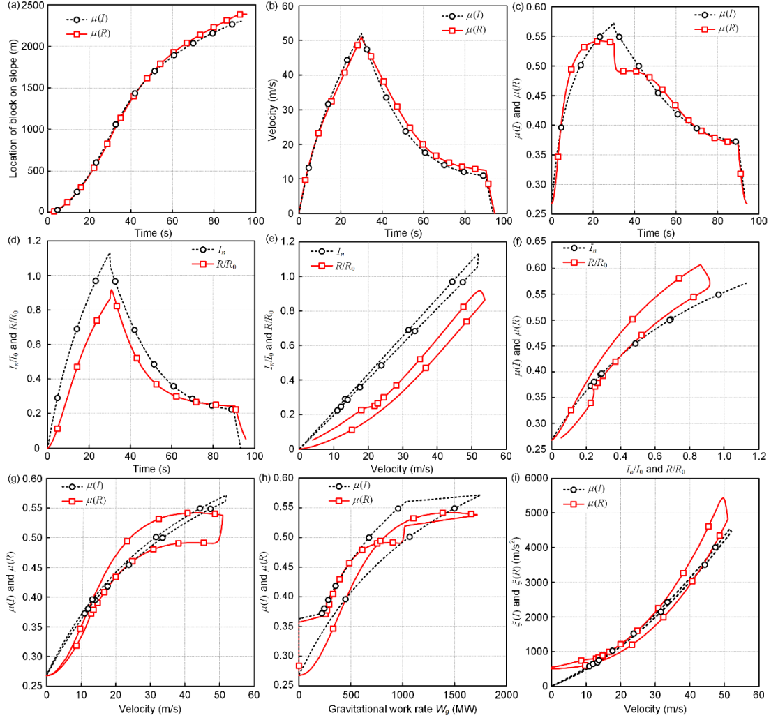
Figure 3. Comparison between the \mu(I) vs \mu(R) rheologies. (a)-(c) show the calculated location of center-of-mass, velocity and friction of the two rheologies. (d)-(e) Comparison between I_n/I_0 and R/R_0 over time and flow velocity. (f) Calculated friction \mu(I) vs \mu(R) as a function of I_n/I_0 and R/R_0 . (g)-(h) Calculated \mu(I) vs \mu(R) as a function of the velocity and gravitational work rate. (i) Comparison between \xi(I) (Eq. 7) and \xi(R) .
