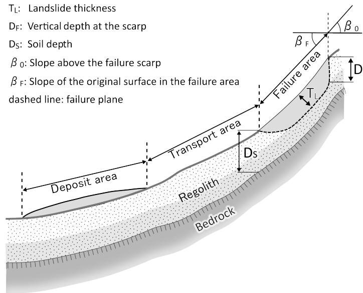
Figure 1. Schematic representation of a shallow landslide with its failure, transport, and deposit area, including important definitions used in this study. Different shades in the regolith indicate differing properties.
