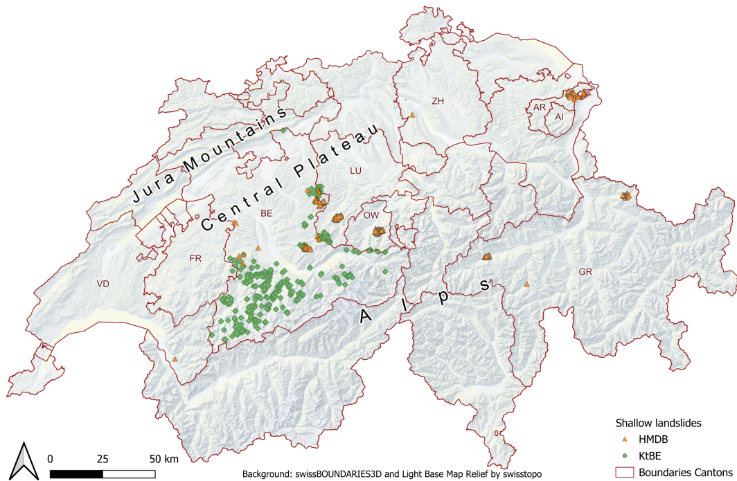
Figure 2. Map of the recorded shallow landslide locations across Switzerland for the HMDB (orange triangles) and KtBE (green diamonds) datasets. Background: swissBOUNDARIES3D (Swisstopo, 2024b) and light base map relief (Swisstopo, 2024c)
