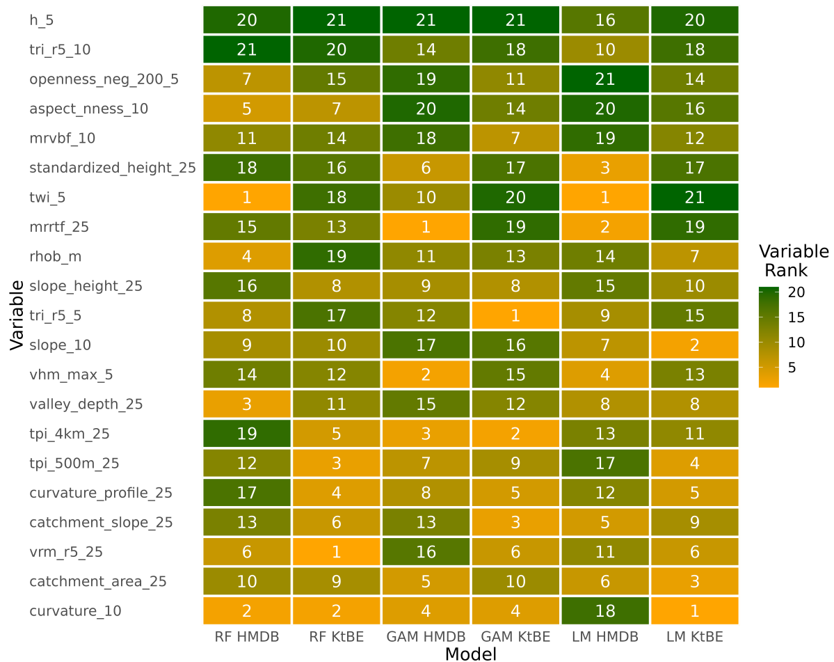
Figure B1. Heatmap showing the overall variable importance extracted from 10-fold cross validation for the RF and LM models and the importance of the best fit for the GAM model. The number in the cells and their colour correspond to the importance rank of the variable within the model, with 21 (green) being the most important and 1 (yellow) being the least important variable. The variables are sorted by the sum of the ranks of each row.
