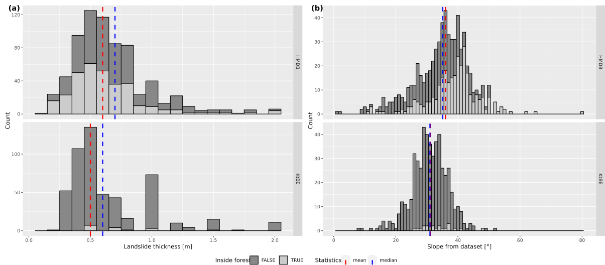
Figure 4. Histograms showing the distribution of (a) the landslide thickness and (b) the mean slope values in the release areas recorded in the HMDB (upper row) and KtBE (lower row) datasets.
