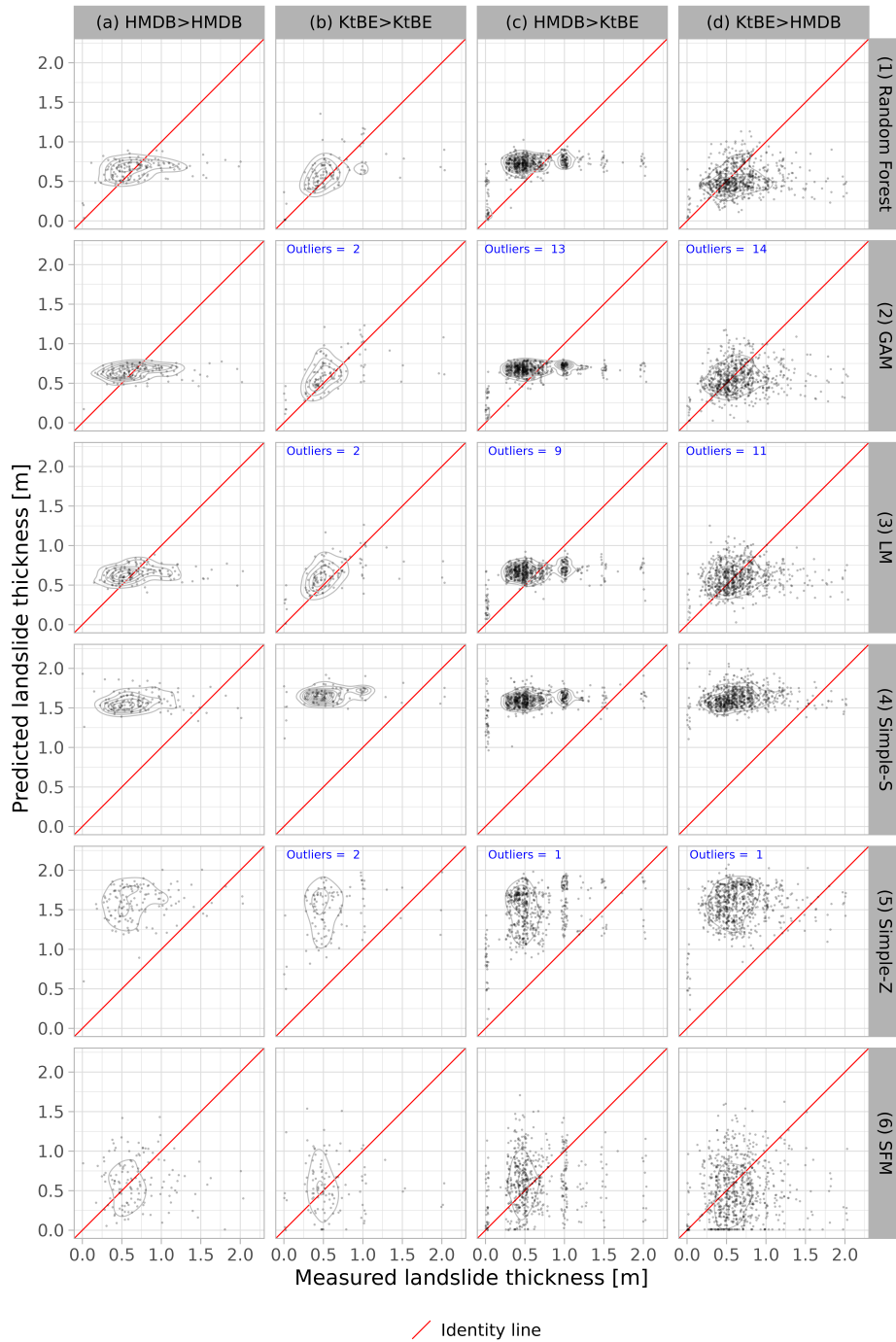
Figure 6. Scatter plots showing the actual-measured vs. the predicted landslide thickness differentiated by model type (rows) and dataset (columns): (a) model trained and tested with HMDB dataset, (b) model trained and tested with KtBE dataset, (c) model trained with HMDB and tested with KtBE dataset, and (d) model trained with KtBE and tested with HMDB dataset. The diagrams have 2D kernel density contours in the background as well as the identity line in red. Where present, the blue text denotes the number of outliers outside the display range of the plots.
