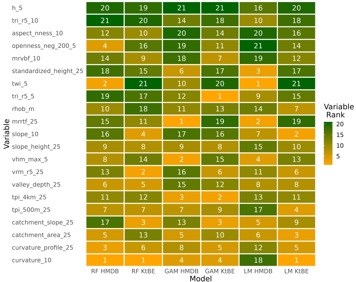
Figure B1. Heatmap showing the overall variable importance extracted from 10-fold cross-validation cross-validation for the RF and LM models and the importance of the best fit for the GAM model. The number in the cells and their colour correspond to the importance rank of the variable within the model, with 21 (green) being the most important and 1 (yellow) being the least important variable. The variables are sorted by the sum of the ranks of each row.
