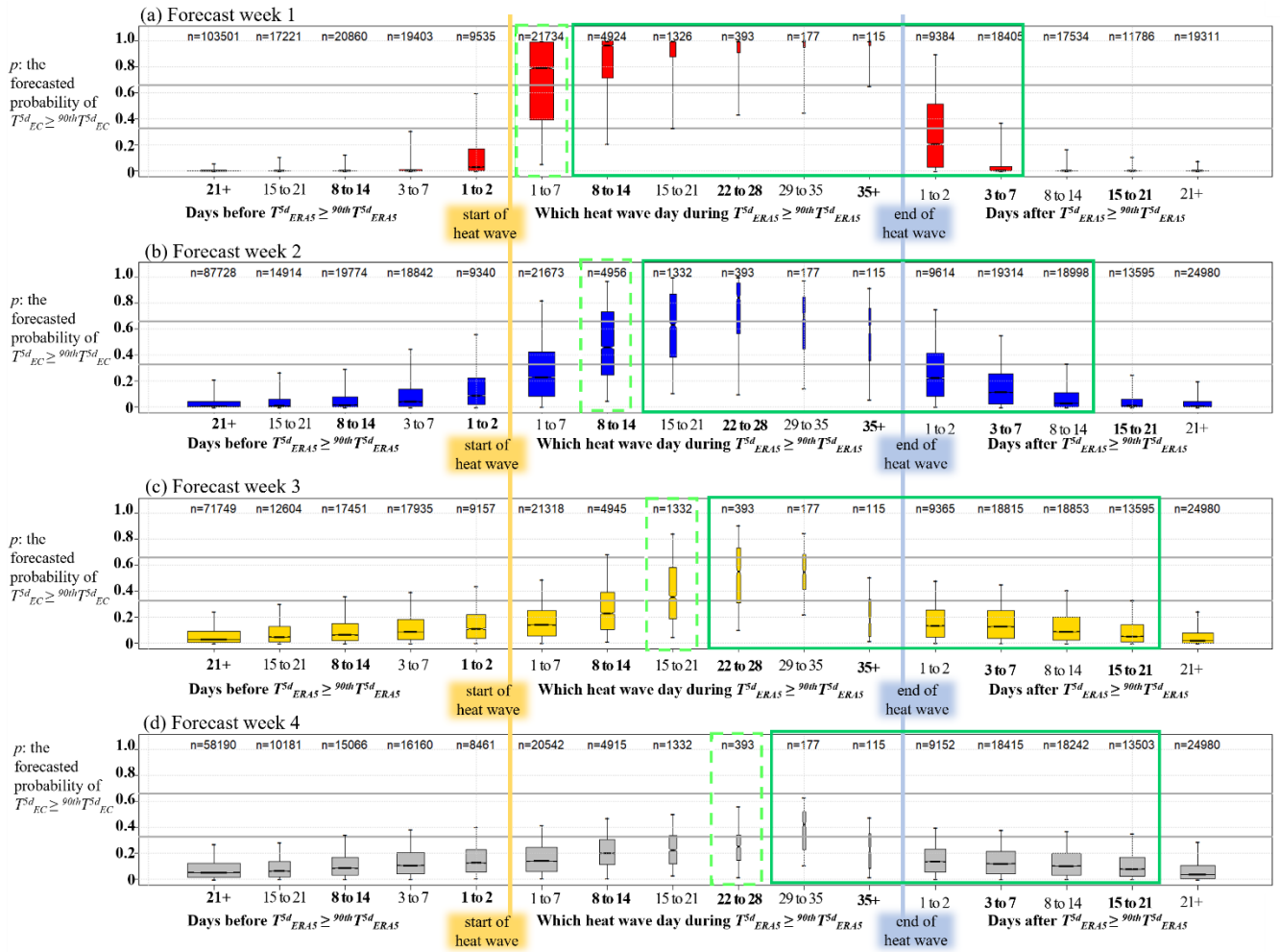
415 Figure 6: The forecasted probabilities of heat wave days shown for days that (in ERA5) were 21 to 1 days before the heat wave, the 1 st to 35 th heat wave day during the heat wave, and 1 to 21 days after the heat wave with lead times of a) one week, b) two weeks, c) 420 three weeks, and d) four weeks. Dashed green boxes indicate forecasts where, at the time of issuance, a heat wave in that grid point was about to begin within a week. Solid green boxes indicate forecasts where, at the time of issuance, a heat wave was already ongoing in that grid point. In the boxplots, a horizontal line box into two parts shows the median of the data; the ends of the box show the lower and upper quartiles; and the whiskers indicate the 5 th and 95 th percentiles of the data in each group. The boxplots include all forecast data across the European region at each land-grid point. The width of each box and the n written above each box indicate the number of observations in each group.
