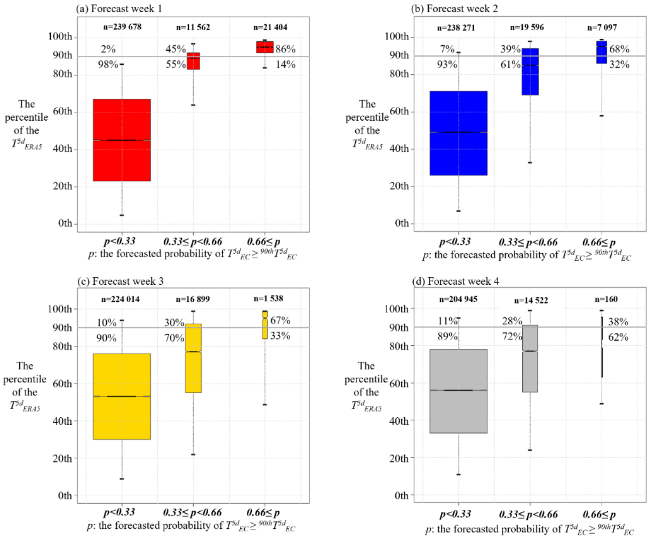
380 Figure 5: Boxplots of the ERA5 5-day moving average temperature over Europe in each grid point across different levels of p (the forecasted probability of a heat wave day) with lead times of a) one week, b) two weeks, c) three weeks, and d) four weeks. The horizontal line dividing each box into two parts shows the median of the data; the ends of the box show the lower and upper quartiles; and the whiskers indicate the 5 th and 95 th percentiles of the ERA5 data in each group. The width of each box and the n written above 385 each box indicate the number of observations in each group. The grey horizontal line indicates the 90 th percentile, i.e., the threshold of a heat wave day, and the percentiles above (and below) the grey line depict the fraction of observed heat wave days (and no-heat wave days) after the different levels of forecasted probability.
