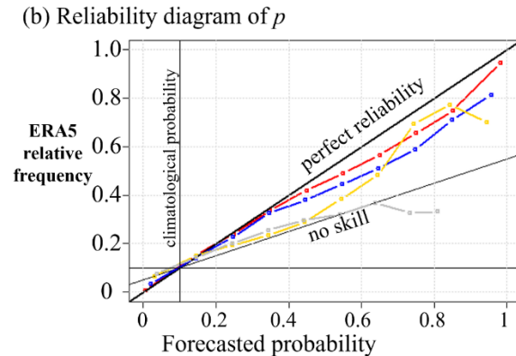
295 Figure 3: (a) sharpness diagram and (b) reliability diagram of the 1-4 weeks probabilistic heat wave days forecasts, p , over Europe (all land grid points) in summers 2000-2019.
