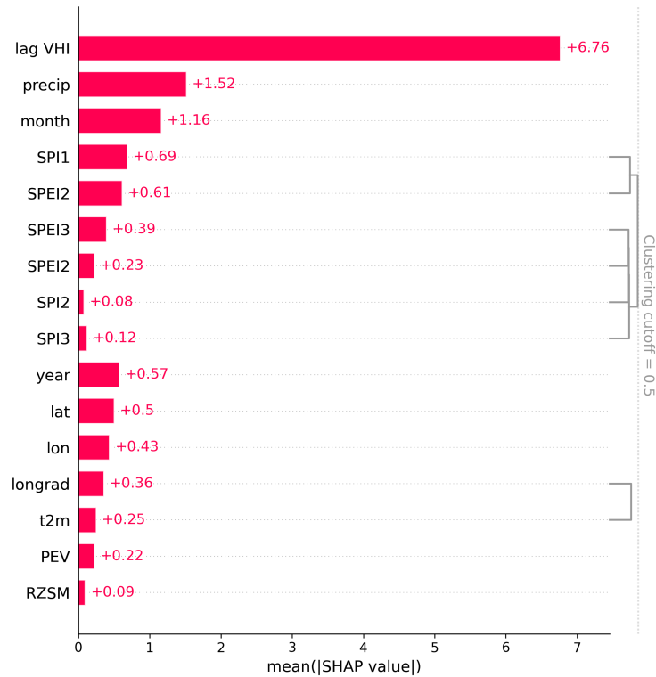
Figure 9. Shapley values obtained for each of the model input variables
