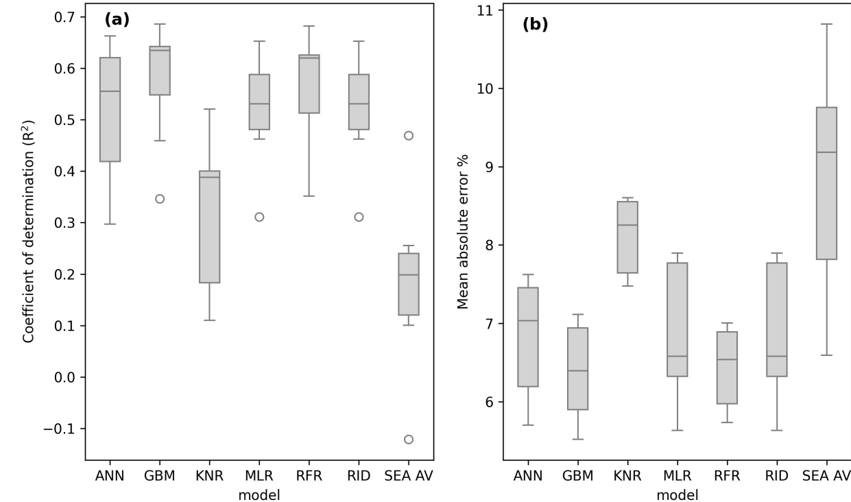
Figure 3. VHI forecasting model performance (a: coefficient of determination, b: mean absolute error) across a range of initially selected models. SEA AV refers to the monthly average model.
