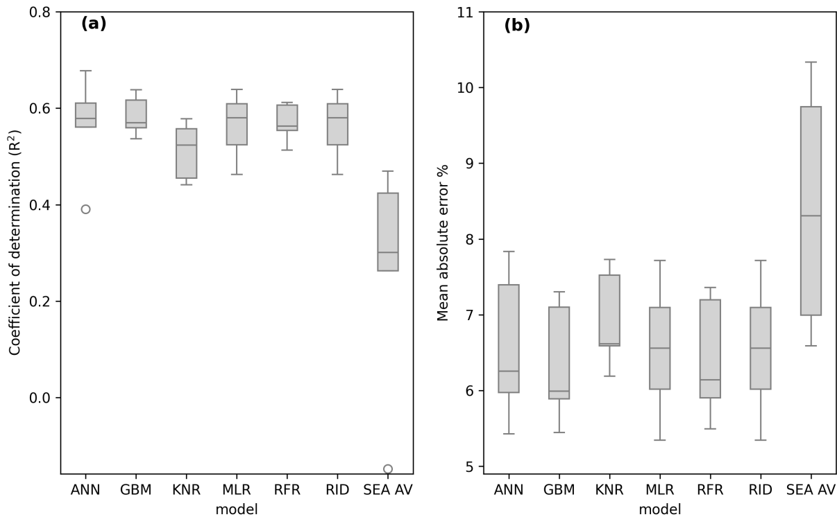
Figure A1. VHI forecasting model performance across the hold out evaluation data set for each of the initially selected models. Results shown are for optimized hyperparameters.
