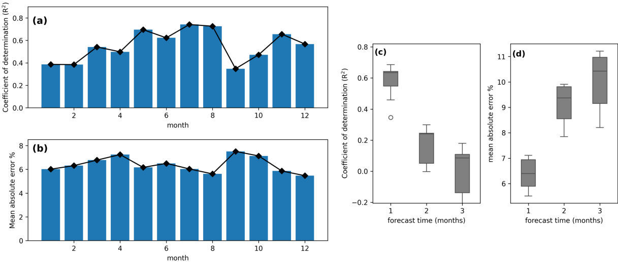
Figure B1. VHI forecasting model performance for the best model summarised as an average for each month, showing the R^2 score and mean absolute error per month (a) and (b). Secondly, model performance was compared for 2 and 3 month in advance forecasts (c) and (d).
