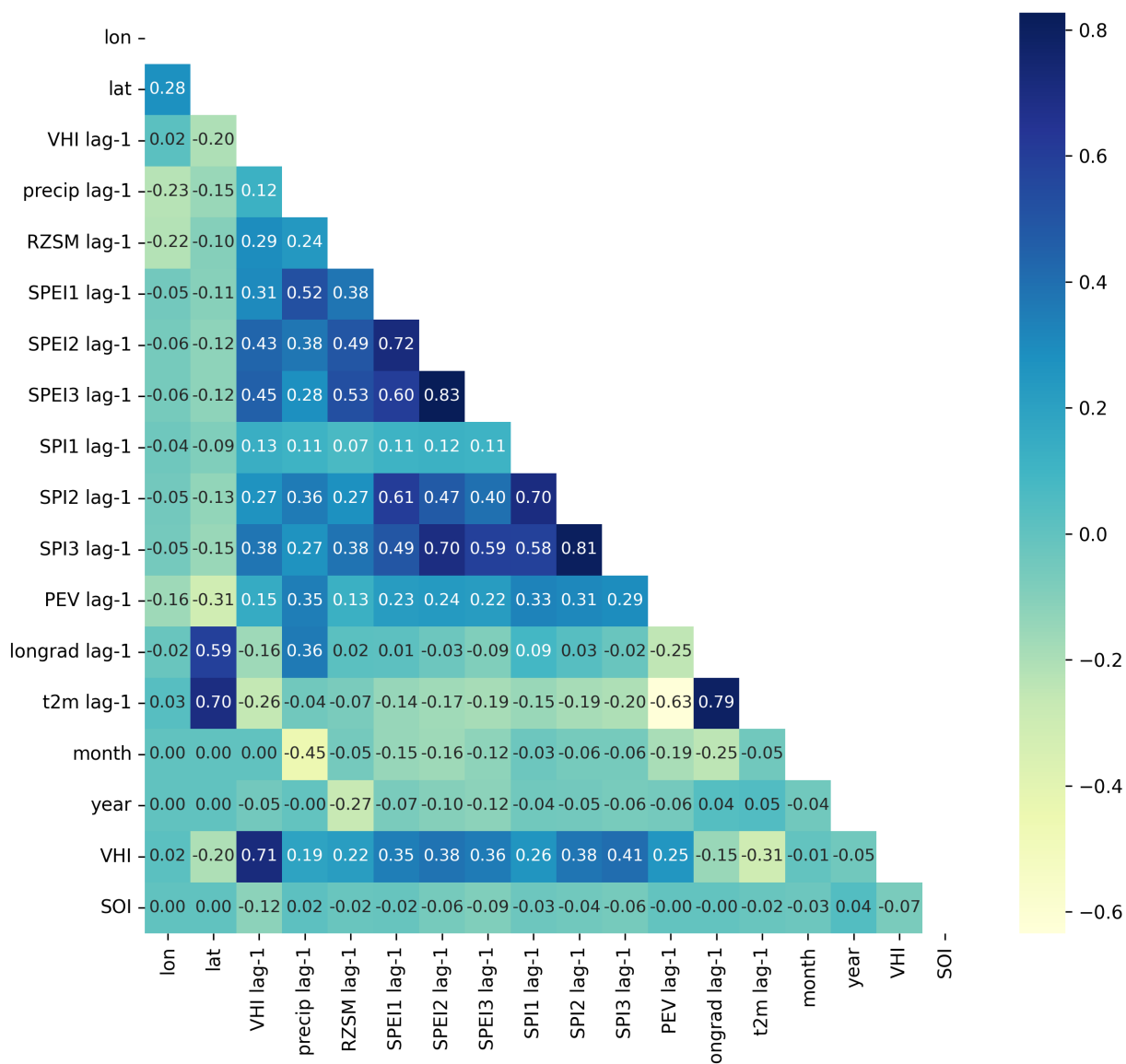
Figure C1. Spearman-rank correlation between proposed input variables and the target variable (VHI), lag-1 denotes a lag time of 1 month relative to time step of VHI.
