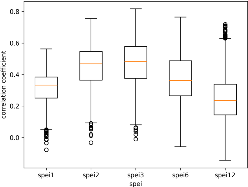
Figure E1. Correlation coefficient between SPEI indicators and observed VHI of the following month. Each correlation is calculated per grid cell (across 216 months) with box plots forming the spatial distribution of all correlations.
