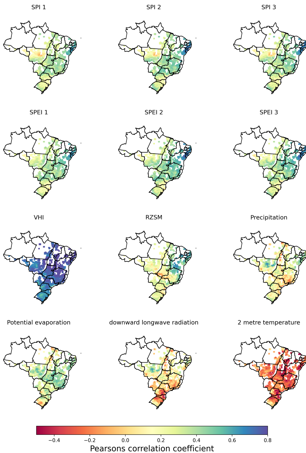
Figure 2. Correlation coefficient between the vegetation health index and predictor-input variables used in this study.
