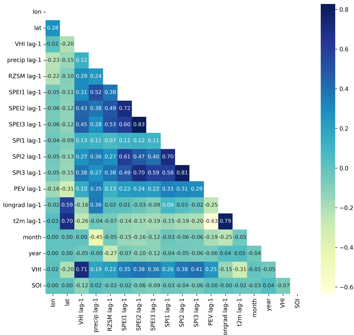
Figure C1. Spearman-rank correlation between proposed predictor input variables and the target variable (VHI), lag-1 denotes a lag time of 1 month relative to time step of VHI.
