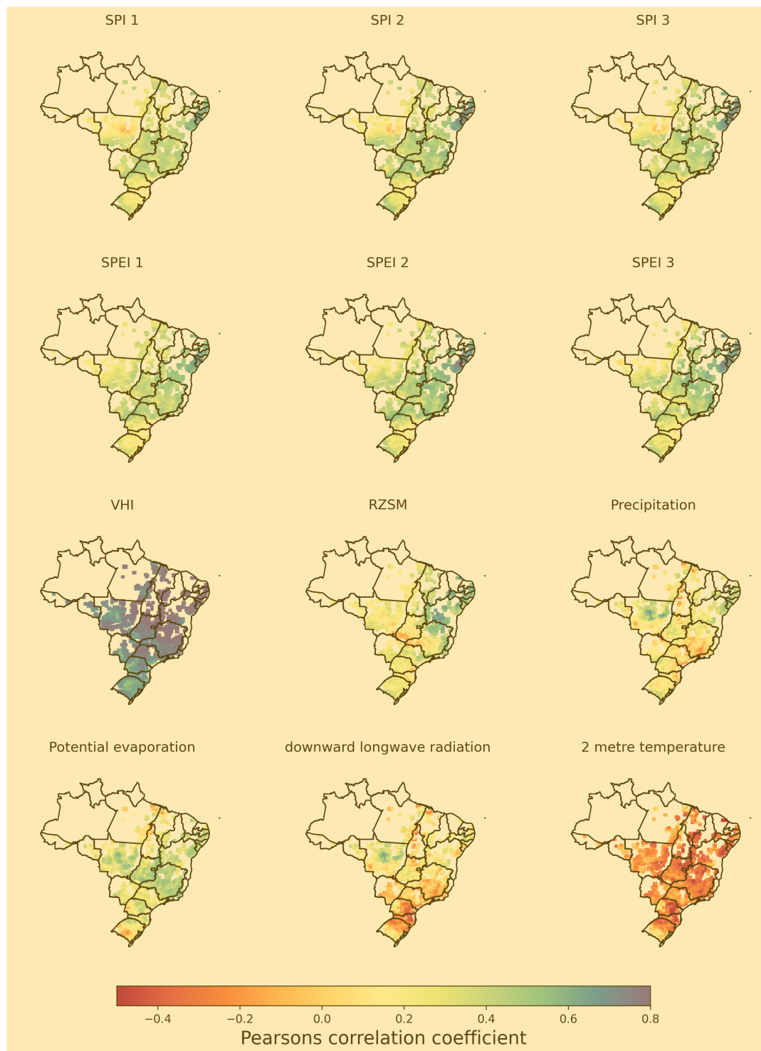
Figure 2. Correlation coefficient between the vegetation health index and predictor variables used in this study.
