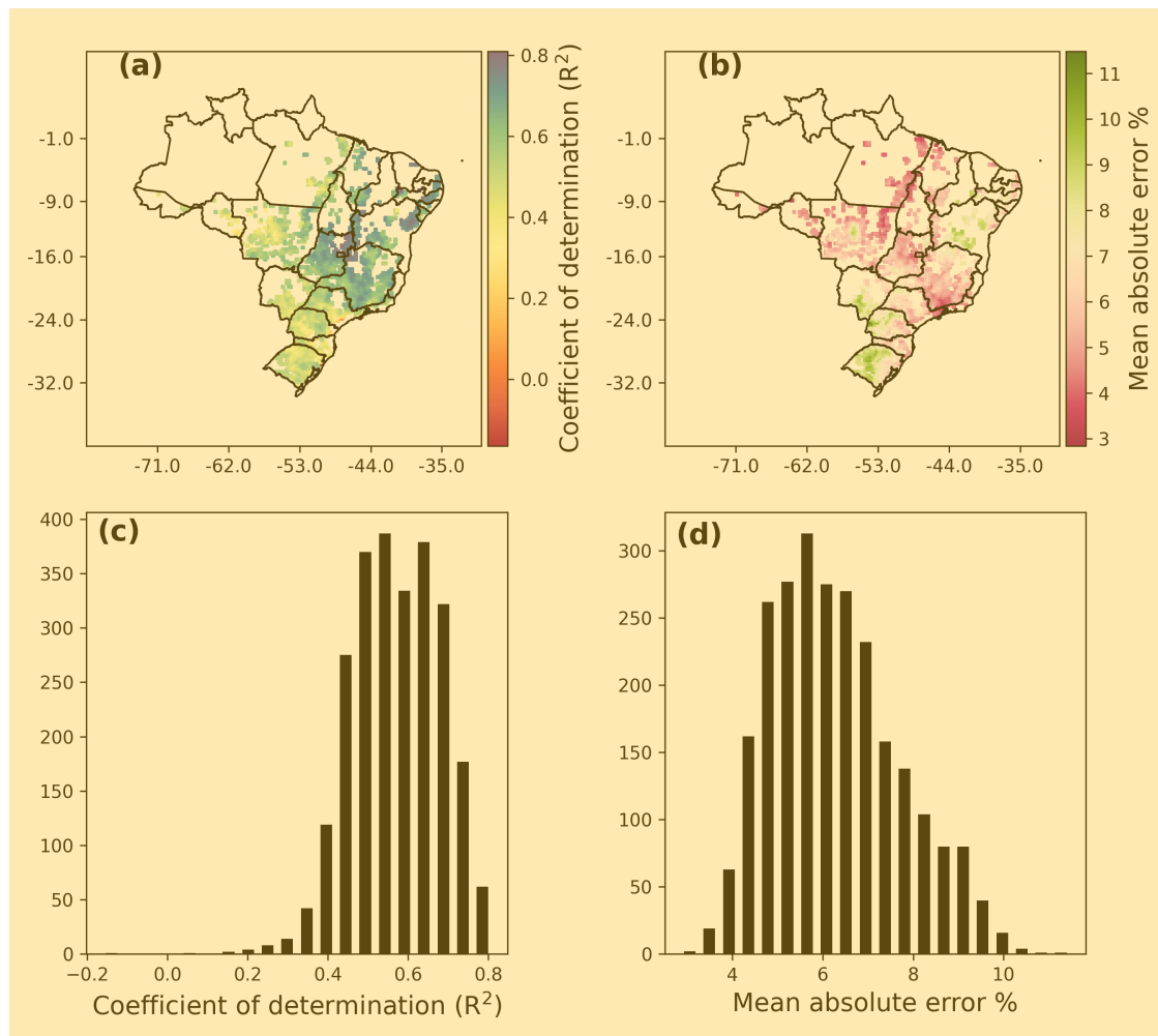
Figure 4. VHI forecasting model performance for the best model (GBM) across the spatial domain in Brazil, showing the R^2 score and mean absolute error for each grid cell location. Panels (a) and (b) show the spatial distribution of model performance for the two metrics, panels (c) and (d) show histogram of model performance metrics.
