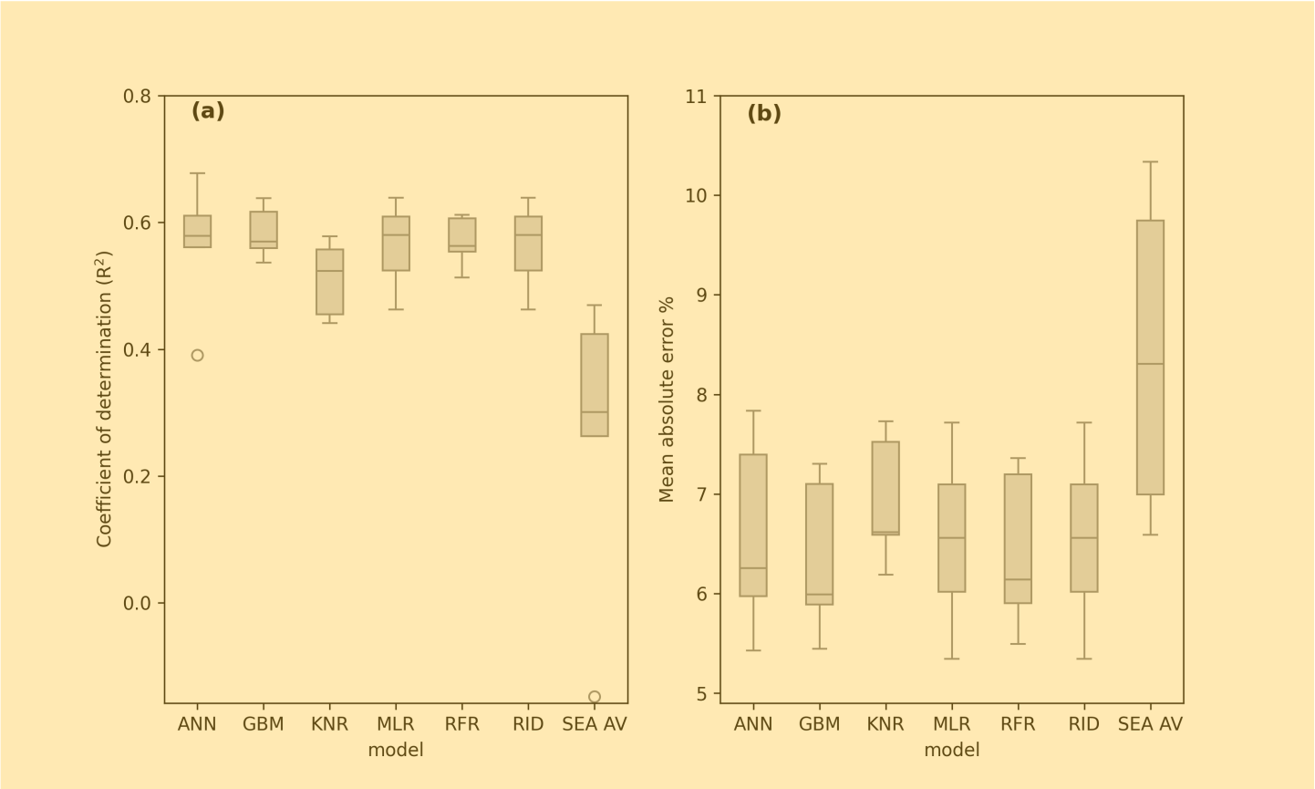
Figure 1a. VHI forecasting model performance across the hold out evaluation data set for each of the initially selected models. Results shown are for optimized hyperparameters.
