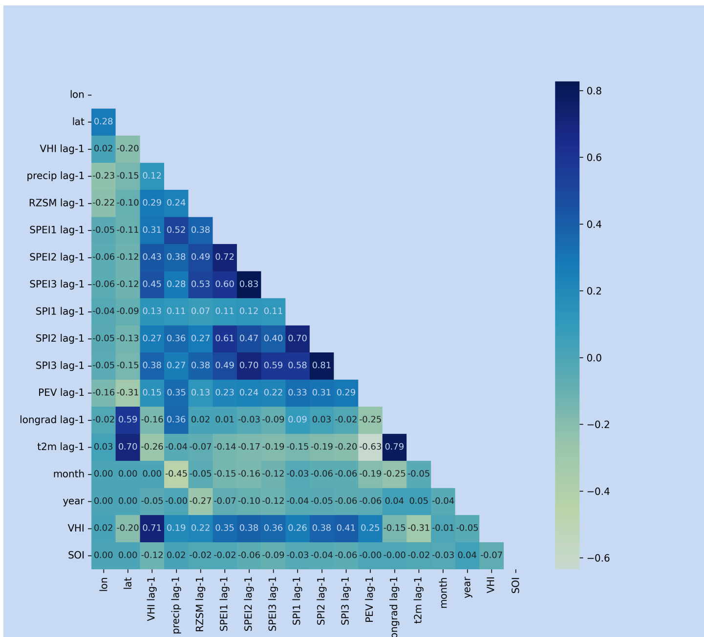
Figure 11. Spearman-rank correlation between proposed predictor variables and the target variable (VHI), lag-1 denotes a lag time of 1 month relative to time step of VHI.
