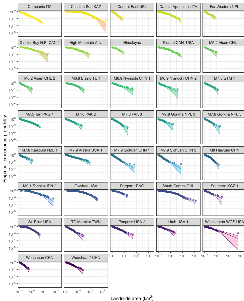
Figure 2. Size and frequency of large landslides from 37 inventories that reported at least 25 slope failures affecting \geq 0.1 km 2 each (Table 1). Circles are observed data ranked by their empirical exceedance probabilities, and lines are posterior medians of a fitted multi-level Generalised Pareto distribution (GPD) with shaded 95% highest density intervals (HDIs). Three-letter codes are ISO country identifiers; numbers refer to different catalogue versions of the same triggering event; catalogues related to earthquakes show estimated magnitude; * denotes inventories derived from deep learning.
