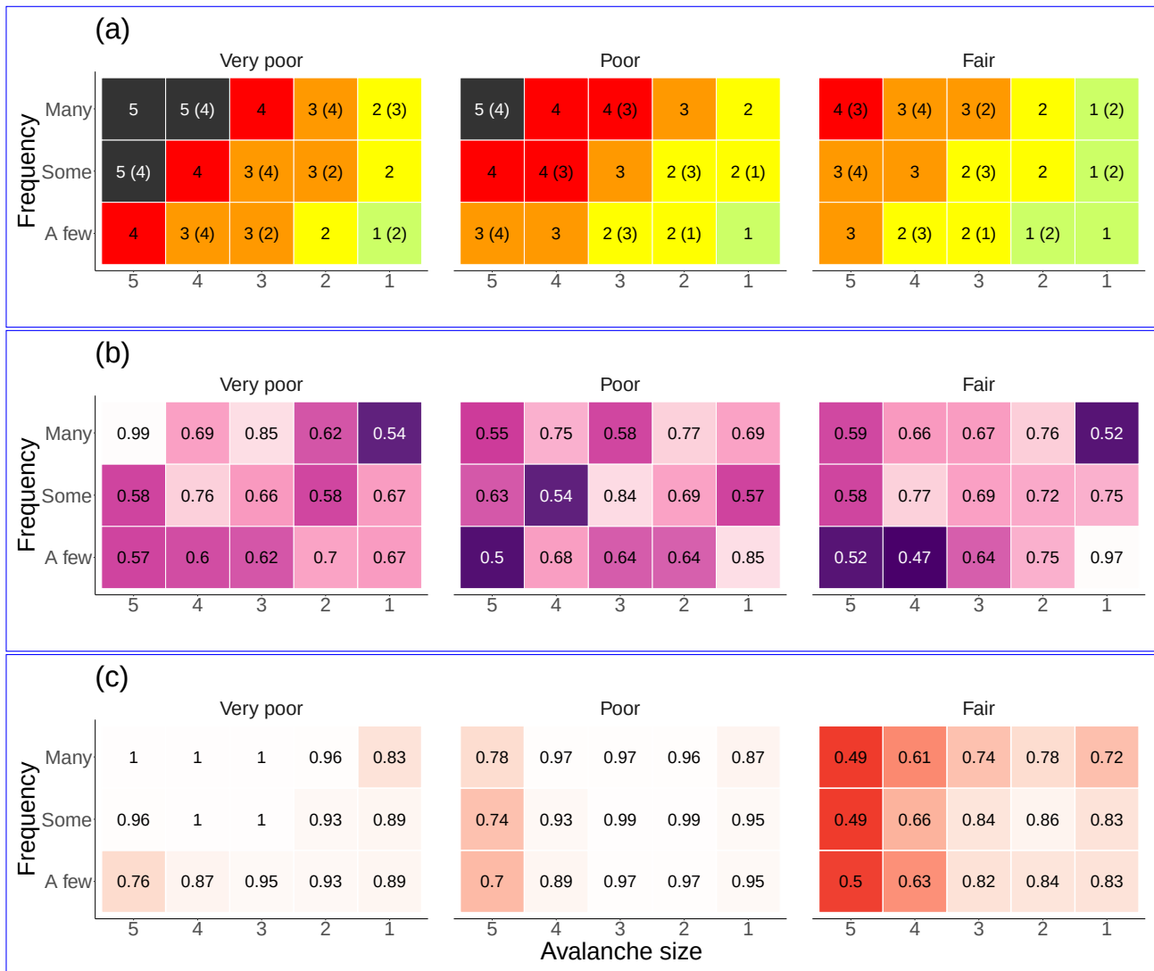
Figure 2. Survey responses for each combination of stability (panels), frequency (y-axis), and avalanche size (x-axis). The median danger level ( D^1 ) is displayed in a), while the proportion of responses agreeing with D^1 is shown in b). The proportion of responses providing a danger level estimate is depicted in c). Stronger color saturation indicates a larger proportion of responses agreeing with D^1 (b) or fewer responses (c) to emphasize considerable variability in opinions.
