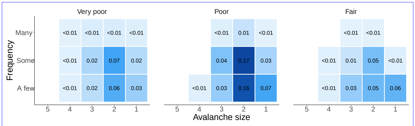
Figure 5. Use of individual matrix cells. The values represent the unweighted means of the respective proportions for all groups of warning services as in Table 6. Stronger color saturation indicates a larger proportion of responses.
