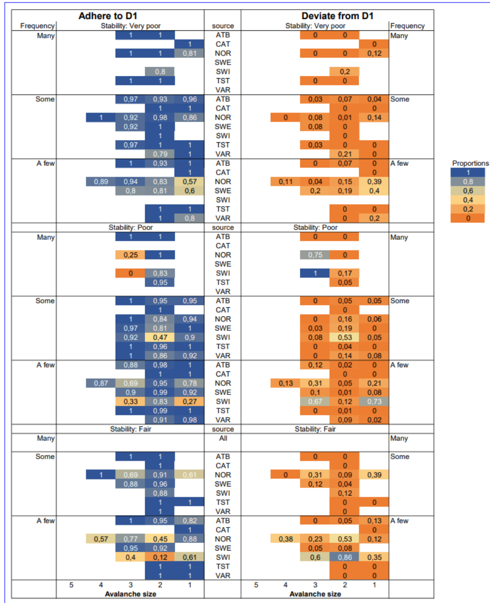
Figure 6. Proportion of cases that D = D^1 where forecasters adhere to D^1 or D \neq D^1 deviate from D^1 as were used by groups of warning services (center column). Combinations involving stability class fair and frequency class many were not recorded during 2022-2023. Abbreviations according to Table 6. Cells are displayed if the number of cases was \geq 5 .
