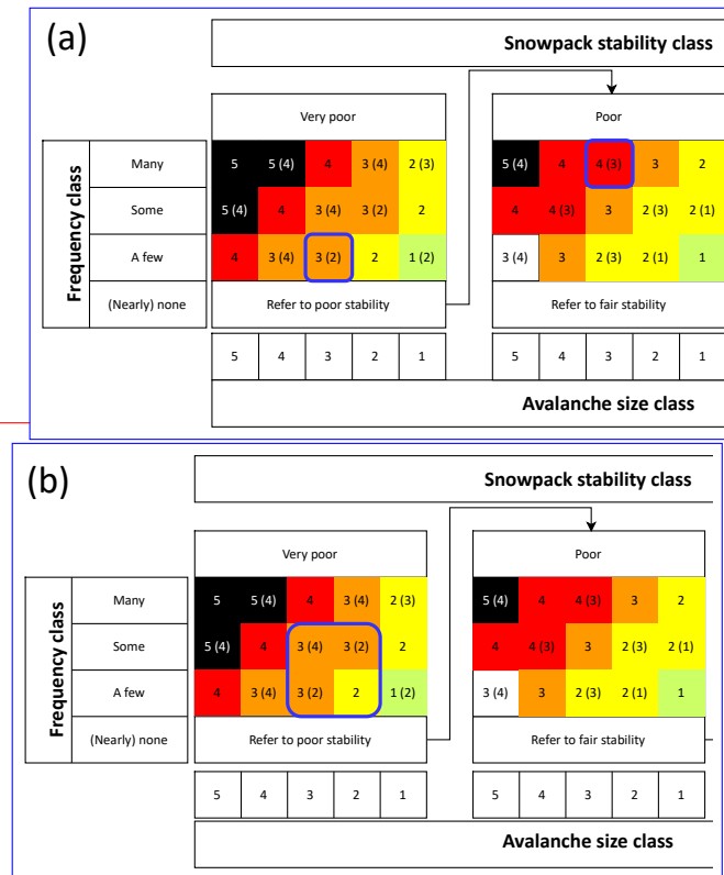
Figure 9. EAWS Matrix (extract) with several cells marked as relevant (blue border) to accommodate (a) a range of possible combinations or (b) uncertainty. In (a), two combinations of stability and frequency are considered ( very poor - a few , poor - some ), in (b) uncertainty relates to frequency ( a few or some ) and avalanche size ( size 2 or 3 ). For explanations refer to text.
