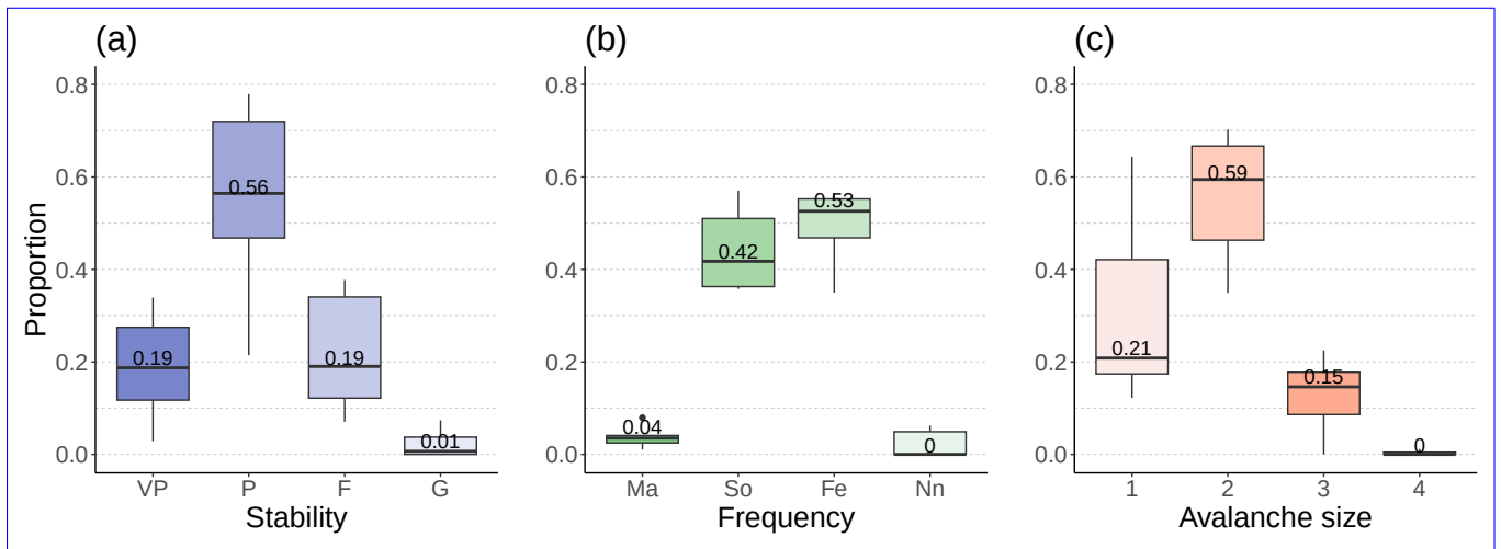
Figure 4. Use of classes during winter 2022-2023 describing (a) snowpack stability, (b) frequency, and (c) avalanche size. The boxplots represent the distribution of the class labels summarized for all warning services in Table 6. Abbreviations for i) stability are VP-very poor, P-poor, F-fair, G-good, ii) frequency are Ma-many, So-some, Fe-a few, Nn-none or nearly none, iii) and the avalanche size classes 1-5 (size-5 never used).
