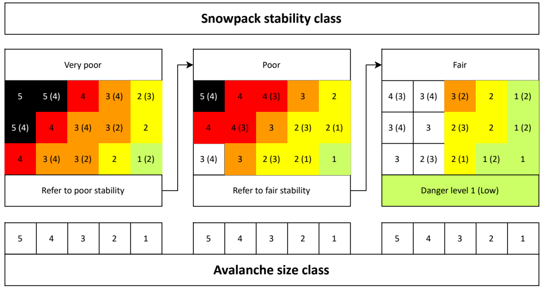
Figure 3. EAWS Matrix, as accepted by the EAWS General Assembly in 2022 (taken from EAWS, 2022b), is organized into three distinct panels, each corresponding to one of the three lowest snowpack stability classes. Within each panel, the frequency (on the y-axis) is plotted against avalanche size (on the x-axis). To navigate through the matrix, arrows interlinking the panels indicate to transition to the next stability class, specifically when the frequency is evaluated as none or nearly none . According to the workflow (Müller et al., 2023), forecasters first assess the frequency of the most vulnerable locations, progressing progress from left to right across the panels, assessing the frequency of the lowest stability class first . Upon identifying a relevant stability-frequency combination, forecasters then evaluate the corresponding avalanche size, culminating in a leading to the recommended danger level(s).
