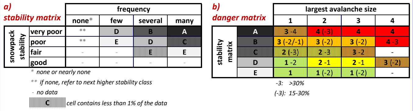
Figure A4. Data-driven look-up table for avalanche danger assessment (figure and caption taken from Techel et al., 2020a). The (a) stability matrix combines the frequency class of the most unfavorable snowpack stability class (columns) and the snowpack stability class (rows) to obtain a letter describing specific stability situations, the (b) danger matrix combines the largest avalanche size (columns) and the specific stability situations (letter) obtained in the stability matrix (rows) to assess the danger level. In (b): The most frequent danger level is shown in bold. If the second most frequent danger level was present more than 30% of the cases, the value is shown with no brackets, if present between 15 and 30% it is placed in brackets. In (a) and (b): Cells containing less than 1% of the data are marked.
