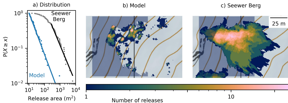
Figure 9. a) Release area distribution of recorded glide snow avalanches on the Seewer Berg slope (black, \alpha_{\text{Seewer Berg}} = 2.1 \pm 0.2 , x_{\text{min}} = 273 \text{ m}^2 ) and the simulation based on the DEM (blue, \alpha = 2.2 \pm 0.2 , x_{\text{min}} = 10 \text{ m}^2 ) with the corresponding power law fit (line plot). b) The heatmap of modelled avalanche release with the masked out area due to the high vegetation roughness (blue shaded). c) The heatmap of observed glide-snow avalanche releases (2008/09 to 2022/23) with the masked out area (blue shaded). Map: Federal Office of Topography
