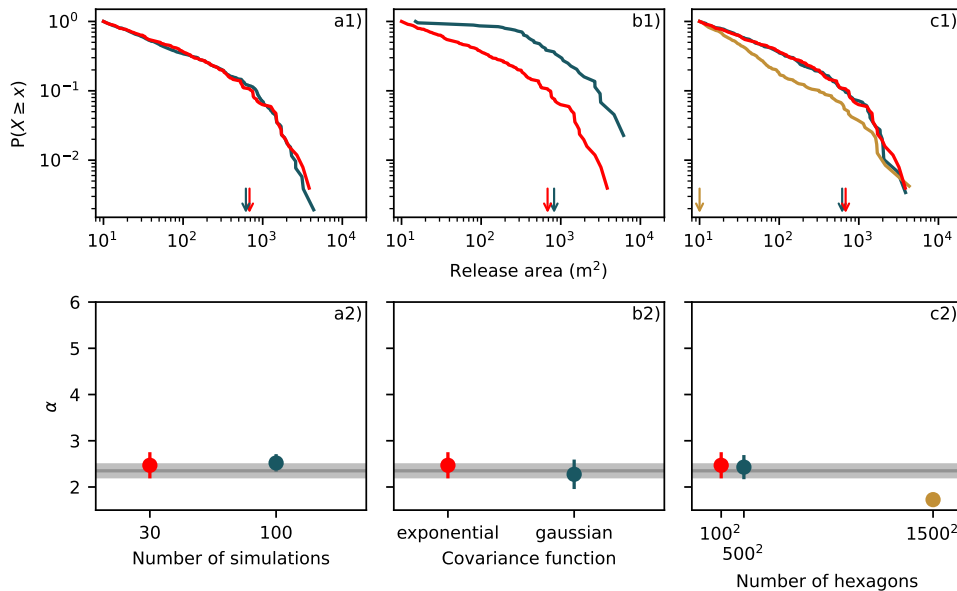
Figure A1. _1) Effect of the boundary conditions on the release area distribution. For the 1500 x 1500 system size only 15 simulations were performed due to long simulation duration. The color indicates the parameter value as given in the graph below. The arrows indicate x_{\min} . _2) Comparison between the modelled power law exponents \alpha and the Dorfberg power law exponent and its fit uncertainty (gray).
