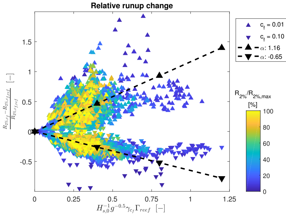
Figure A2. Variation in relative wave runup as a function of the right-hand term of Equation A5. Linear proportionality constants \alpha_r found for reef profiles with lower ( c_f = 0.01 ; \blacktriangle ) and higher ( c_f = 0.10 ; \blacktriangledown ) reef roughness are shown as dashed lines. Computed relative runup values are coloured by the computed wave runup relative to the maximum runup in the calibration dataset.
