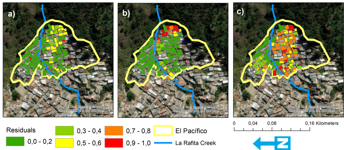
Figure 11. Residuals computed from the difference between physical vulnerability at the worst case scenario minus the median scenario for Flash flood (a), rockfall (b) and landslide (c)
