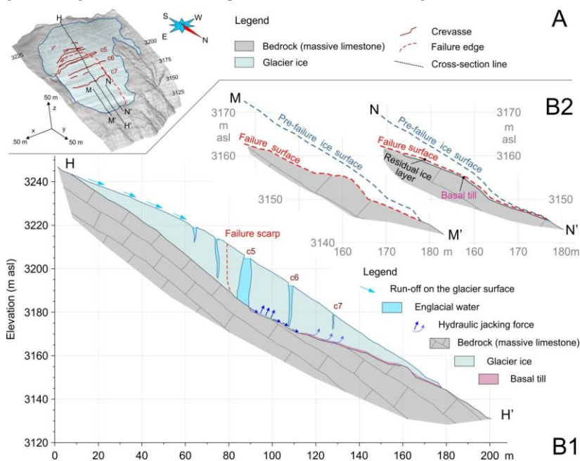
Figure 16: (A) Pre-failure model of the glacieret with evidenced cross-sections HH', MM', and NN'. (B1) Pre-failure cross section HH' with indicated: failure surface; bedrock morphology; hydraulic jacking forces, etc. (B2) Post-failure models of the lower portion of the failure surface along cross sections MM' and NN'. The failure surface developed along an ice foliation in NN' while the detachment reached the underlying bedrock in MM'.
