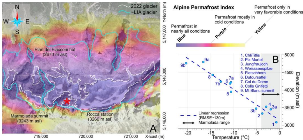
355 Figure 8: (A) Modelled permafrost occurrence in the Marmolada massif (after Boeckli et al., 2012). The detachment zone is marked with a red asterisk. A strong contrast exists between the sun-exposed, ice-free south wall with its warm, probably non-frozen rocks, and the cold north-slope oriented away from the sun and with widespread permafrost. The glacier boundary in July 2022 is outlined with a white line while the line in cyan colour outlines the boundary of the LIA glacier. (B) Ice temperature measured at different sites in the Alps (redrawn from Haeblerli et al., 2004a and updated including the Weissseespitze from Fischer
