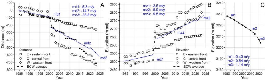
Figure 3: FrontMeasurements of front migration and surface ablation-measurementslowering for the Marmolada glacierGlacier. A reference point was available for each of the different glacier sections (see also Fig. SM 4). (A) Inclined distance taken from the glacier front over the period 1985-2023. (B) Vertical distance taken from the glacier front over the period 1985-2023. (C) Progressive lowering of the glacier surface in the period 1980-2022 computed right at the point of collapse.
