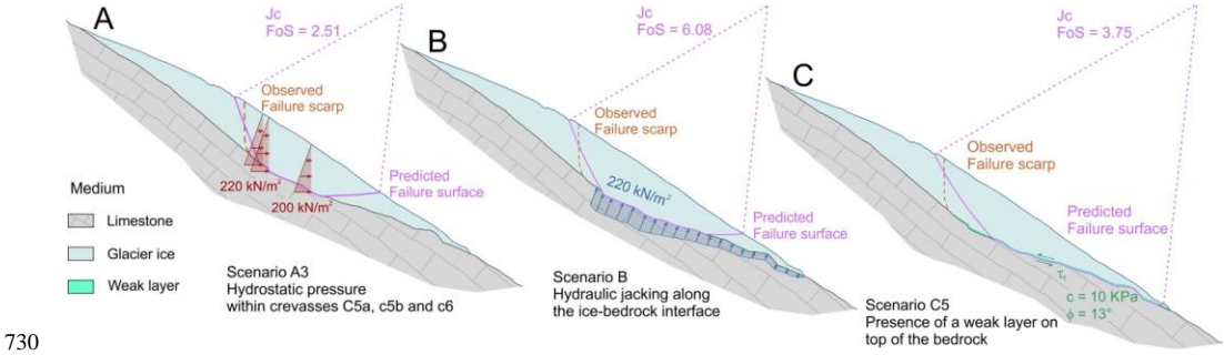
Figure 17: Numerical simulations: base scenarios. (A) Scenario A3 - hydrostatic pressure acting on crevasses 5a, 5b and 6; (B) Scenario B - hydraulic jacking pressure acting along the ice-bedrock interface; (C) Scenario C - reduction of the basal friction caused by a weak layer on top of the bedrock in the worst case ( c=10 \text{ kPa} ; \phi=13^{\circ} ). See text and Table 1a for details.
