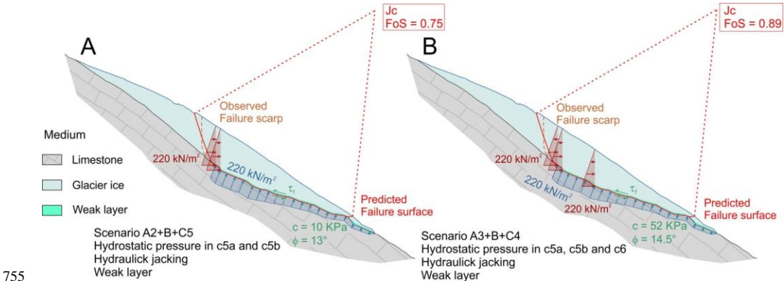
Figure 18: Numerical simulations: combined scenarios. (A) The instability condition, with relative FoS less than 1, is reached in the scenario A2 (hydrostatic pressure in two crevasses) + B (hydraulic jacking pressure) + C5 (worst c , \phi pair in the weak layer); (B) The instability condition, with relative FoS less than 1, is reached in the scenario A3 (hydrostatic pressure in all crevasses) + B (hydraulic jacking pressure) + C4 (second worst c , \phi pair in the weak layer). See text and Table 1b for details.
