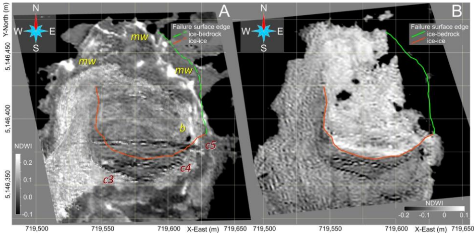
390 Figure 10: NDWI (Normalized Difference Water Index) map obtained via processing of multispectral satellite images (Pléiades Neo, AIRBUS Defence & Space) of the glacieret before and after the failure. (A) Date of acquisition: June 20, 2022; b – longitudinal bédrière; mw - meltwater. (B) Date of acquisition: June 20, 2022. See text for details.
