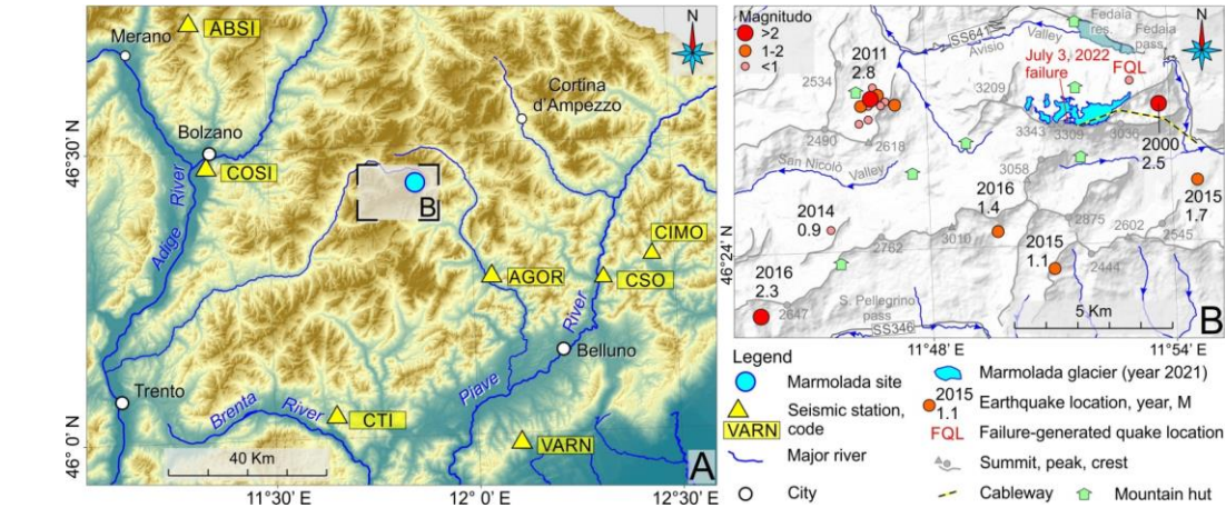
Figure 14: Seismological settings. (A) Topographic map showing the location of the seismic stations around the Marmolada glacier. (B) Historical earthquakes occurred in the vicinity of the failure site; the FQL letter designates where the earthquake that was caused by failure was recorded by the nearby seismic stations; an earthquake with magnitude 2.5 was detected in the year 2000 just east of the glacier. On the day of the collapse only three earthquakes (Table 2) occurred in northern Italy and they were located more than 50 km from the glacier.
