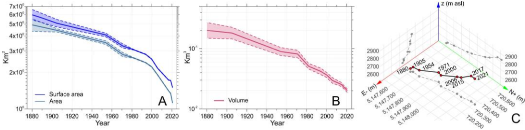
Figure 4: Over a century (1880–2021) of retreat of the Marmolada glacier as for Glacier retreat in terms of area, surface, area (two-dimensional measure of the slope's terrain surface, accounting for all inclinations and undulations), volume, and front migration , obtained via through GIS/CADD analysis and processing. (A) Area and surface area reduction, the interval of confidence is represented by dashed lines. (B) Volume reduction, the interval of confidence is represented by dashed lines. (C) Tri-dimensional spatial migration of the centroid of the glacier front (the centroid was calculated as the arithmetic mean of the xyz coordinates of the nodes in the polyline representing the glacial front in different years, see SM in Bondesan and Francese, 2023 for details).
