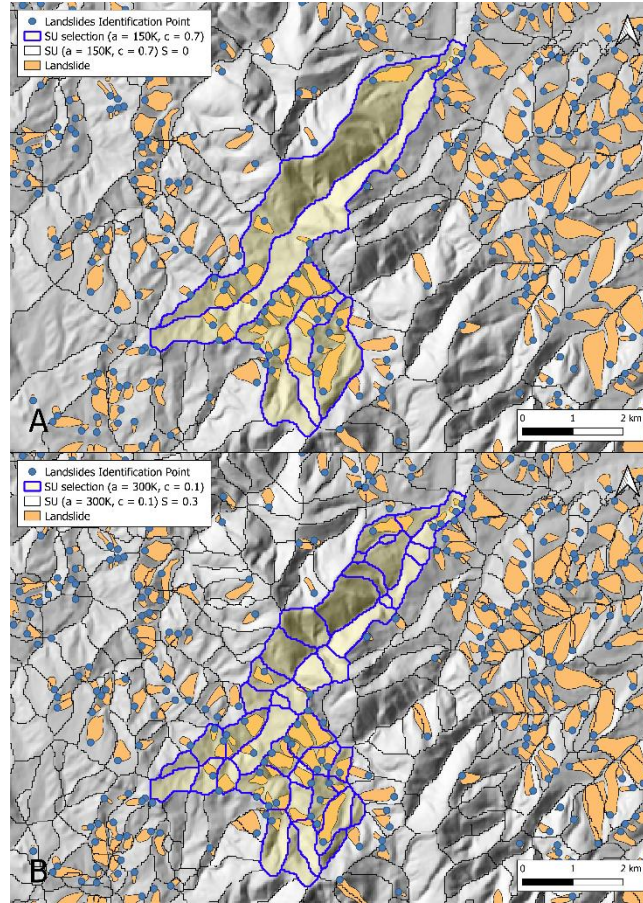
Figure 13: SUs partitions of a sub-portion of the Marche study area (AOIa) compared to landslides distribution from the PAL. A) the SU partition ( a: 150 \times 10^3 \text{ m}^2 and c: 0.7 ) with lowest value of S , B) the SU partition ( a: 300 \times 10^3 \text{ m}^2 and c: 0.1 ) with highest value of S .
