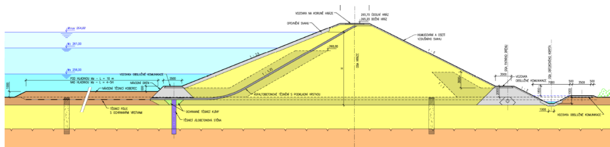
195 Figure 4: Cross section of the planned Skalička Dam
