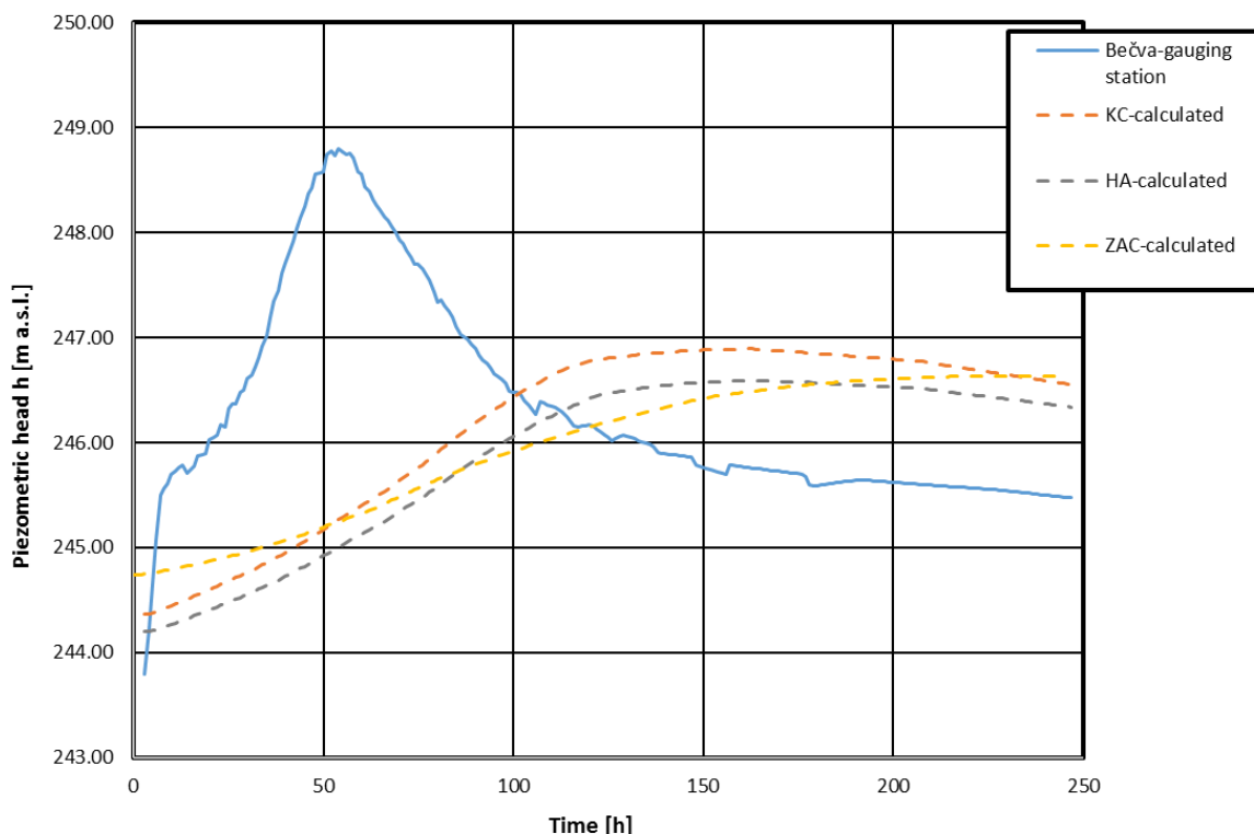
435 Figure 12: Water levels in monitored objects for scenario II.B.
