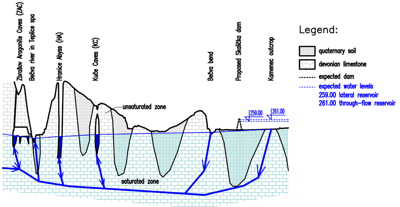
250 Figure 4: The sketch with conceptual model of a karst system
