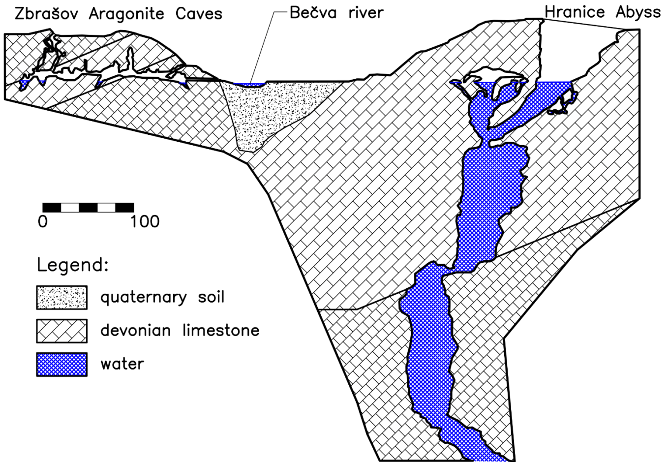
185 Figure 3: The detailed interpretation of ZAC and HA in the Teplice spa, cross section from ZAC to HA in Fig. 2 (Sracek et al., 2019), vertical and horizontal scales are the same.
