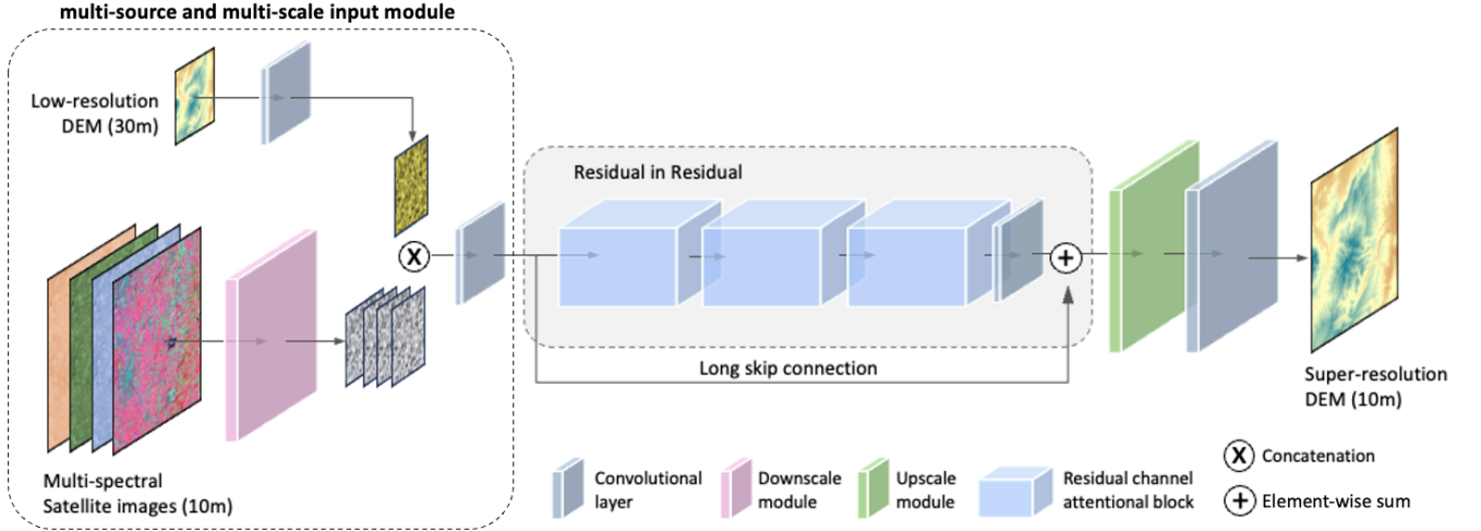
Fig. 1 The structure of the proposed DEM super-resolution model, MS-RCAN. Low-resolution DEM data and four-band multispectral satellite images are fused using a tailored multi-source and multi-scale input module to facilitate the reconstruction of high-resolution DEM data.
