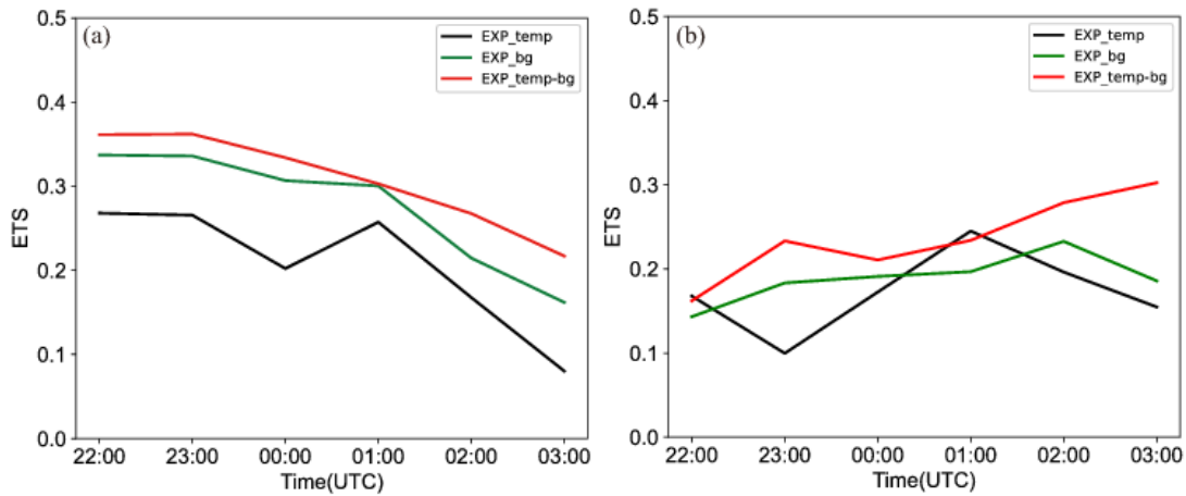
Fig. 15. ETS of three DA experiments for the thresholds of (a)2.5mm/h, (b)10mm/h, (c)1mm/h, (d)3mm/h and (e)5mm/h.
