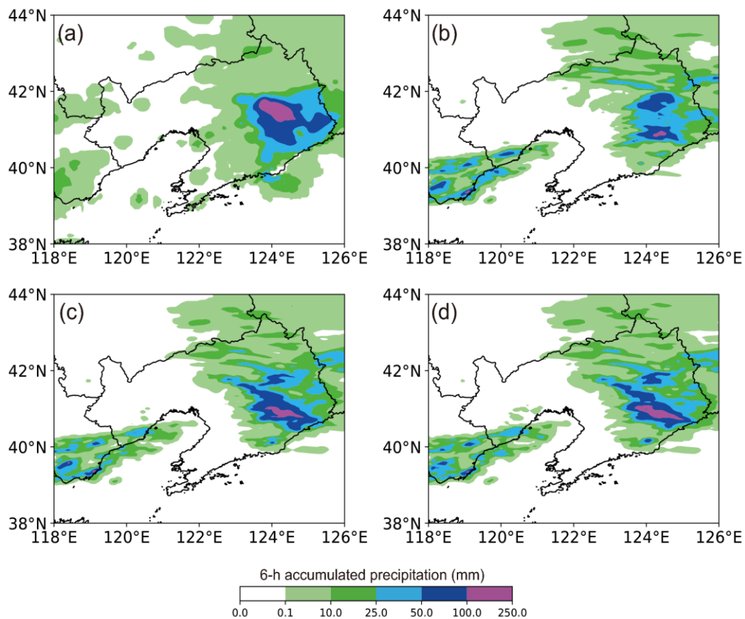
Fig. 14. 6-h accumulated precipitation initialized at 2100 UTC 06 August 2018. (a) the observation, (b) EXP_temp, (c) EXP_bg, and (d) EXP_temp-bg.
