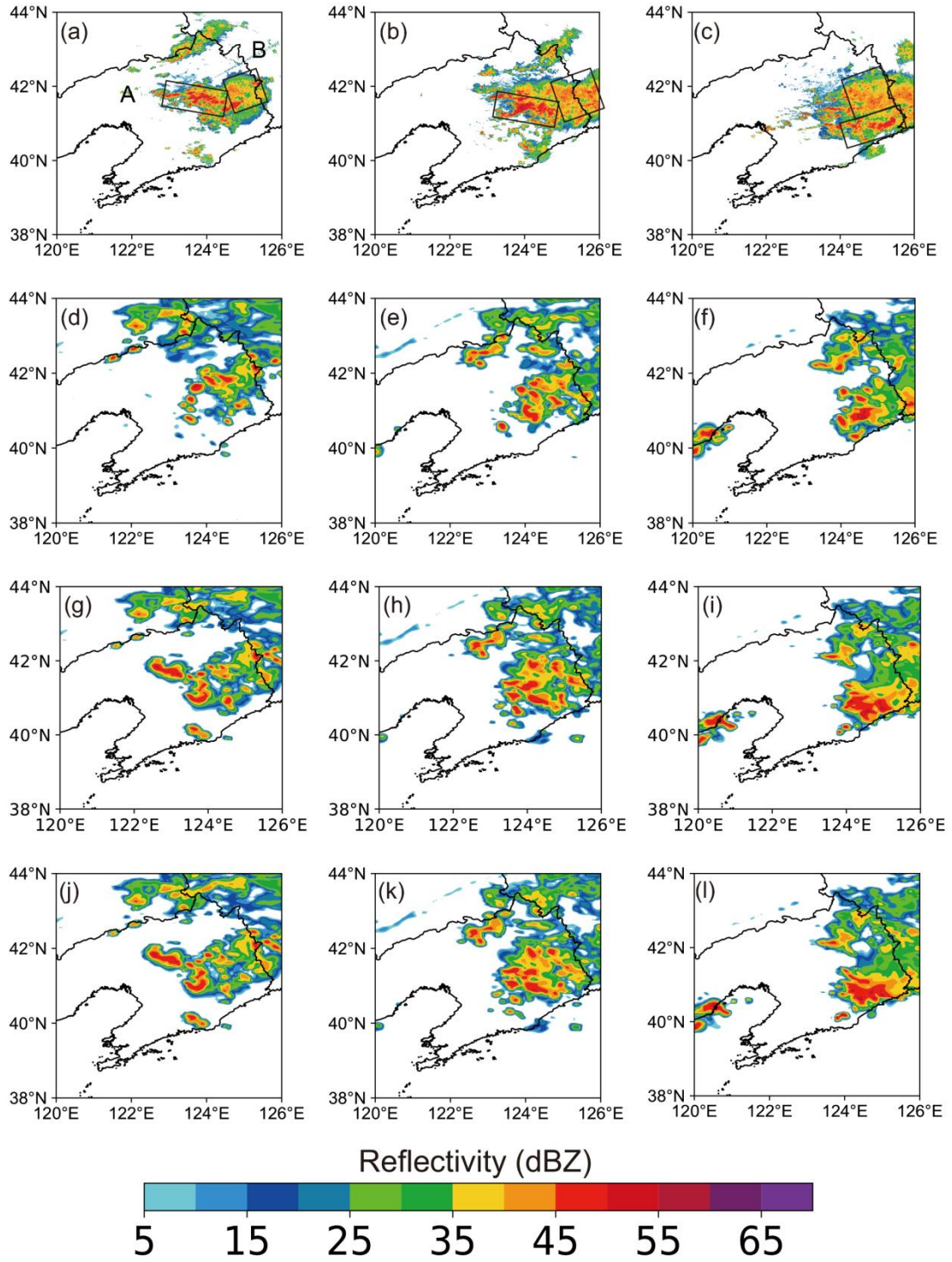
Fig. 13. The composite reflectivity (shaded; units: dBZ) predicted by (d)-(f) EXP_temp (g)-(i) EXP_bg and (j)-(l) EXP_temp-bg, as compared to (a)-(c) the observed composite reflectivity. The corresponding times from left to right are 2200 UTC 06 August (left), 0000 UTC 07 August (middle) and at 0200 UTC 07 August (right), respectively. The labels A and B present the convection locations.
