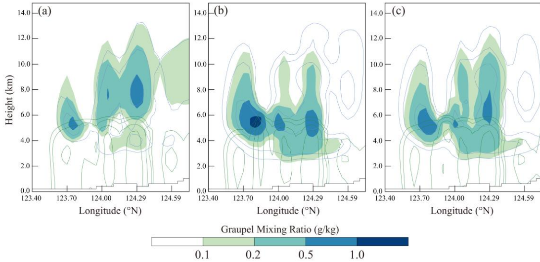
352 Fig. 11. The vertical cross sections of rainwater mixing ratio (green contours), snow mixing ratio (blue contours), 353 graupel mixing ratio (shading) at 2100 UTC for the experiments (a) EXP_temp, (b) EXP_bg, (c) EXP_temp-bg. The 354 position of the cross sections is located at the line ab of the Fig. 10a.
