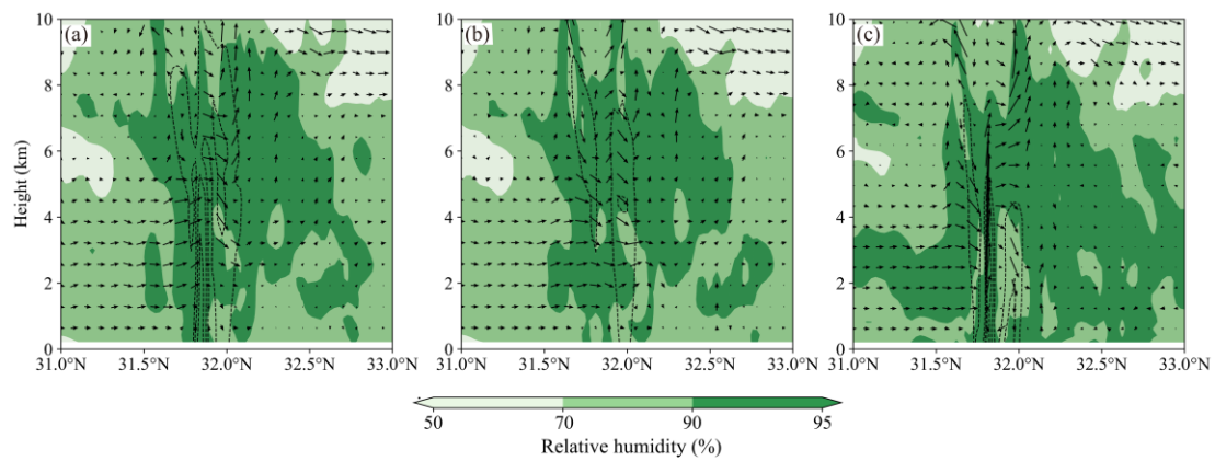
Fig. 6. The cross sections of relative humidity (shading; units: %), radar reflectivity (black contours starting at 40 dBZ; units: dBZ), and wind vectors for (a) EXP_temp, (b) EXP_bg and (c) EXP_temp-bg along the line a1-a2. These are 1-hour forecasts initialized at 1501 UTC.
