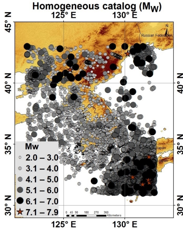
Figure 6: Homogeneous earthquake catalog for South Korea and neighboring regions covering the period from 1905 to 2023.
