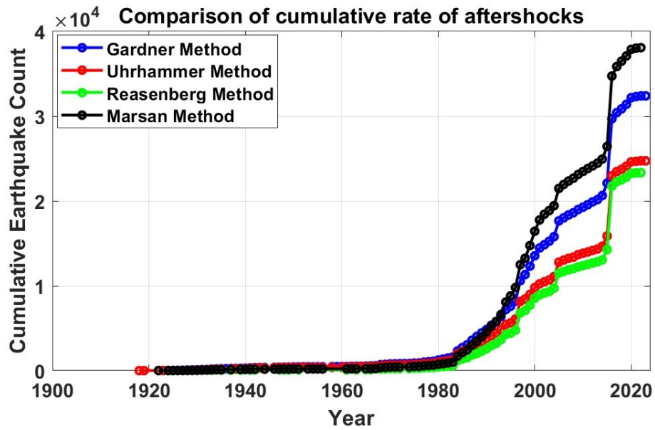
Figure 18: Time-series plot of cumulative seismicity of aftershocks for each algorithm.
