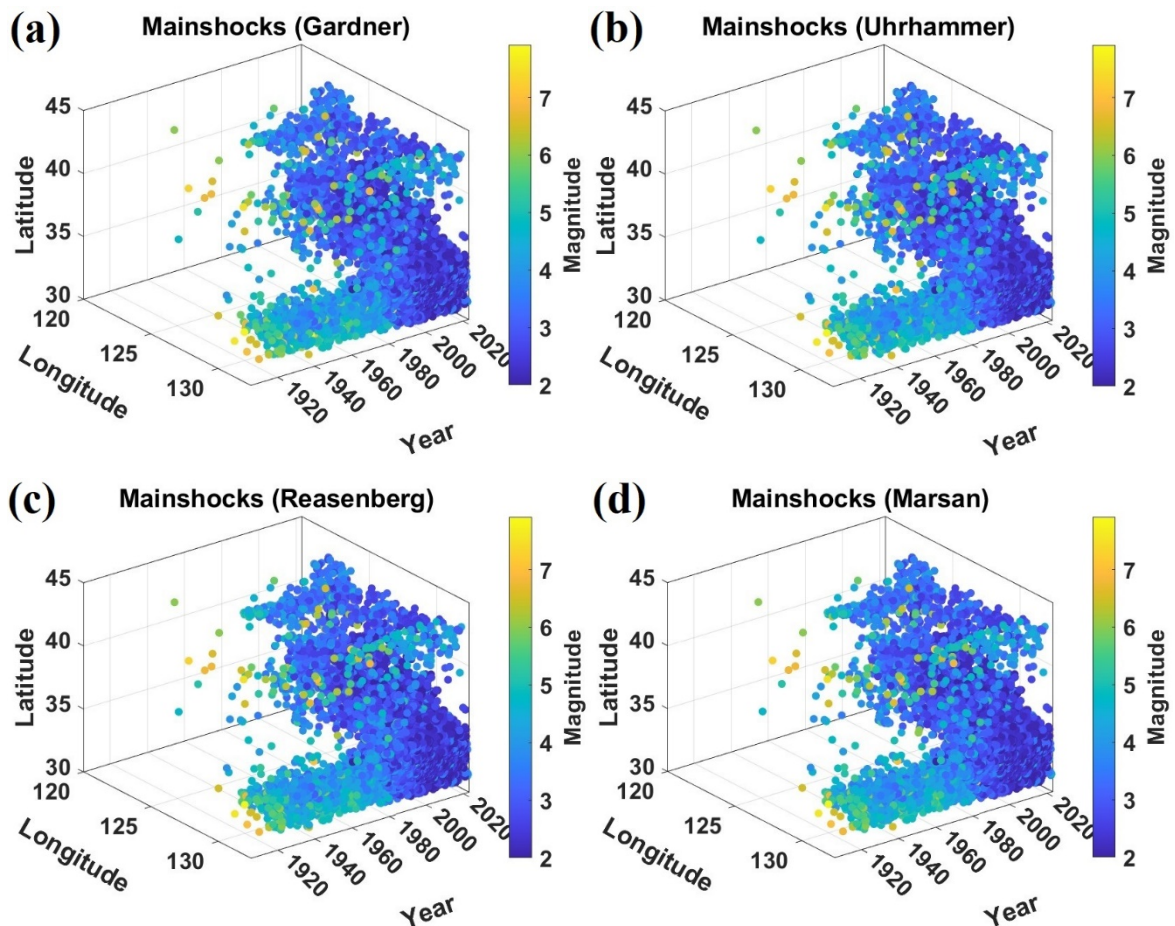
Figure 19: Time of Occurrence vs. Latitude-Longitude Comparison plot of Mainshock earthquakes using (a) Gardner method (b) Uhrhammer method (c) Reasenberg approach (d) Marsan method.
