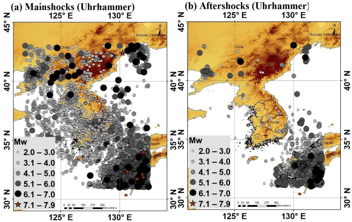
Figure 8: Declustered seismicity distribution map using the Uhrhammer method depicting (a) for mainshocks and (b) for aftershocks, covering the period from 1905 to 2023.
