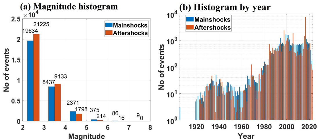
Figure 9: Histogram plots for (a) number of events by magnitude and (b) temporal distribution of events for mainshocks and aftershocks using the Gardner and Knopoff method.
