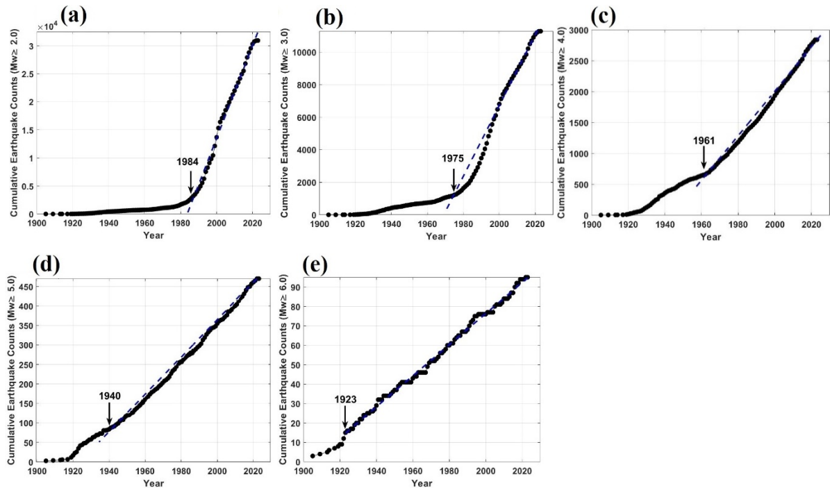
Figure 15: Completeness analysis for the Gardner and Knopoff declustered catalog using the CUVI method for each magnitude range: (a) M_W \geq 2.0 (b) M_W \geq 3.0 (c) M_W \geq 4.0 (d) M_W \geq 5.0 (e) M_W \geq 6.0 . Arrows indicate the completeness year.
