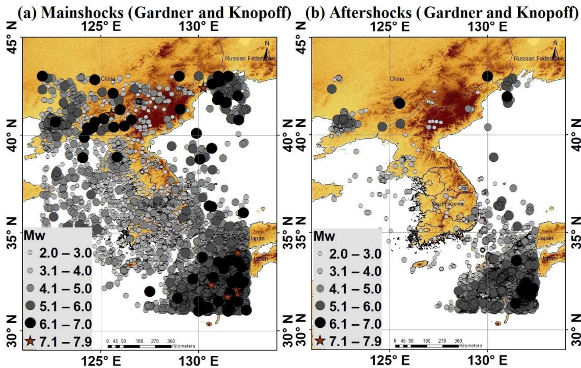
Figure 7: Declustered seismicity distribution map using the Gardner and Knopoff method depicting (a) for mainshocks and (b) for aftershocks, covering the period from 1905 to 2023.
