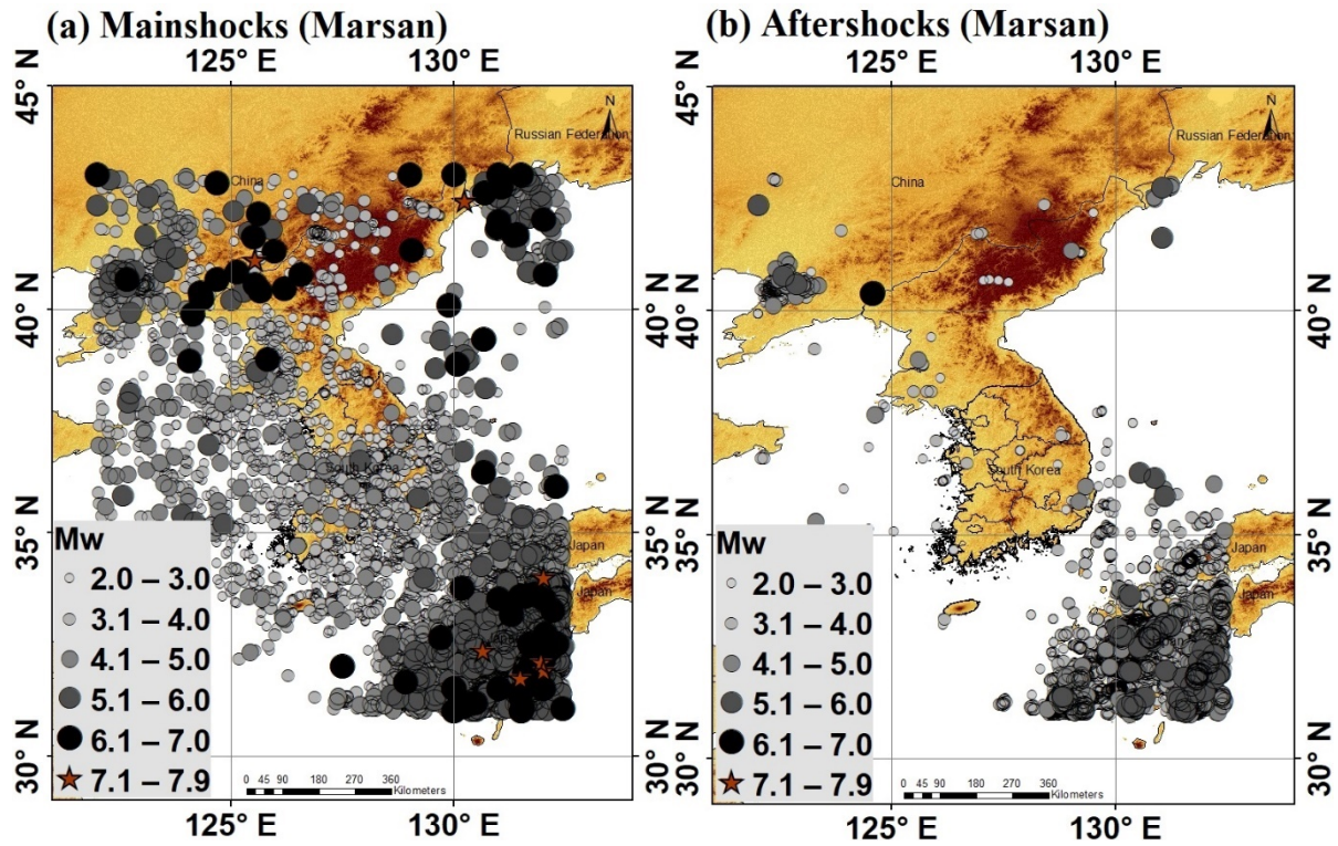
Figure 13: Declustered seismicity map using the Marsan algorithm depicting (a) for mainshocks and (b) for aftershocks, covering the period from 1905 to 2023.
