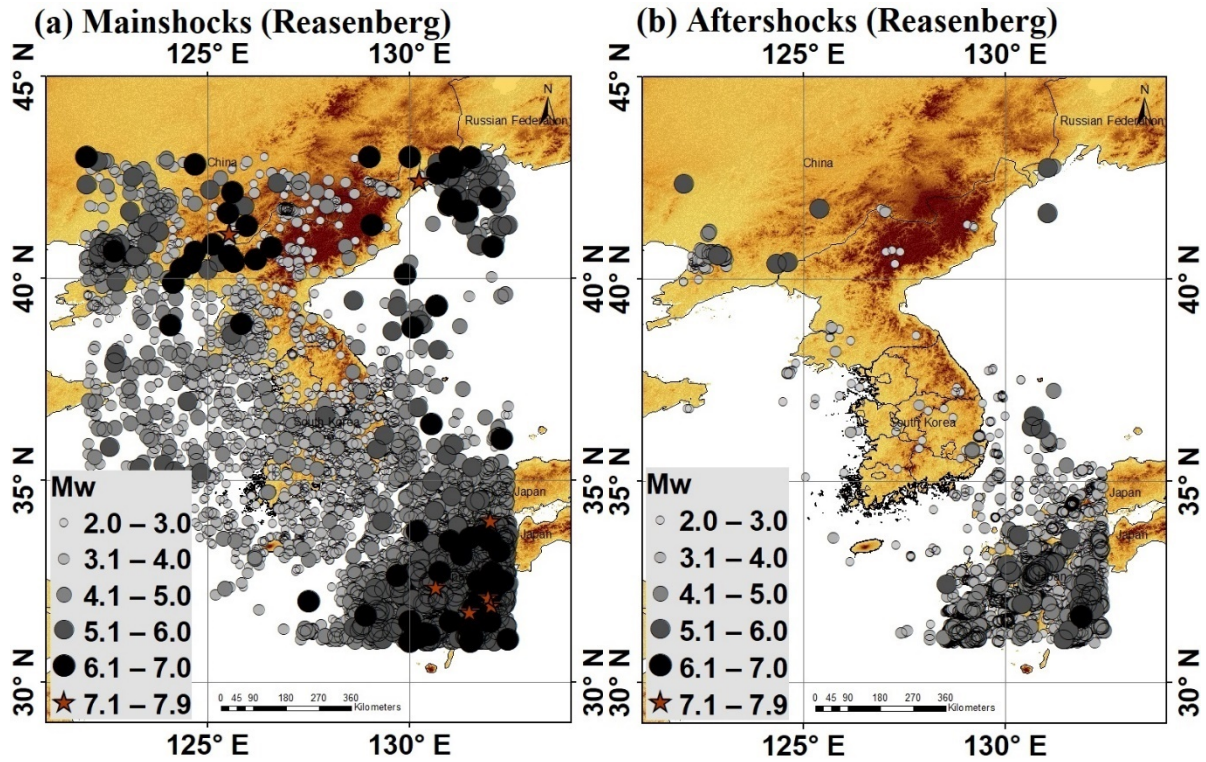
Figure 11: Declustered seismicity map using the Reasenberg algorithm depicting (a) for mainshocks and (b) for aftershocks, covering the period from 1905 to 2023.
