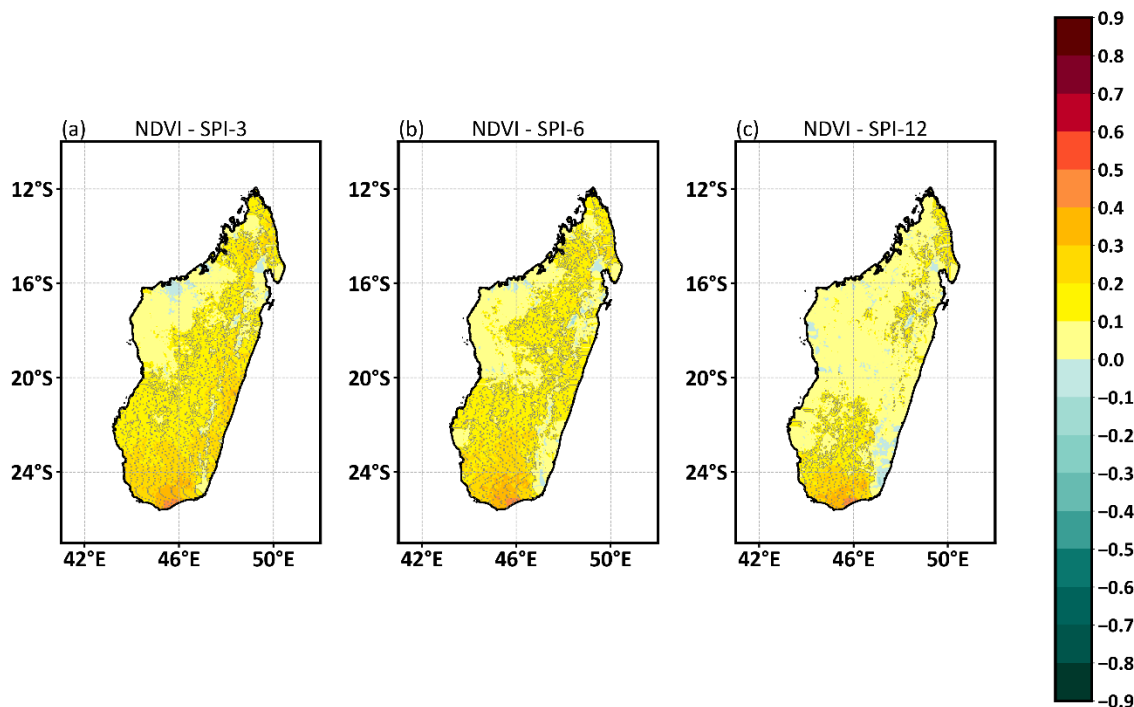
Figure 11: Spatial distribution of the Pearson correlation between detrended NDVI anomaly and drought index for all three timescales (SPI-3, -6, -12). Dotted areas are statistically significant at 95% confidence level using a student's t-test.
