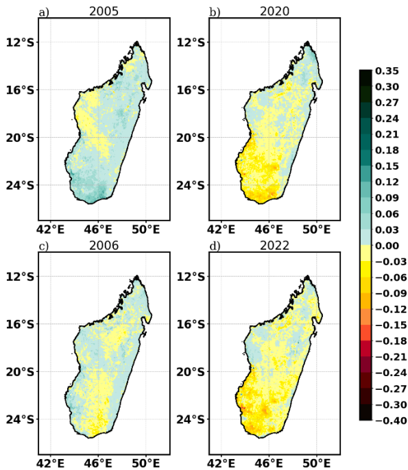
Figure 8: NDVI difference (anomaly) between selected years and the NDVI yearly mean throughout the whole study period. The years are selected based on the continuous and simultaneous negative SPI values found during the seasonal and annual analyses from Fig. S2 as marked with green rectangles. a) and c) represent the difference at the beginning and the ending of the first
