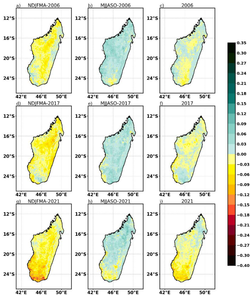
460 Figure 9: Seasonal and annual NDVI difference between selected years and NDVI seasonal and annual mean throughout the study period. The years 2006, 2017 and 2021 were chosen based on smaller negative values found during the wet season from Fig. S2a as marked with green circles. a), d), g) represent the differences during the wet season of each mentioned year. b), e), h) represent the differences during the dry season of each mentioned year. c), f), i) represent the differences for the annual averaged NDVI of each mentioned year.
