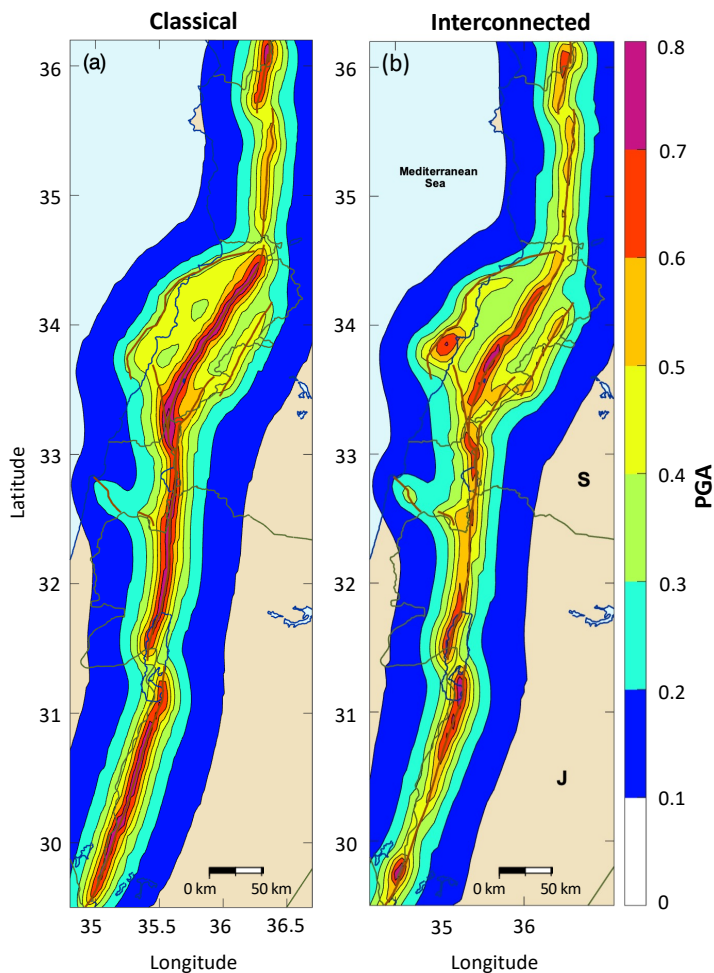
Figure 8 : Seismic hazard maps, PGAs at a 475 year return period (a) based on the classical implementation of faults, assuming that the maximum magnitude is M_{max} 7.5, (b) based on the interconnected model assuming M_{max} 7.5 (maximum jump 10km, ruptures cannot jump major discontinuities). Generic rock site condition ( V_{S30}=760 m/s).
