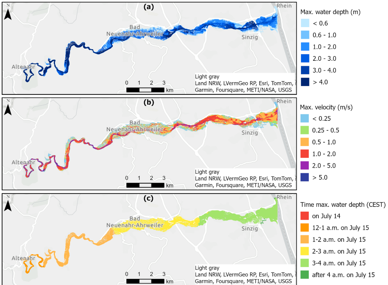
240 Figure 4: Flood characteristics of the 2021 Ahr Valley flood simulated with RIM2D at a resolution of five meters. (a) Maximum water depth. (b) Maximum flow velocities. (c) Time of maximum water depth.
