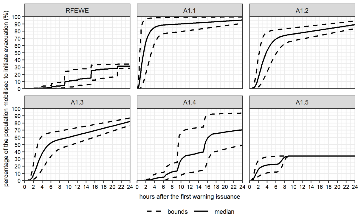
395 Figure 7: Combination of the warning diffusion and mobilisation curves for each alternative scenario of early warning and evacuation in the first approach. RFEWE (reconstructed scenario of the 2021 flood), A1.1 (optimal scenario), A1.2 (intermediate scenario), A1.3 (suboptimal scenario), A1.4 (suboptimal with empirical warning diffusion curve), and A1.5 (suboptimal with empirical mobilisation curve).
