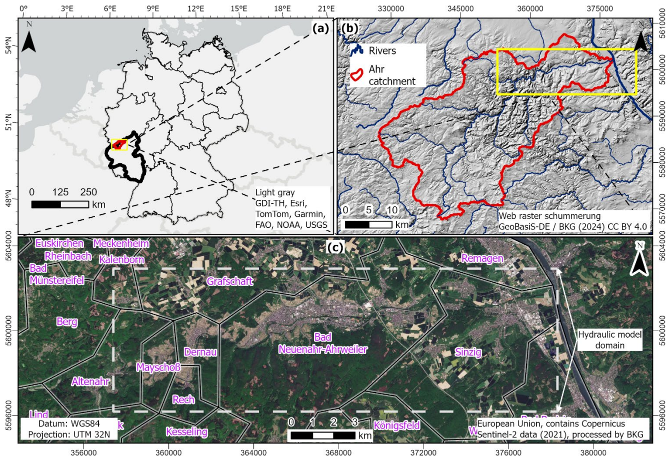
210 Figure 3: Overview of the Ahr Valley and its most impacted area by 2021 flood. (a) Germany Federal States, highlighting Rhineland-Palatinate and the location of the Ahr Valley catchment. (b) Ahr Valley catchment with drainage system and hillshade base map. (c) Satellite image and local administrative units of the downstream portion and most impacted area of the Ahr Valley, between the cities of Altenahr and Sinzig, at the confluence with the Rhine River. Data sources: Germany Federal states and local administrative units: GeoBasic DE / BKG (2023); Rivers and Ahr catchment: Global dataset of drainage systems (He et al., 2024).
