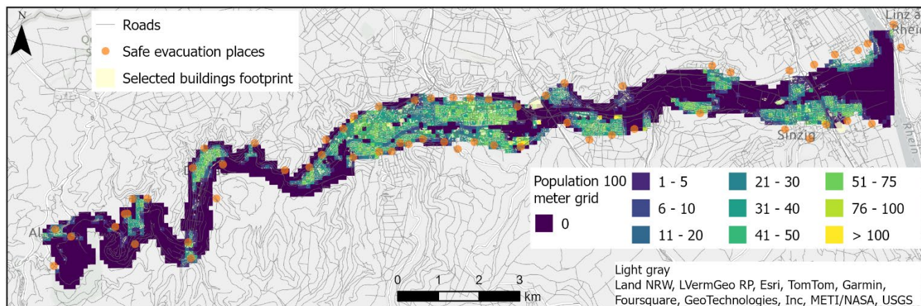
285 Figure 5: Overview of exposure at building scale. Population counts aggregated at a 100 meter grid resolution, buildings and road network along the Ahr Valley, simulated flood extent, and safe places. Data sources: 100 meter grid: HANZE 2.0.3 (Paprotny, 2023). Roads and buildings: © OpenStreetMap contributors 2021. Distributed under the Open Data Commons Open Database License (ODbL) v1.0.
