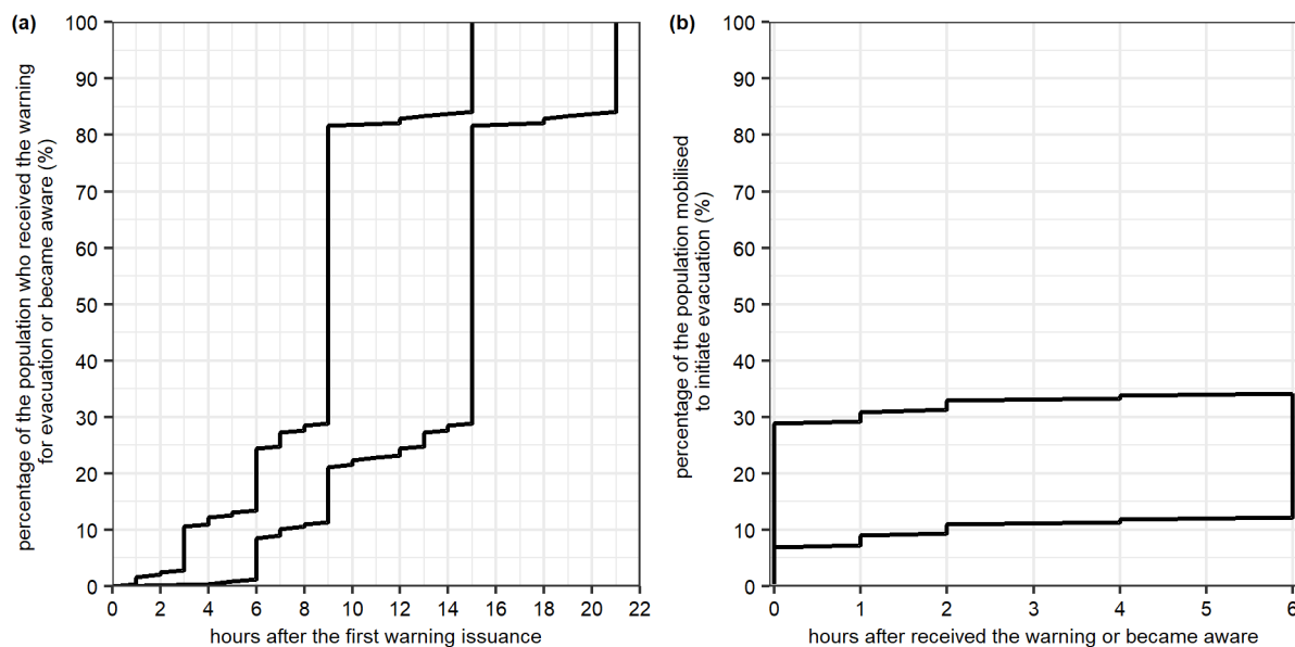
340 Figure 6: Reconstruction of warning diffusion and mobilisation times in the Ahr Valley 2021 flood based on the post-event survey with flood affected residents. (a) Warning diffusion curve: cumulative proportion of the population who were warned or became aware of the hazard after the first flood warning. (b) Mobilisation curve: cumulative proportion of the population who initiated an outdoor evacuation after receiving or becoming aware of the hazard.
