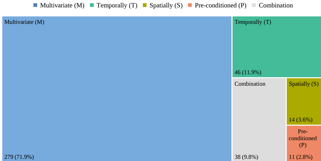
Figure 2. Count of the number of studies reviewed for each compound event category, and their combinations (in grey) (total = 388 events). The percentage (%) indicated is the proportion of all compound event types studied.
