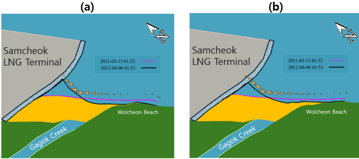
330 Figure 17: Comparison of LST vector results over the entire analysis period: (a) from satellite images; (b) from the shoreline change model.
