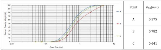
160 Figure 6: (a) Sand collection location and (b) survey results for cumulative grain size curves and median grain sizes for sand ( D_{50} ) at Gagok Creek estuary (source: GSESRH, 2013; © Google Earth).
