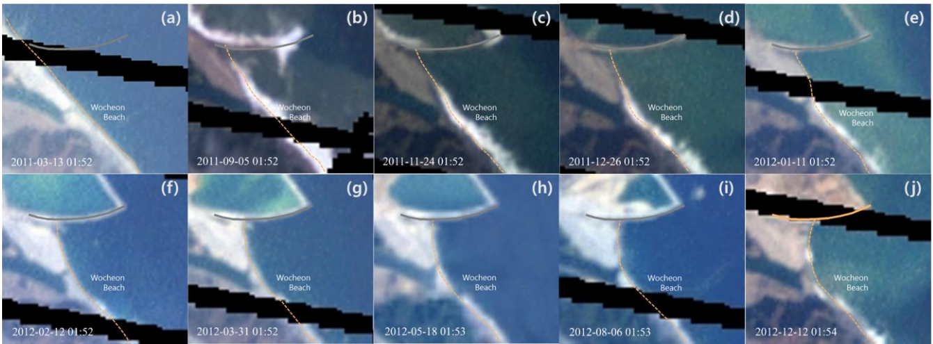
Figure 7: Satellite images of Landsat-7 selected for Wolcheon Beach shoreline analysis from 2011– 2012, and extracted shorelines: (a) 2011.03.13; (b) 2011.09.05; (c) 2011.11.24; (d) 2011.12.26; (e) 2012.01.11; (f) 2012.02.12; (g) 2012.03.31; (h) 2012.05.18; (i) 2012.08.06; (j) 2012.12.12 (© Google Earth).
