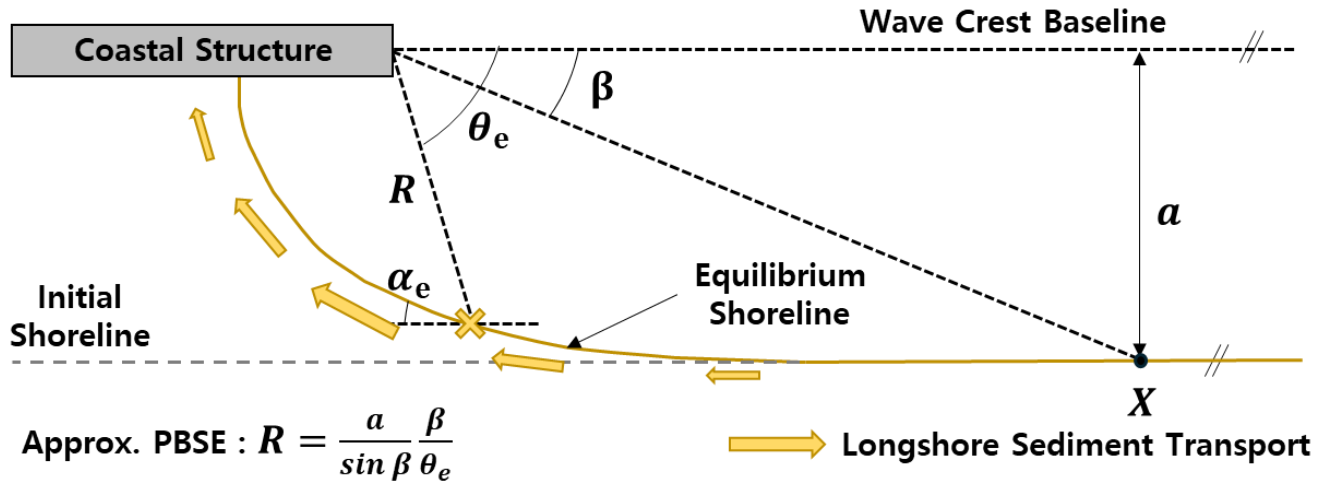
215 Figure 9: Definition sketch for estimation of initial LST owing to coastal structure construction.
