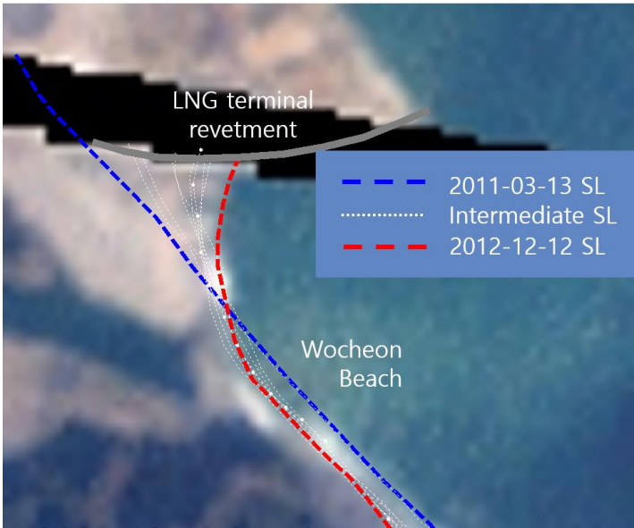
Figure 8: Shoreline changes from Landsat-7 satellite images of Wolcheon Beach from 2011–2012 (© Google Earth).
