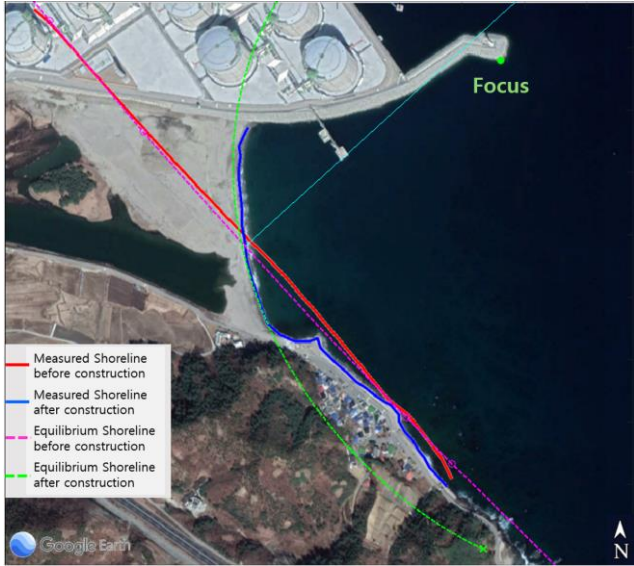
255 Figure 11: Change in equilibrium shoreline after reclamation estimated using MeePaSoL (© Google Earth).
