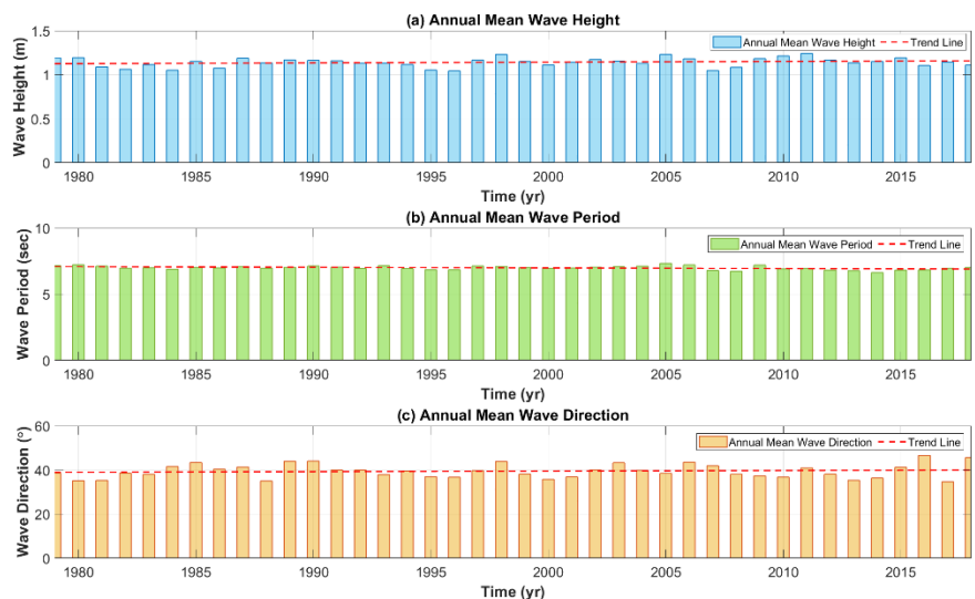
135 Figure 3: Changes in annual mean: (a) wave height, (b) wave period, and (c) wave direction obtained from NOAA wave data near Wolcheon Beach.
