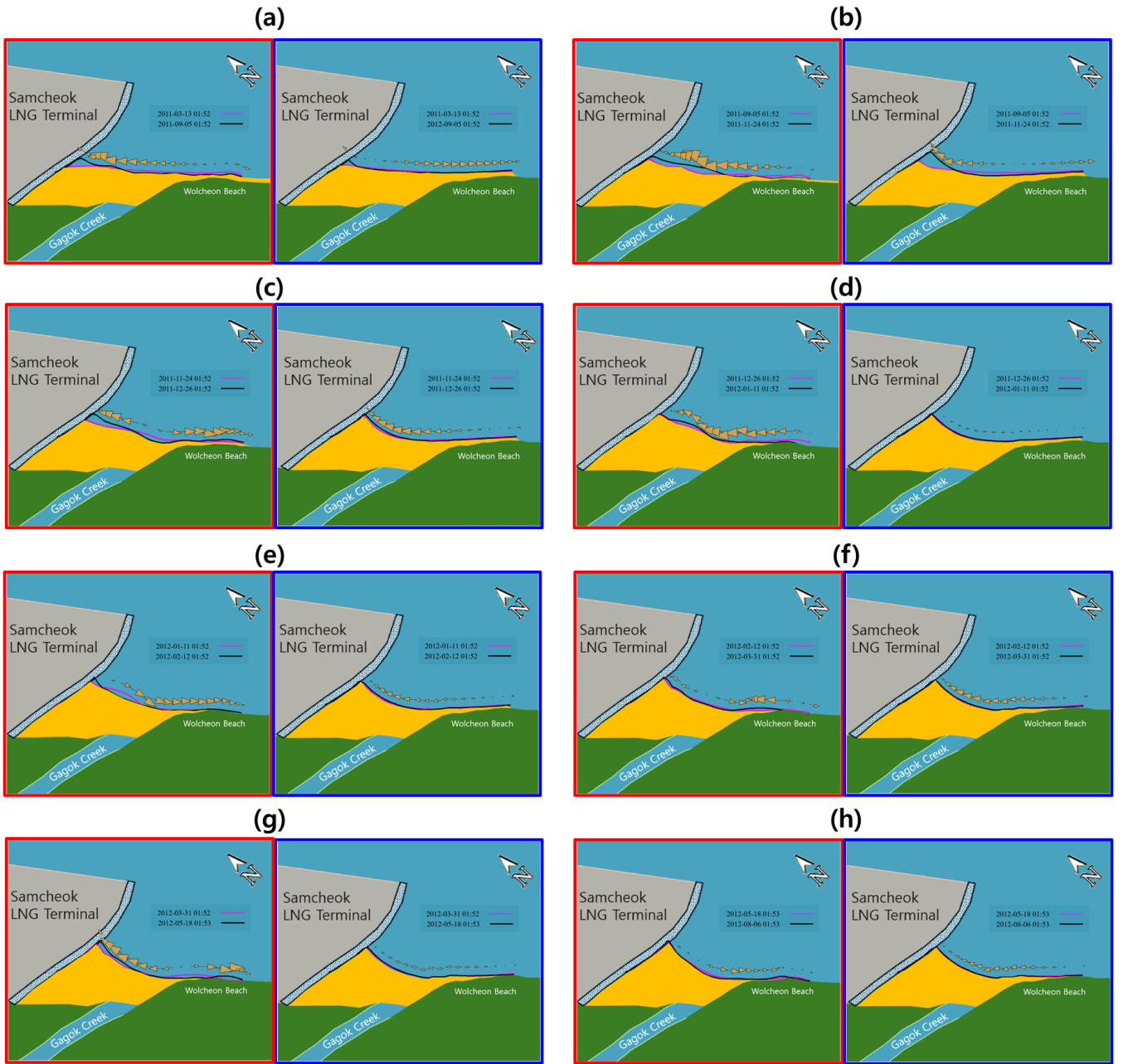
Figure 16: Comparison between LST vectors obtained from satellite images (left; red boxes) and numerically simulated LST vectors (right; blue boxes): (a) 2011.03.13 – 2011.09.05; (b) 2011.09.05 – 2011.11.24; (c) 2011.11.24 – 2011.12.26; (d) 2011.12.26 – 2012.01.11; (e) 2012.01.11 – 2012.02.12; (f) 2012.02.12 – 2012.03.31; (g) 2012.03.31 – 2012.05.18; (h) 2012.05.18 – 2012.08.06.
