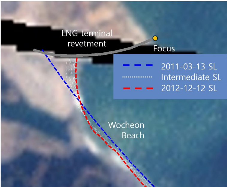
295 Figure 14: Numerical results of shoreline changes on Wolcheon Beach from March 13, 2011 to December 12, 2012 (© Google Earth).
