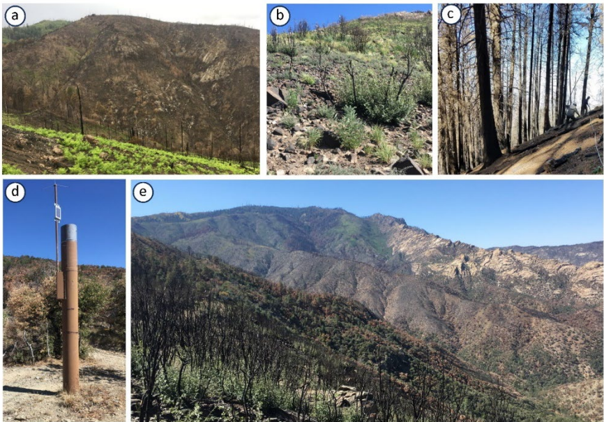
100 Figure 2. (a) Photo taken on 7 July 2020 of small tributaries at the headwaters of the CDO watershed, near the MLFD rain gauge. The area burned primarily at moderate and high severity. (b) Photo taken in October 2020 of a hillslope, which burned at moderate 105 severity in the 2003 Aspen Fire and moderate severity in the 2020 Bighorn Fire, near the MLFD rain gauge. (c) Photo taken in October 2020 of a hillslope near the C2 rain gauge, which did not burn in the 2003 Aspen Fire and was burned at moderate severity in the 2020 Bighorn Fire. (d) The Automated Local Evaluation in Real Time (ALERT) rain gauge installed at Dan’s Saddle (1140). (e) A view of the headwaters of the CDO watershed in October 2020.
