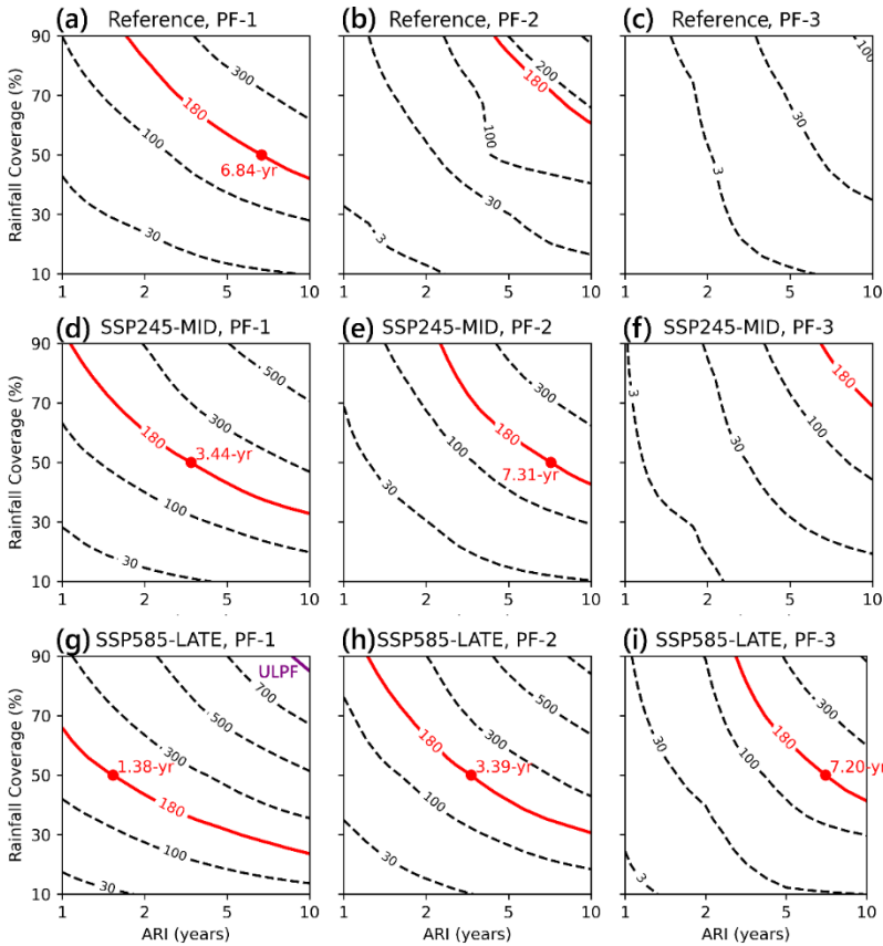
345 Figure 7. Contours of peak discharge ( \text{m}^3/\text{s} ) of simulated floods produced by design storms of varying average recurrence intervals (ARI) and rainfall coverages (from 10% to 90%) during the first three postfire (PF) years for reference and future scenarios at the CDO watershed. The thick red contours represent the 100-year flood ( 180 \text{ m}^3/\text{s} ), as derived from StreamStats ( https://www.usgs.gov/streamstats ; Paretti et al., 2014). Red dots indicate the ARIs of the storms that can produce a 100-year flood
