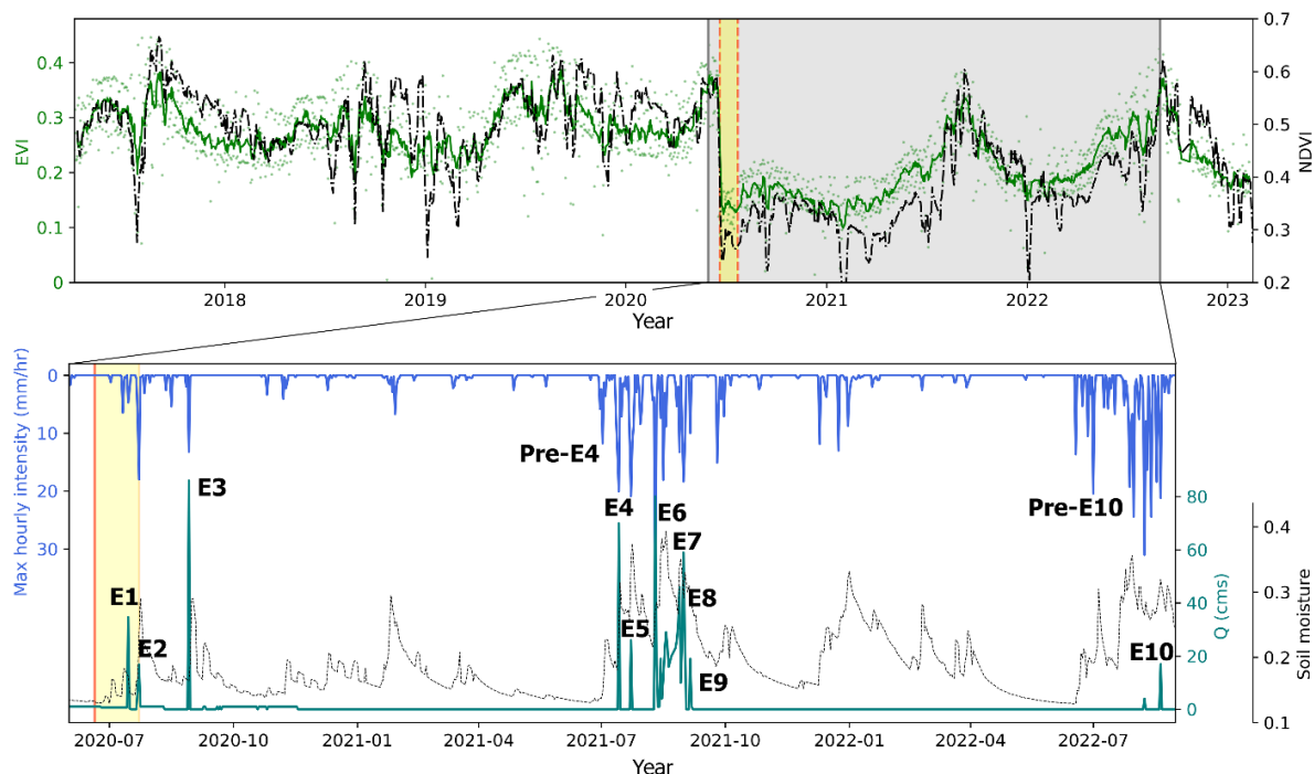
140 Figure 3. The 12 simulated events occurred after the ignition of the 2020 Bighorn Fire. The Enhanced Vegetation Index (EVI) and Normalized Difference Vegetation Index (NDVI) data, were derived from MODIS Terra satellite imagery at a resolution of 500 meters. Rainfall measurements collected by six Automated Local Evaluation in Real Time (ALERT) tipping bucket rain gauges maintained by the Pima County Regional Flood Control District (PCRFC), supplemented by four additional gauges we installed 145 during the study period (referenced in Figure 1). The maximum hourly rainfall intensity was estimated using these rain gauge data with the Thiessen polygon method. Runoff hydrographs at the outlet of the CDO watershed were obtained from a PCRFC- maintained streamflow gauge.
