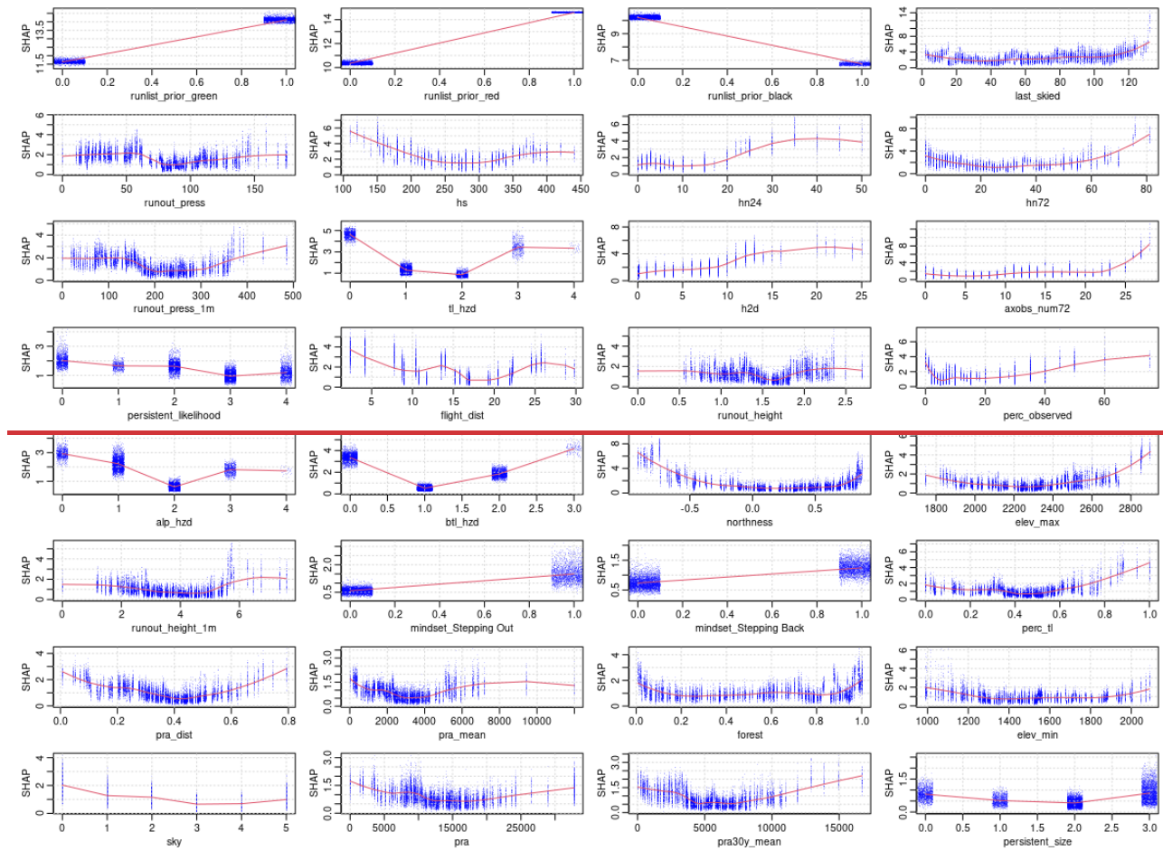
Figure C1: Grid of SHAP plots for the top 32 features ranked by feature importance relative to the overall classification.
