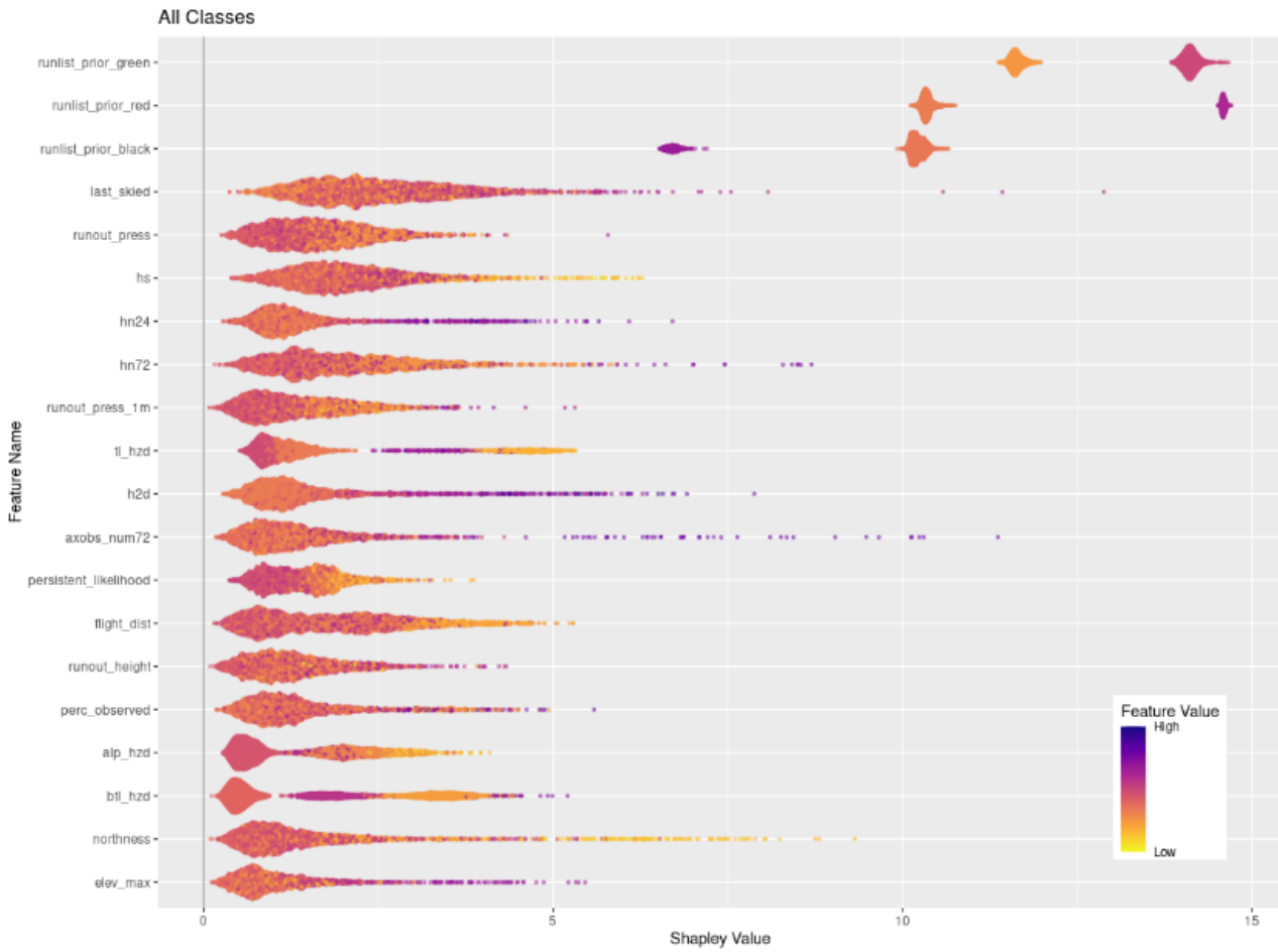
Figure C12: SHAP value summary plot with features ranked by feature importance relative to the overall classification on the y-axis, SHAP value on the x-axis, and the relative value of the individual features shown with color coded points.
