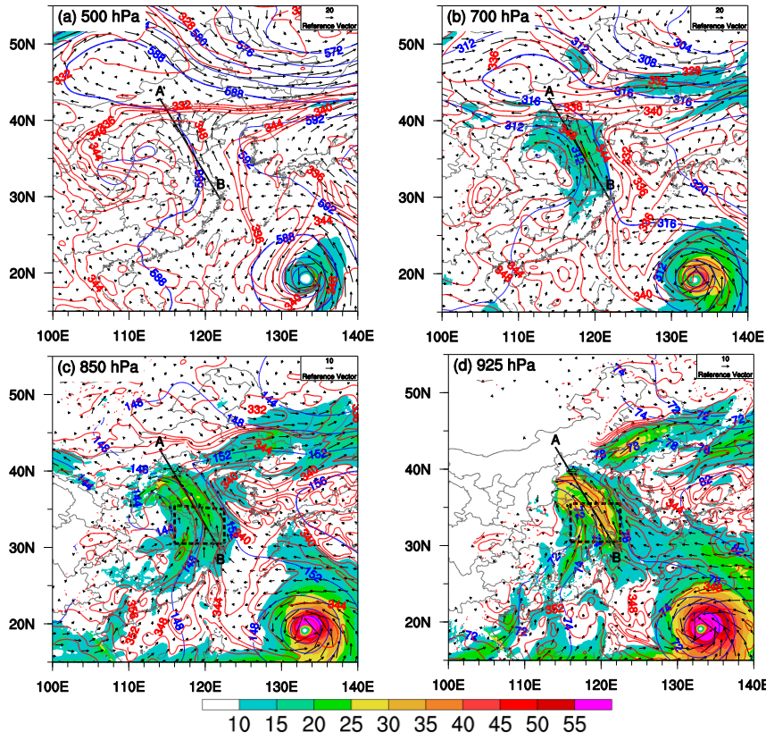
317 Fig. 9 Spatial distribution of geopotential height (blue contoured at 40 gpm), equivalent 318 potential temperature (red contoured at 2K intervals, \theta_e ), wind bars (a full barb is 4 m s -1 ), and 319 water vapor flux ( \text{g s}^{-1} \text{cm}^{-1} \text{hPa}^{-1} , shadings) from the model D01 at 0000 UCT 30 July 2023: 320 (a) 500 hPa, (b) 700 hPa, and (c) 850 hPa, and (d) 925 hPa. The isolines of 588, 316, and 156 321 are bolded to represent the WPSH at 500 hPa, 700 hPa, and 850 hPa, respectively. The 322 convergence zone of southeast and southwest flows is marked by a dashed line box in panels 323 (c) and (d). The thick black line A–B denotes the locations for cross-section along the water 324 vapor transport pathway used in Fig. 10.
