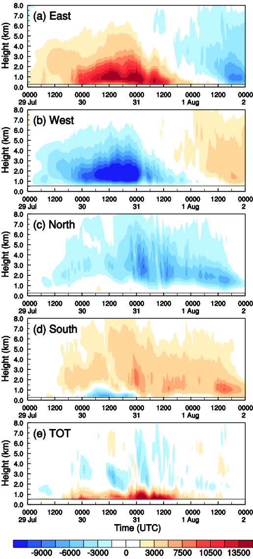
Fig. 13 Time-height cross sections of moisture fluxes ( \text{kg kg}^{-1} \text{ m}^2 \text{ s}^{-1} ) through the (a) eastern, (b) western, (c) northern, and (d) southern boundaries of the MTG region in Fig. 1; (e) TOT provides the total net moisture flux of all boundaries.
