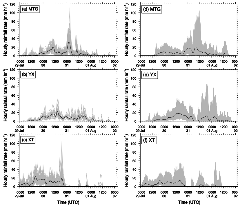
250 Fig. 7 Time series of (a-c) rain gauge observations and (d-f) simulation hourly rainfall rates 251 (gray lines, \text{mm hr}^{-1} ) for all stations/grid points over the (a, d) MTG, (b,e) YX, and (c,f) XT 252 regions during the period of 0000 UTC 29 July to 0000 UTC 02 August 2023. The black line 253 denotes the domain-averaged hourly rainfall rates of all stations (grid points) from observations 254 (simulations). (see Fig. 1 their locations). In total, 74, 19, and 67 observations are used for (a) 255 MTG, (b) YX, and (c) XT, respectively. For the simulation, there are (d) 2296, (e) 2365, and (f) 256 2420 grid points.
