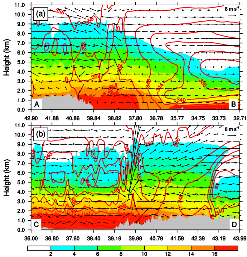
388 Fig. 12 Vertical cross-sections along lines (a) A–B and (b) C–D given in Fig. 11 of equivalent 389 potential temperature ( \theta_e , red-contoured at 4K intervals), water vapor mixing ratio ( q_v , g kg -1 , 390 shadings), and in-plane flow vectors (vertical motion amplified by a factor of 10) at 0800 UCT 391 31 July 2023. Gray shadings denote terrain.
