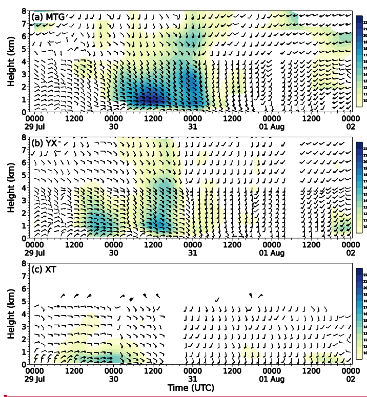
Fig. 2 Temporal evolution of wind profile (a full barb is 4 \text{ m s}^{-1} , and shadings denote wind speed over 10 \text{ m s}^{-1} ) from observations near (a) MTG, (b) YX, and (c) XT during the period of 0000 UTC 29 July to 0000 UTC 2 August 2023. Note only the wind profile below 5 km above the ground can be observed due to the limitation of the instrumentation near Xingtai (XT). (see Fig. 1 their locations).
