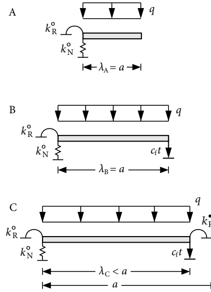
Figure 2. Boundary conditions of the unsupported segment. Reactions by the slab resting on the intact weak layer ( \circ ) are represented by linear and rotational springs with stiffnesses k_N^o and k_R^o , respectively. Deflections are limited to a fraction f_c t of the weak layer thickness. Moments introduced by the slab resting on the collapsed weak layer ( \bullet ) are represented by rotational springs of stiffness k_R^\bullet .
