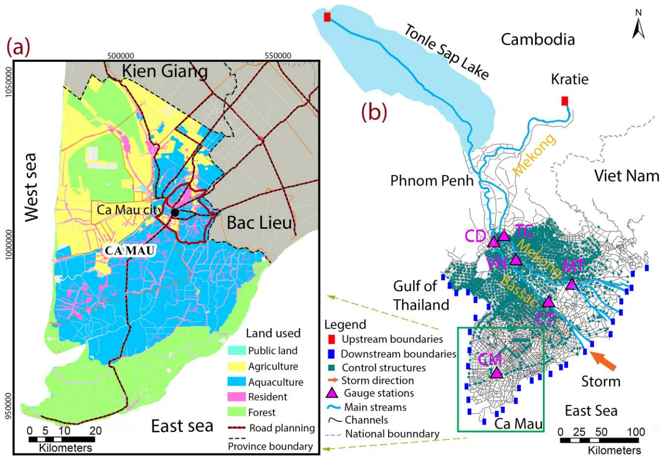
Figure 1. (a) Location of the study area and land use data for the year 2022 (The People's Committee of Ca Mau Province, 2023); (b) the 1D model used in this study
