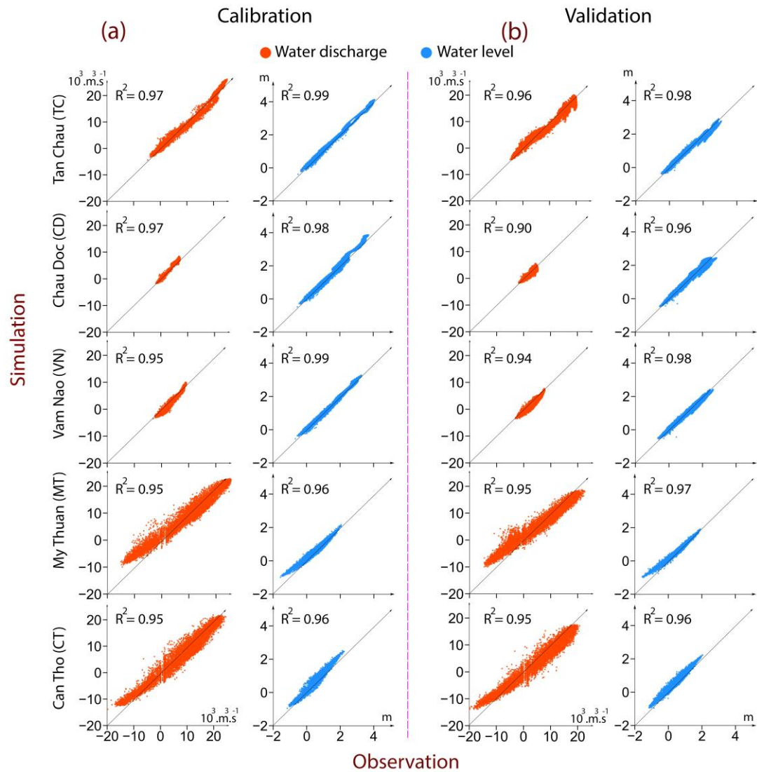
230 Figure 3. Assessing the agreement between the predicted and observed hourly data for water level and water discharge at monitoring stations throughout the VMD during the calibration run in 2018 and validation run in 2016 along with the coefficient of determination ( R^2 ).
