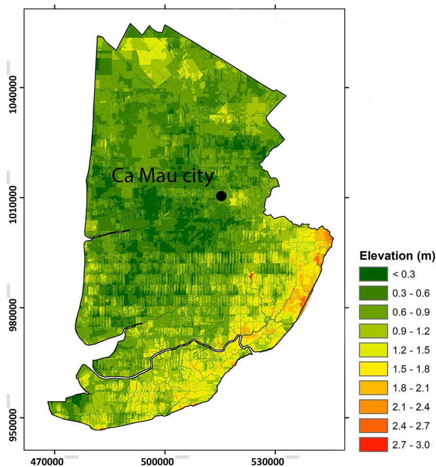
600 Figure A1. DEM illustrates the flat terrain of the CMP acquired from the Ministry of Natural Resources and Environment (MONRE) in 2008 (Tran et al., 2016).
