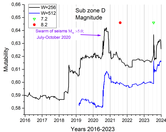
Figure 12. Mutability on magnitude for the 908 seisms of sub zone D. An empty green triangle identifies the time for the largest seisms of this subzone, while a solid red circle marks the time of the largest seisms of the whole zone under study.
