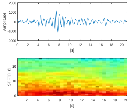
(a) Long Period Event (LPE)
