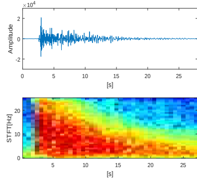
(b) Volcano-Tectonic Earthquake (VTE)
