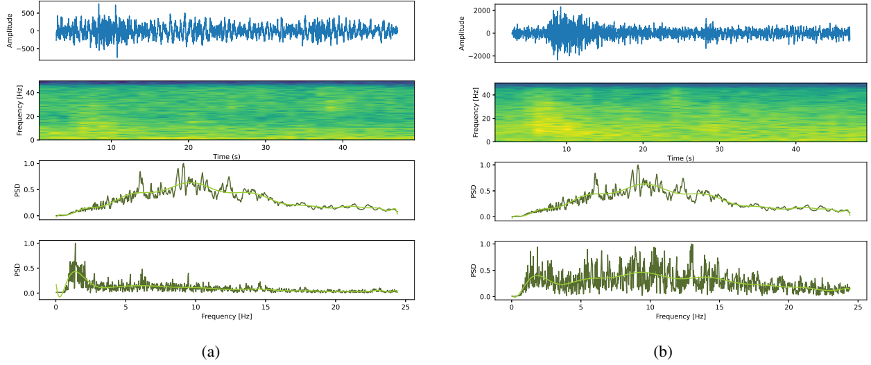
Figure 10. Example of two earthquakes annotated in the catalog that were not detected by any of the 3 reference systems. a) Spectral analysis of an undetected earthquake, where a clear attenuation of energy at high frequencies is observed. b) Spectral analysis of an undetected earthquake, where an energy distribution in intermediate frequencies and attenuation at high frequencies are observed.
