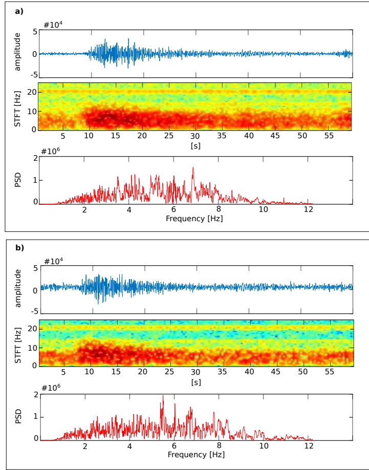
Figure 6. Two examples of event annotated as VTE in the POPO2002 catalogue being recognized as TRE for the systems. The current colormap in the spectrogram represents the energy levels. The blue color corresponds to the minimum energy, while the red color corresponds to the maximum energy. The PSD reflects the distribution of a signal’s energy among the frequencies.
