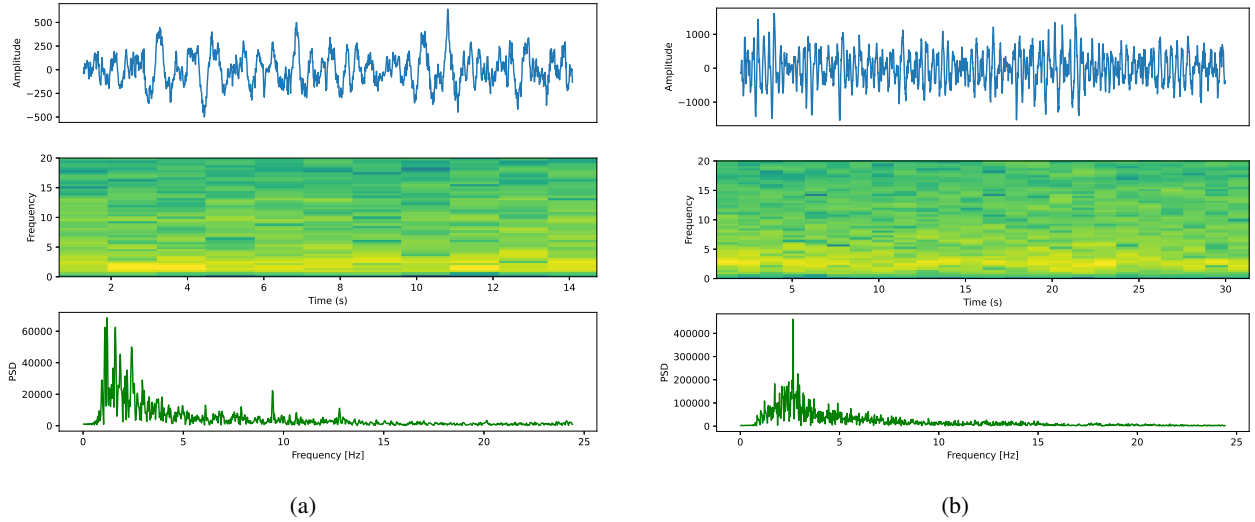
Figure 12. Example of a) LPE detected but not annotated and b) TRE detected but not annotated in the catalog.
