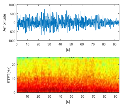
(c) Tremor (TRE)
