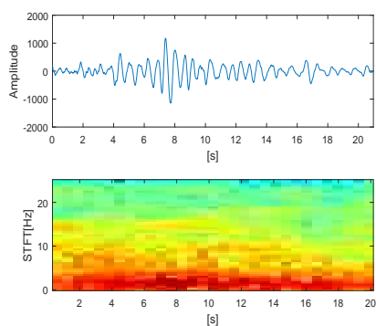
(a) Long Period Event (LP)
