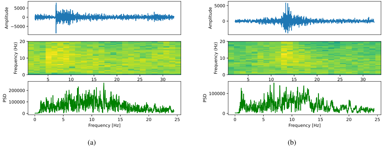
Figure 11. Example of two earthquakes not annotated in the catalog that were detected by the 3 reference systems with probabilities ranging from 63% to 78%.
