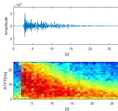
(b) Volcano-Tectonic Earthquake (VT)
