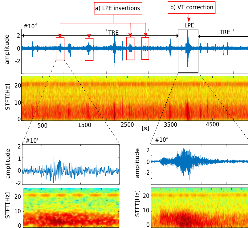
Figure 4. Insertion-based errors when retraining systems using a weakly supervised approach. Detection of LP events (red boxes) that were initially overlooked during the labeling process within a trace labeled as TRE–LPE–TRE. Correction of an event originally labeled as LP, which the system now re-labels as VT. This scenario occurs frequently throughout the dataset, and these additions reduce per-frame recognition accuracy compared to the original labeling; however, they do not always indicate errors.
