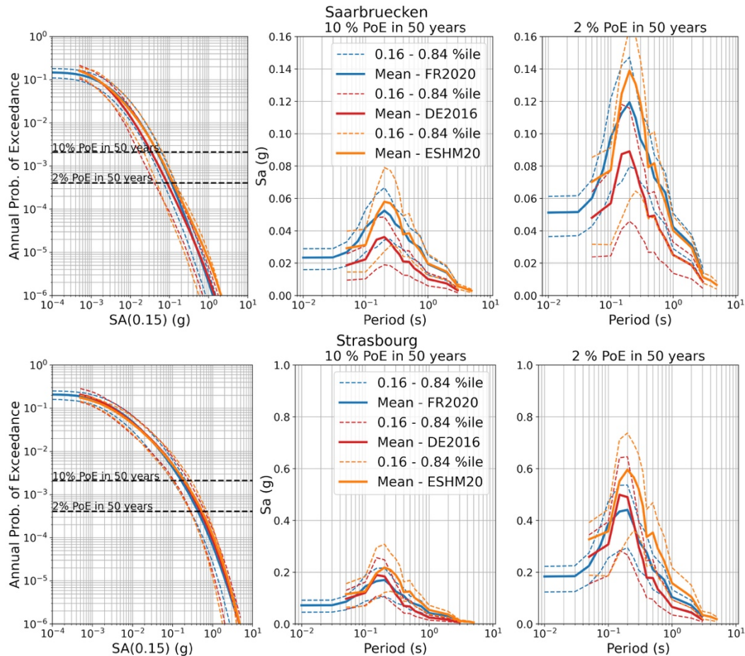
Figure 22. Comparison of the distributions of seismic hazard for Saarbrücken (top row) and Strasbourg (bottom row) for hazard curves at Sa (0.15 s) (left) column) and UHS for 10 % PoE in 50 years (middle column) and 2 % PoE in 50 years (right column)
