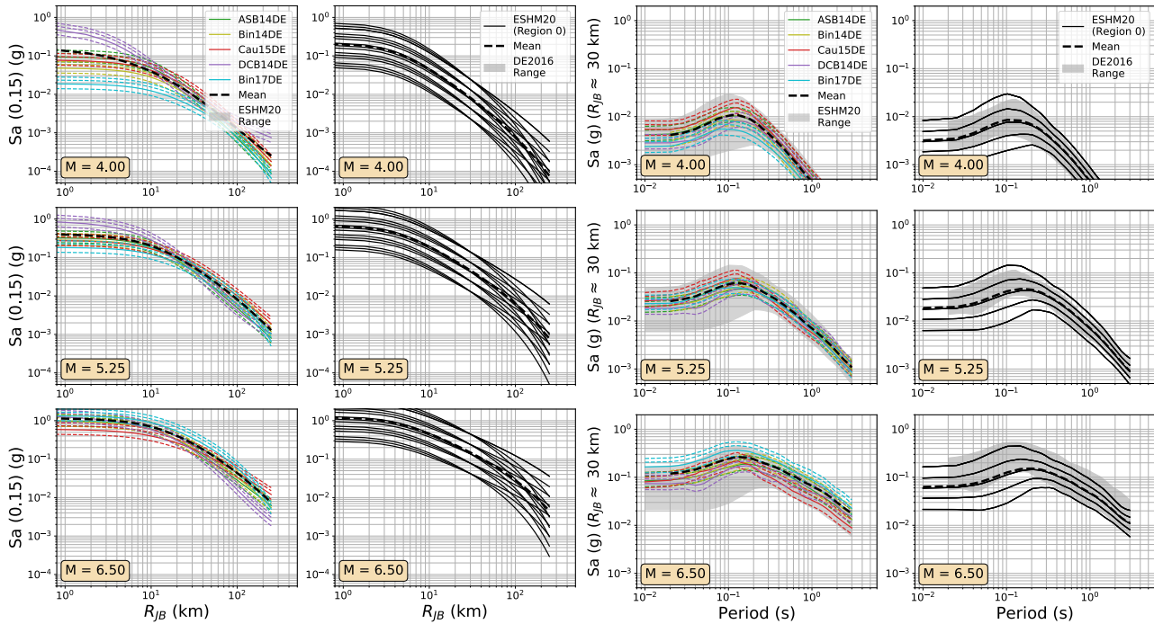
Figure 10: As Figure 7, comparing the median ground motions ESHM20 and DE2016 GMM logic trees
