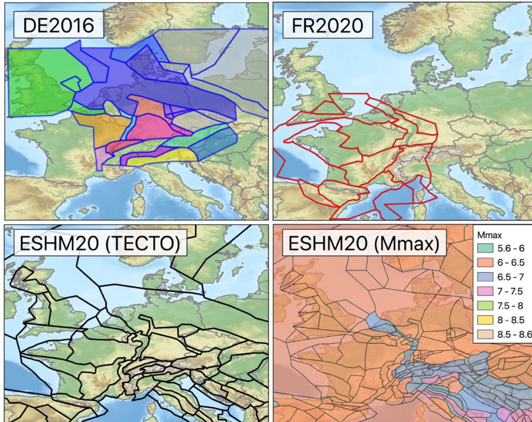
330 Figure 5: Large-scale area source zonations (LASZ) assumed for DE2016 (top left), FR2020 (top right) and the two LASZ zonations for ESHM20 based on regional tectonics (bottom left) and maximum magnitude (bottom right). Colours for DE2016 indicate the groupings of LASZ (from Model A) sharing a common b-value.
