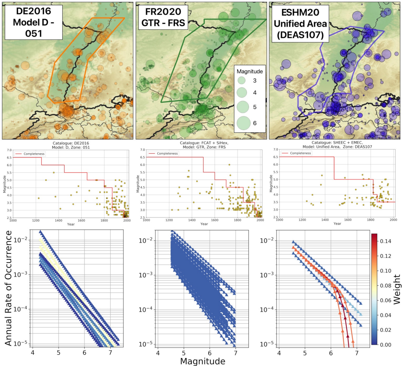
410 Figure 6: Example comparison of fit and representation of earthquake recurrence for the Upper Rhine Graben (URG) for the DE2016 (left column), FR2020 (middle column) and ESHM20 (right column). Example geometry of the selected URG seismic source in different models and the respective earthquake catalogues with symbols scaled according to magnitude (top row), distribution 415 magnitude with time for the respective zones and the corresponding temporal completeness magnitude assumed by the model (middle row), and distribution of magnitude frequency relations for the zone colour scaled according to weight. All catalogues share the same symbol size scaling with magnitude (top row) and all magnitude frequency distributions share the same colour scale (bottom row).
