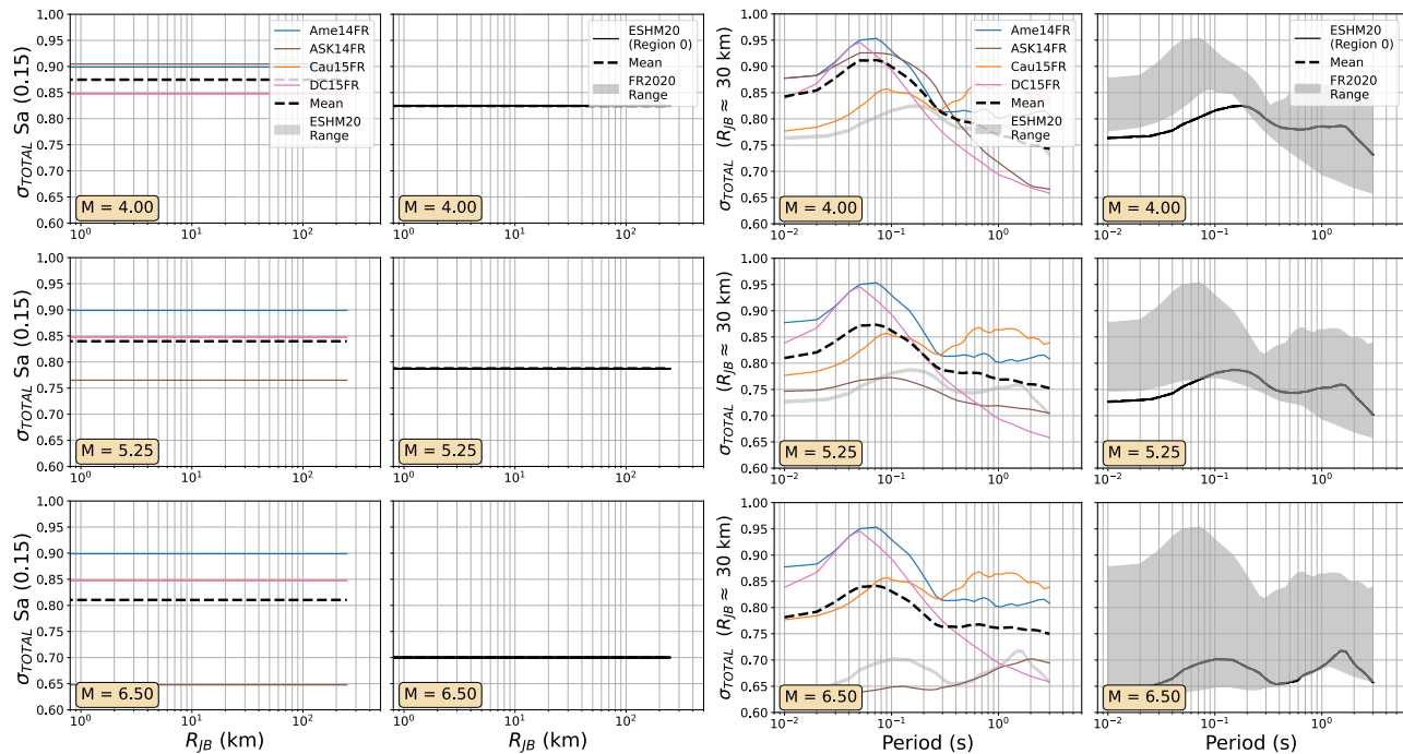
575 Figure 11. As Figure 8, comparing the aleatory uncertainty distributions of the FR2020 and ESHM2020 GMM logic trees
