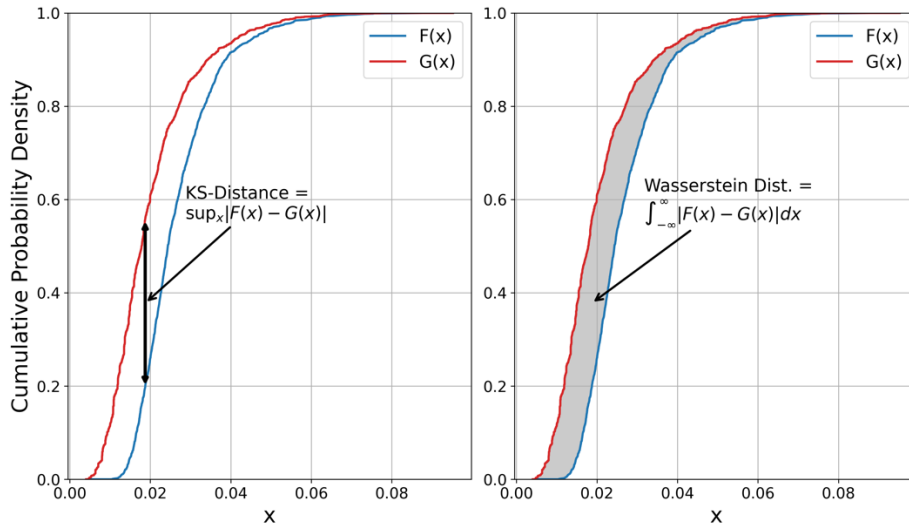
840 Figure 16. Definition of the Kolmogorov-Smirnov (KS) statistic (left) and Wasserstein Distance (right) with respect to empirical CDFs F(x) and G(x)
