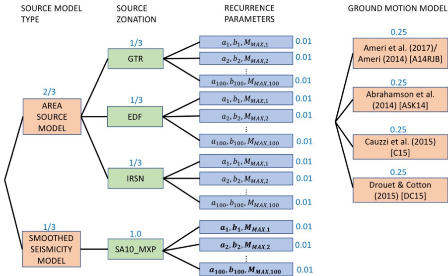
Figure 3. Complete logic tree for France (Drouet et al., 2020) containing both the seismogenic source model and ground motion model
