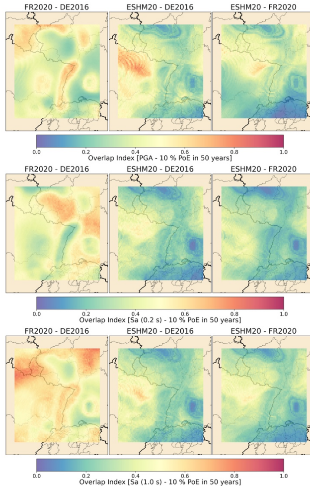
940 Figure 21: As Figure 20 considering the overlap index (OI)
