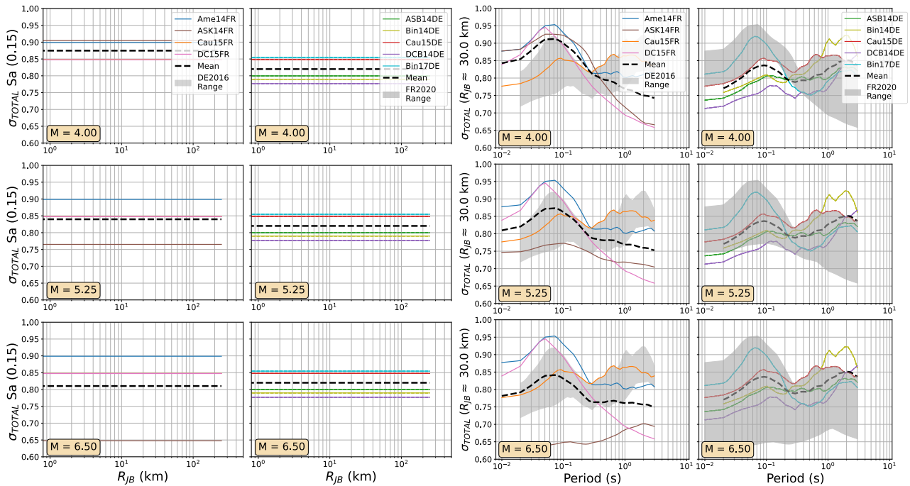
Figure 8: As Figure 7, comparing the aleatory uncertainty distributions of the FR2020 and DE2016 GMM logic trees. The dashed black lines refer to the sum of the aleatory variabilities of each GMM ( \sigma_i ) weighted by their logic tree weight ( w_i ): \sum_i(\sigma_i \cdot w_i)
