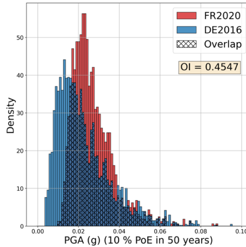
905 Figure 19: Illustration of the Overlap Index (OI) between the distribution of hazard at a site using the FR2020 and DE2016 models
