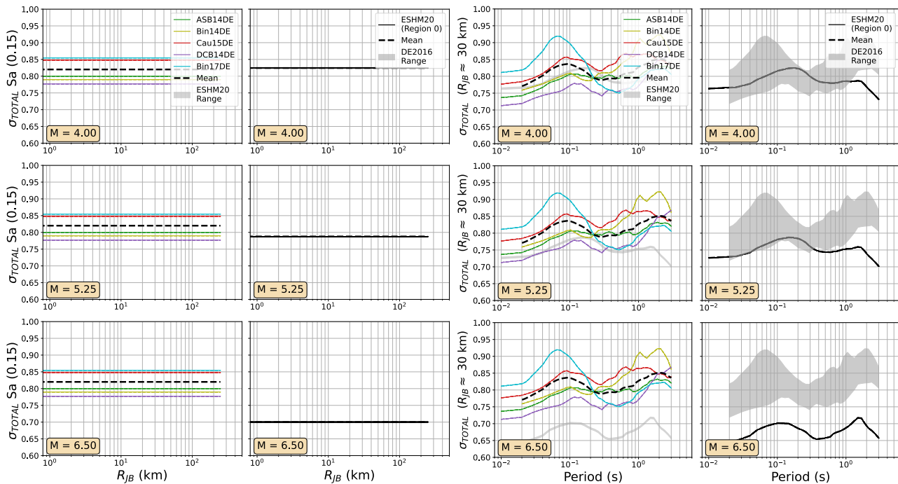
585 Figure 12: As Figure 8, comparing the aleatory uncertainty distributions of the ESHM20 and DE2016 GMM logic trees
