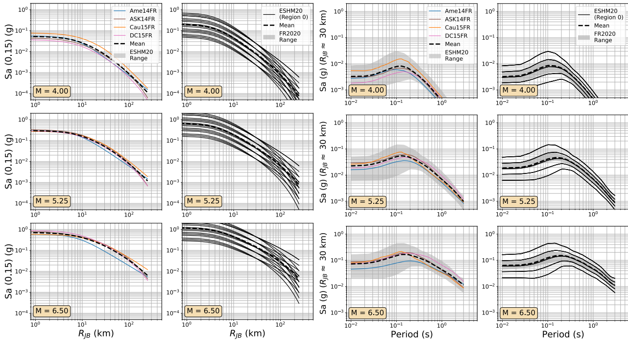
Figure 9. As Figure 7, comparing the median ground motions of the ESHM20 and FR2020 GMM logic trees
