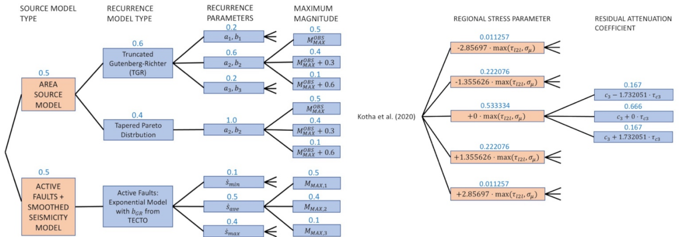
Figure 4. Complete logic tree of seismogenic source models (left) and ground motion models (right) for ESHM20 (Danciu et al. 2021)
