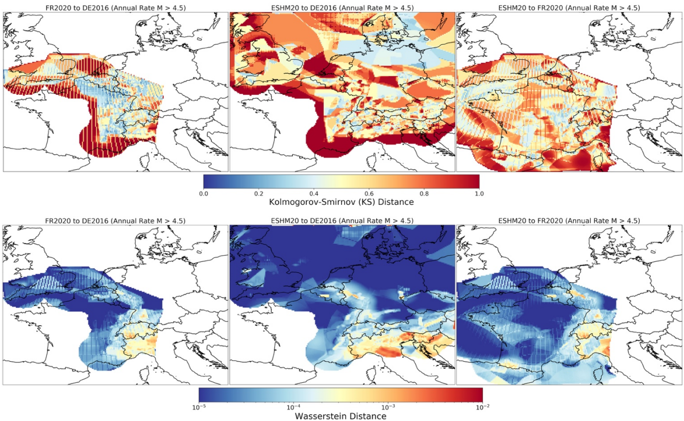
870 Figure 17: Seismicity rate distribution differences between the models given in terms of KS Distance, D_{KS} (top row), and Wasserstein Distance, D_{WS} (bottom row): FR2020 to DE2016 (left), ESHM20 to DE2016 (middle), and ESHM20 to FR2020 (right)
