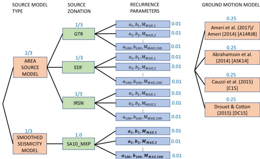
Figure 2. Complete logic tree for France (Drouet et al., 2020) containing both the seismogenic source model and ground motion model
