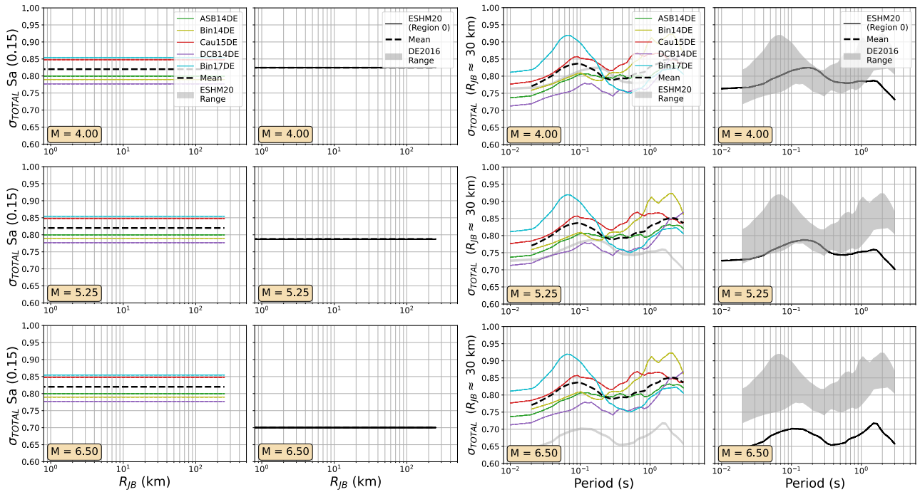
Figure 11: As Figure 7, comparing the aleatory uncertainty distributions of the ESHM2020 and DE2016 GMM logic trees
