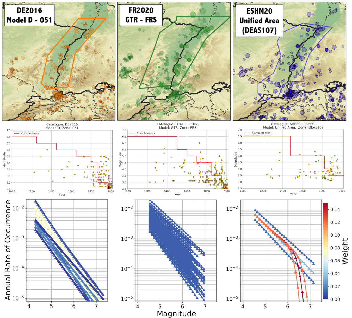
405 Figure 5: Example comparison of fit and representation of earthquake recurrence for the Upper Rhine Graben (URG) for the DE2016 (left column), FR2020 (middle column) and ESHM20 (right column). Example geometry of the selected URG seismic source in different models (top row), distribution magnitude with time for the respective zones and the corresponding temporal completeness magnitude assumed by the model (middle row), and distribution of magnitude frequency relations for the zone colour scaled according to weight.
