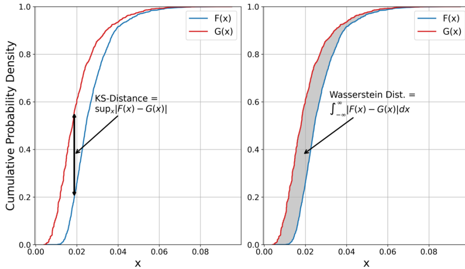
825 Figure 15. Definition of the Kolmogorov-Smirnov (KS) statistic (left) and Wasserstein Distance (right) with respect to empirical CDFs F(x) and G(x)
