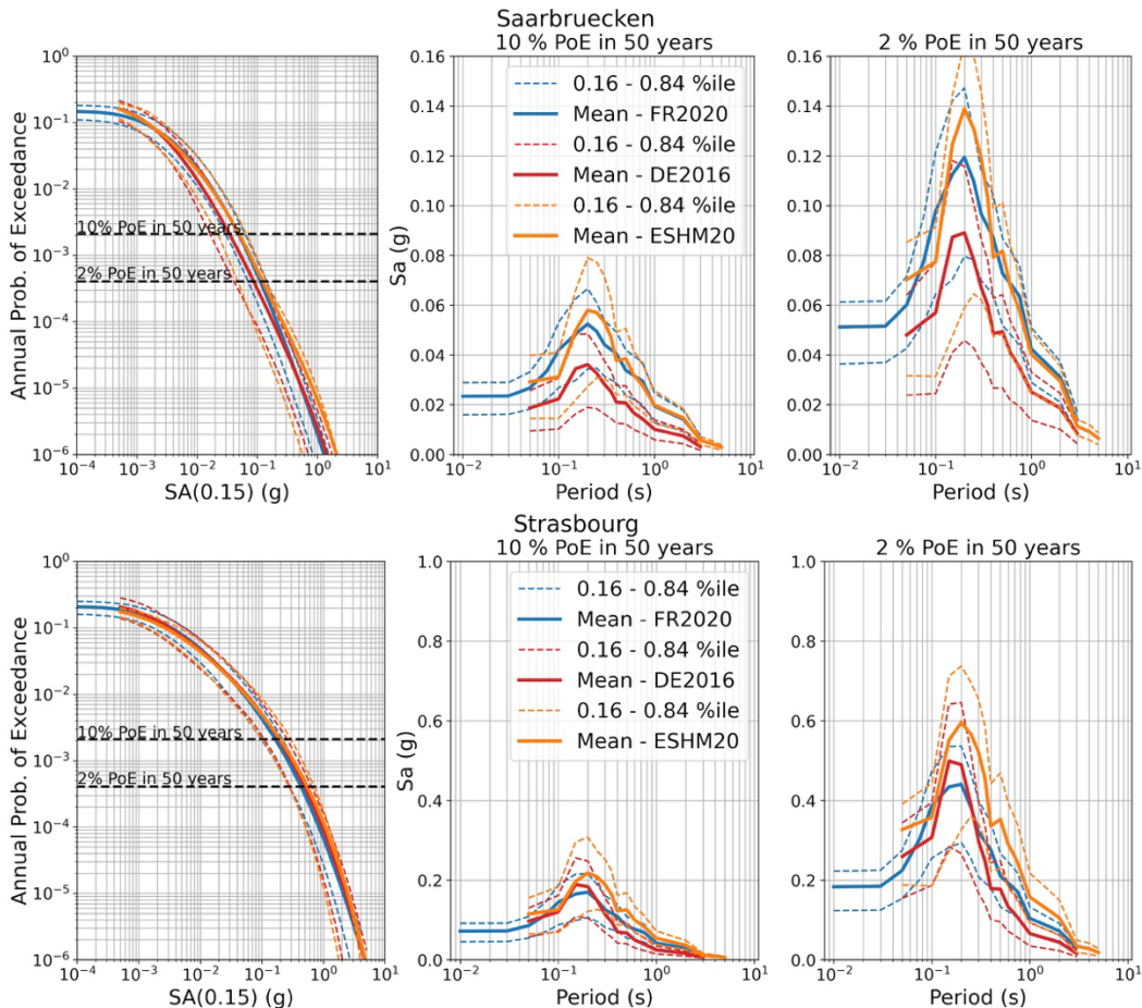
Figure 21. Comparison of the distributions of seismic hazard for Saarbrücken (top row) and Strasbourg (bottom row) for hazard curves at S_a(0.15\text{ s}) (left column) and UHS for 10 % PoE in 50 years (middle column) and 2 % PoE in 50 years (right column)
