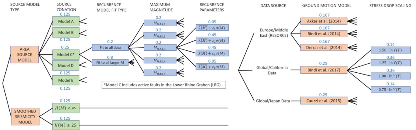
Figure 1. Complete logic tree of seismogenic source models (left) and ground motion models (right) for DE2016 (Grünthal et al. 2018)
