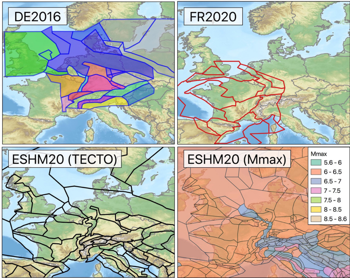
320 Figure 4: Large-scale area source zonation (LASZ) assumed for DE2016 (top left), FR2020 (top right) and the two LASZ zonation for ESHM20 based on regional tectonics (bottom left) and maximum magnitude (bottom right). Colours for DE2016 indicate the groupings of LASZ (from Model A) sharing a common b-value.
