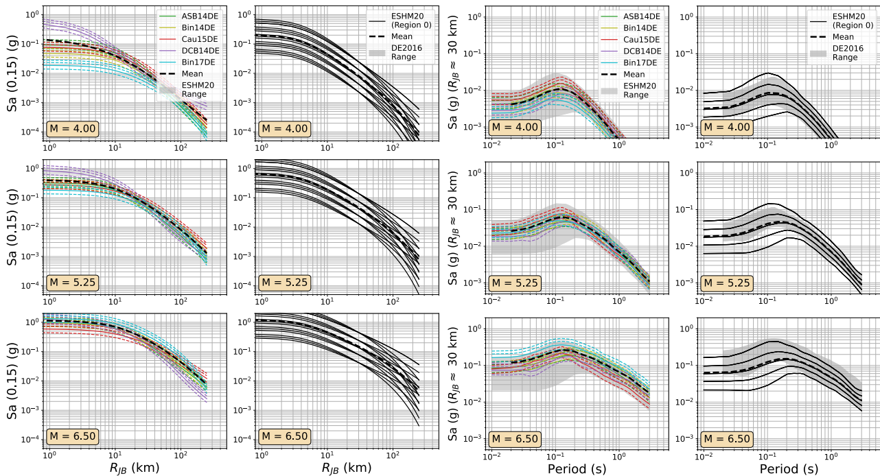
550 Figure 9: As Figure 6, comparing the median ground motions ESHM20 and DE2016 GMM logic trees
