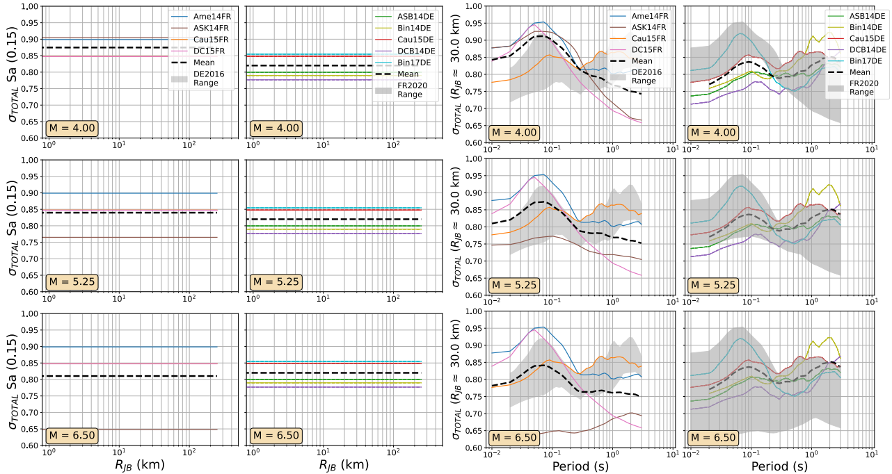
Figure 7: As Figure 6, comparing the aleatory uncertainty distributions of the FR2020 and DE2016 GMM logic trees. The dashed black lines refer to the sum of the aleatory variabilities of each GMM ( \sigma_i ) weighted by their logic tree weight ( w_i ): \sum_i(\sigma_i \cdot w_i)
