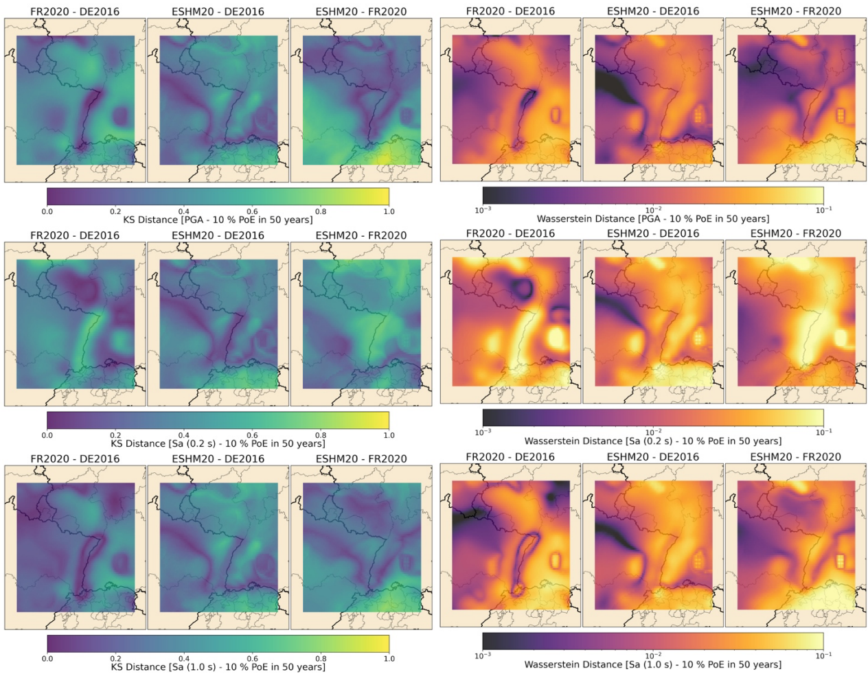
925 Figure 19: Spatial variation in the dissimilarity between distributions of seismic hazard values for a 10 % PoE in 50 years for PGA (top row), Sa (0.2 s) (middle row) and Sa (1.0 s) (bottom row) using KS Distance (left column set) and Wasserstein Distance (right column set)
