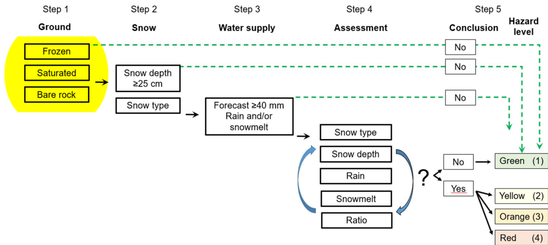
235 Figure 2: Flow chart of the slushflow hazard assessment process
