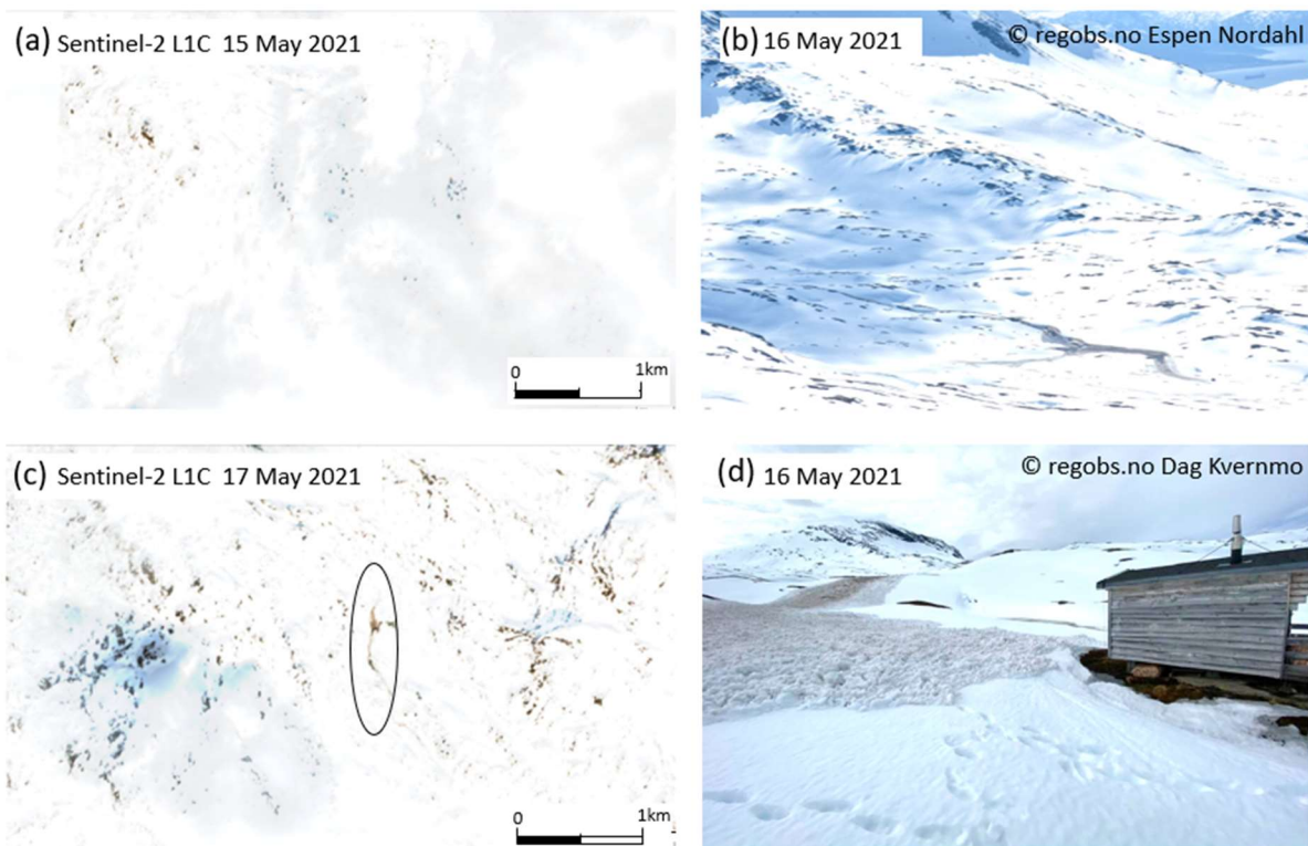
445 Figure 4: Snowmelt situations generally cause substantial changes of the snow cover and slushflows are often challenging to extract from multi-temporal satellite images. The slushflow at Leigassletta, Nordland, Norway 16 May 2021 is an exception with its long runoff and distinct shape. It also occurred at a time of a favourable temporal resolution (of the satellite images). (a) Copernicus Sentinel-2 L1C satellite image 15 May 2021 prior to the slushflow. (b) Parts of the slushflow released on 16 May 2021, seen from a 450 distance. Photo: Espen Nordahl, Regobs.no Copernicus Sentinel-2 L1C satellite image 17 May 2021, the slushflow in black oval. (c) Copernicus Sentinel-2 L1C satellite image 17 May 2021, parts of the slushflow in black oval. The slushflow released on 16 May 2021, seen from distance Photo: Espen Nordahl, Regobs.no (d) Close-up photo of the slushflow on 16 May 2021 Photo: Dag Kvernmo, Regobs.no
