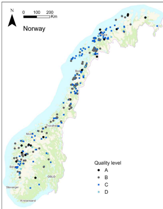
470 Figure 5: Reported and quality-controlled slushflows in Norway in the period 2013-2023. There are 152 events of quality A and B and totally 394 slushflows (Source: www.skrednett.no. Accessed 12 June 2023). Map source: The Norwegian Mapping Authority, Geovekst – Geodata AS.
