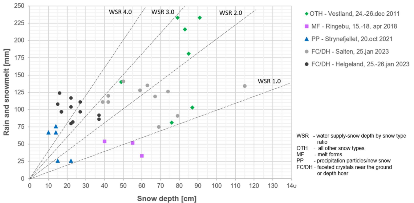
510 Figure 6: An example, dDistribution of reported slushflows according to snow type, and modelled snow depth and water supply (i.e., rain and snow melt) 1-3 days before the events.
