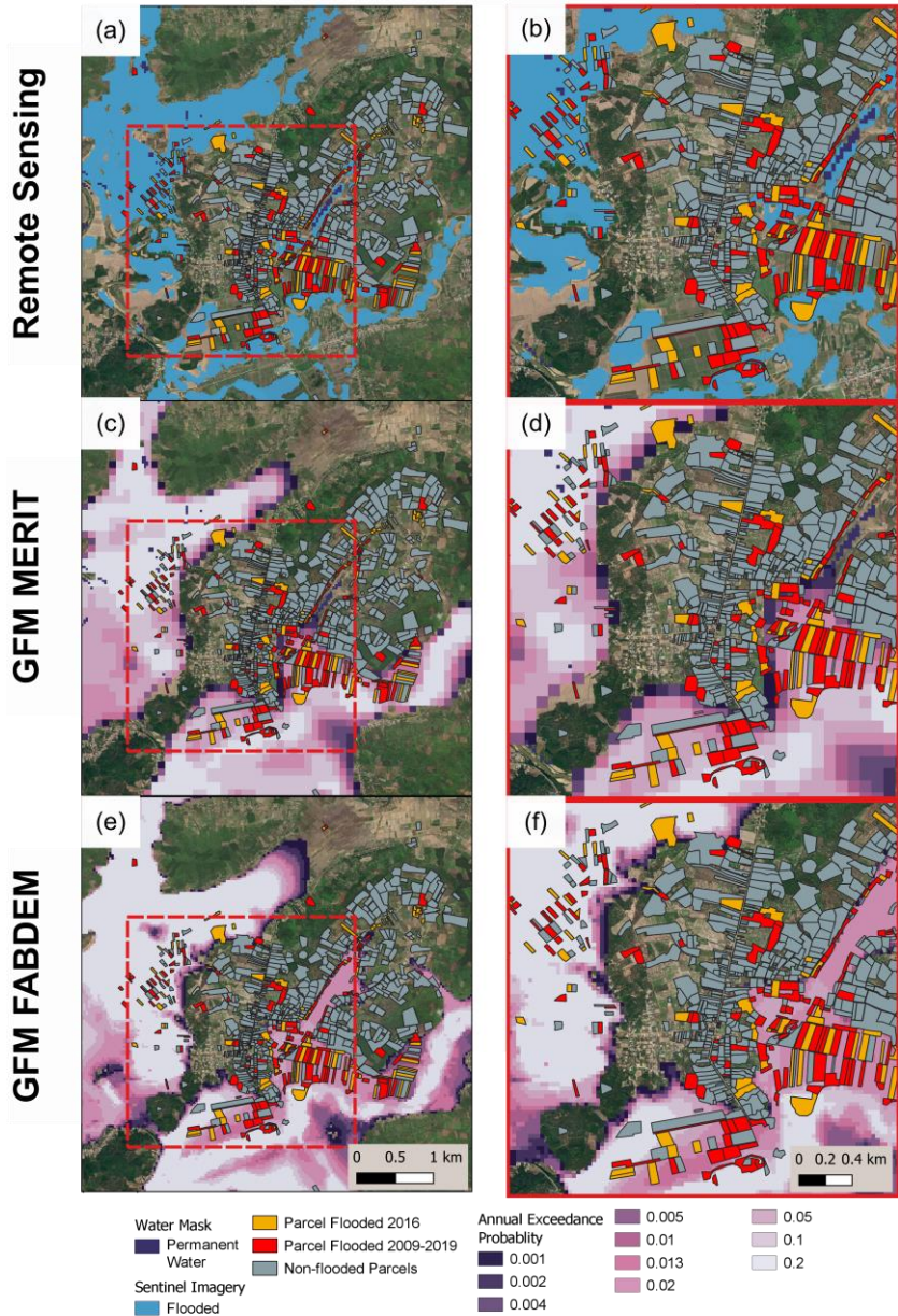
570 Figure 7: Flood Maps for Thon 6 Vu Bon. Panel (a) shows flood extent from 2016 acquired from Sentinel 1 data. Panel (c) shows annual exceedance probability (AEP) for GFM V2, and panel (e) shows AEP for GFM V3. Panels (b), (d) and (f) show zoomed in versions of the remote sensing and GFM outputs.
