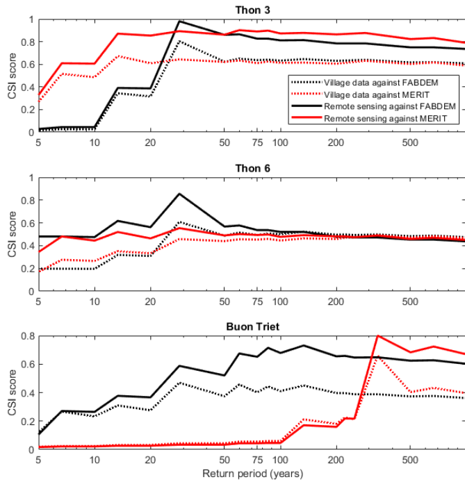
580 Figure 9: Critical success index scores by return period against remotely sensed (solid lines) and household survey (dotted lines) validation data for MERIT (red) based GFM and FABDEM (black) based GFM. The return period on the x-axis refers to the flood return period from the GFM.
