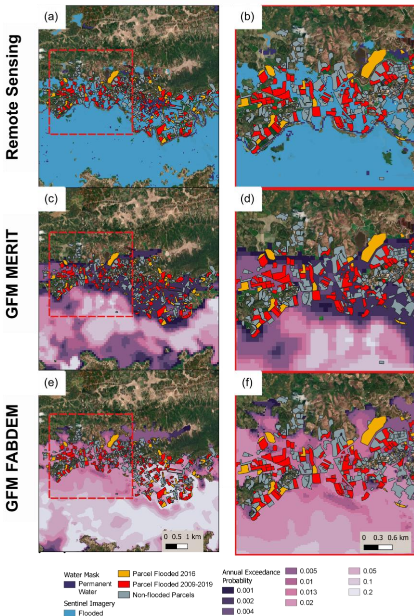
575 Figure 8: Flood Maps for Buon Triet. Panel (a) shows flood extent from 2016 acquired from Sentinel 1 data. Panel (c) shows annual exceedance probability (AEP) for GFM V2, and panel (e) shows AEP for GFM V3. Panels (b), (d) and (f) show zoomed in versions of the remote sensing and GFM outputs.
