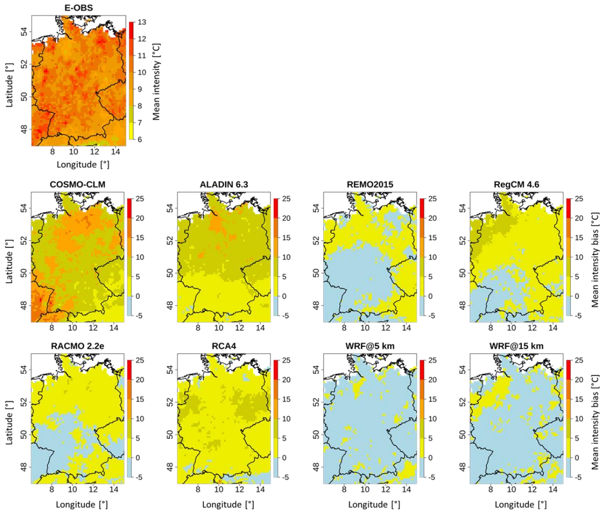
360 Figure 6. Grid cell based E-OBS summer mean heat wave intensity pattern between 1980–2009 and differences between each RCM and E-OBS.
