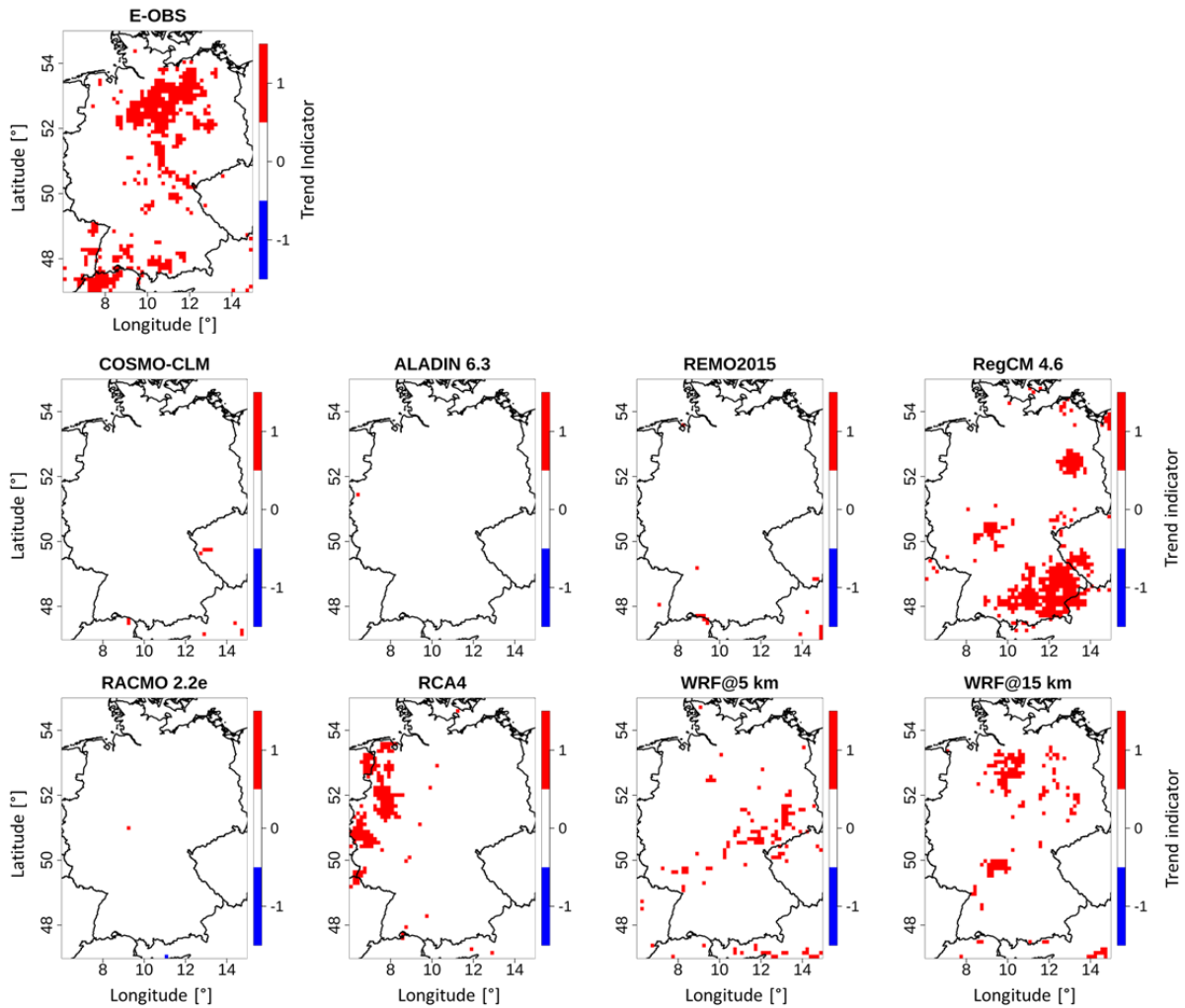
410 Figure 7. Grid cell based trends of the number of annual summer heat waves for 1980–2009 based on the Mann-Kendall Test for E-OBS and each RCM.
