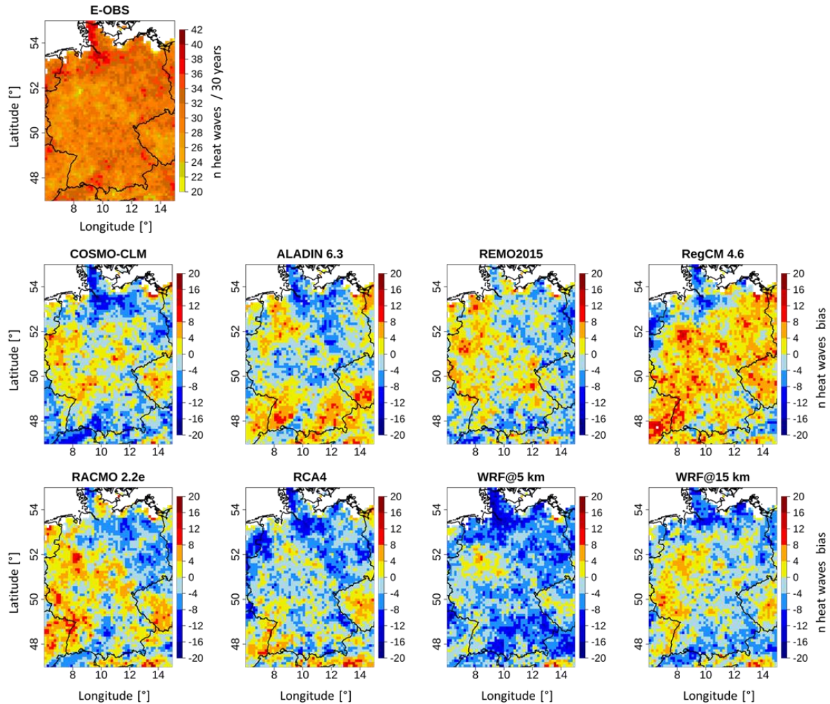
Figure 4. Grid cell based E-OBS summer heat wave frequency pattern between 1980–2009 and differences between each RCM and E-OBS.
