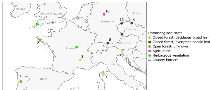
195 Figure 3. Overview on the twelve selected locations European catchments
