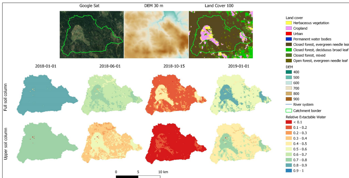
Figure 5. Beginning, propagation and recovery of the 2018 drought on HRU scale in the Natzschung catchment for the root zone (0.45 m) and full soil column (up to 2 m). Reference to satellite imagery: Imagery 2023 TerraMetrics, Map Data 2023, GeoBasis-DE/BKG 2009. Reference to elevation model: NASA Shuttle Radar Topography Mission Global 1 arc second, 2023. Reference to land cover map - Copernicus Global Land Service: Land Cover 100m: collection 3
