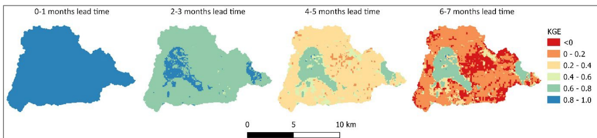
Figure 9. Kling-Gupta Efficiency values for full-column (up to 2 m) daily soil moisture (2017-2020) calculated between simulations with ERA5 and SEAS5 ensemble hindcasts (1, 3, 5 and 7 months lead time) forcings in the Natzschung catchment
