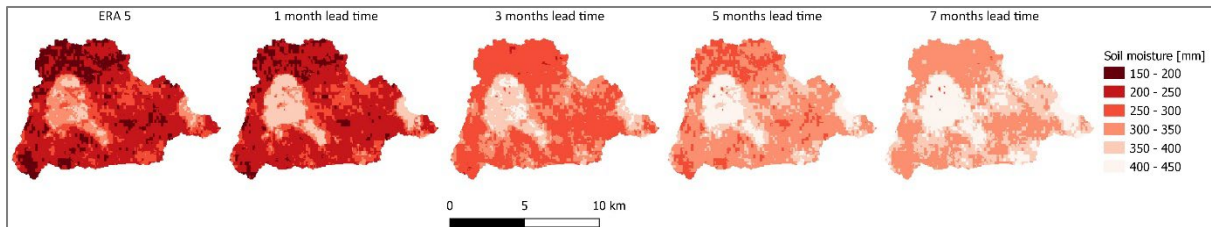
Figure 8. Full-column (up to 2 m) mean monthly soil moisture in October 2018 simulated with ERA5 and SEAS5 ensemble hindcasts (1, 3, 5 and 7 months lead time) forcings in Natzschung catchment. SEAS5-forced runs are represented with the ensemble mean.
