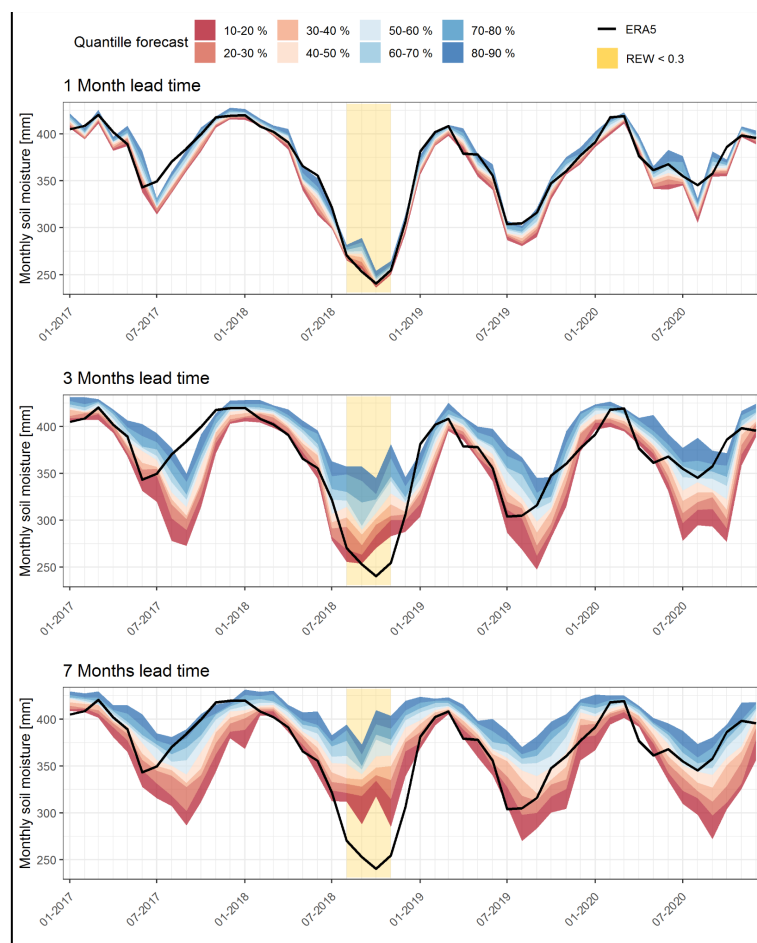
Figure 12. Monthly averages of a catchment-mean full-column (up to 2 m) soil moisture simulated with ERA5 and SEAS5 hindcasts forcings in the Natzschung catchment
