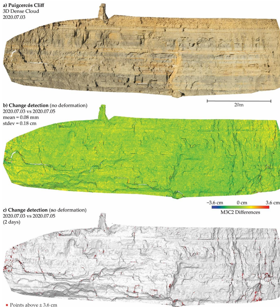
Figure 5. a) Point cloud obtained with the very high-resolution photogrammetric system installed in Puigercós (obtained with MEMI workflow). b) M3C2 (Lague et al., 2013) comparison of two consecutive days (no expected deformation). c) Same comparison than in b) highlighting in red the points with a deformation higher than 0.036 m.
