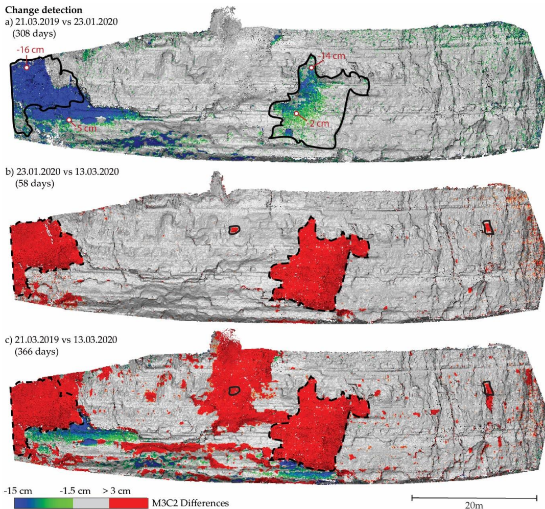
Figure 6. Examples of pre-failure deformations and rockfalls detected. a) Accumulated pre-failure deformation of two active blocks after 308 days. The comparison has been done with the M3C2 algorithm and the MEMI workflow. b) Change detection obtained 58 days after the detection of pre-failure deformation shown in a), with the two detached blocks identified in red. c) Change detection after approximately one year. The red clusters identify rockfalls, while the green-blue areas indicate pre-failure deformation. For all results 0.015 m has been used as level of detection.
