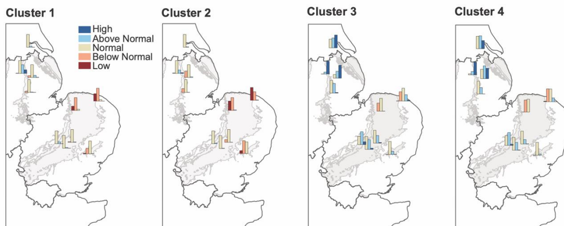
310 Figure 9: Outlook of groundwater levels for each borehole in different categories (percentiles relative to 1965-2015) by spring 2023 for each storyline. Individual plots show the distribution of hindcast winters for each percentile category as indicated by the colour key in Figure 3. Grey shading shows major aquifers in eastern England from the hydrogeology map of the British Geological Survey ( https://www.bgs.ac.uk/datasets/hydrogeology-625k/ ).
