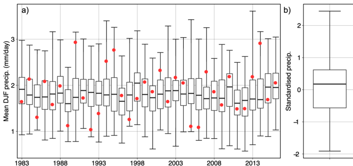
110 Figure 1 (a) Observed (CEH-GEAR) and simulated mean winter (DJF) rainfall over 1983-2016 from the SEAS5 hindcasts across 25 ensemble members and three lead times over the East Anglia region. The whiskers of the boxplots extend to the maximum and minimum modelled value. (b) Distribution of observed winter rainfall for each year over the 1983-2016 period standardised against the distribution of simulated rainfall of the same year.
