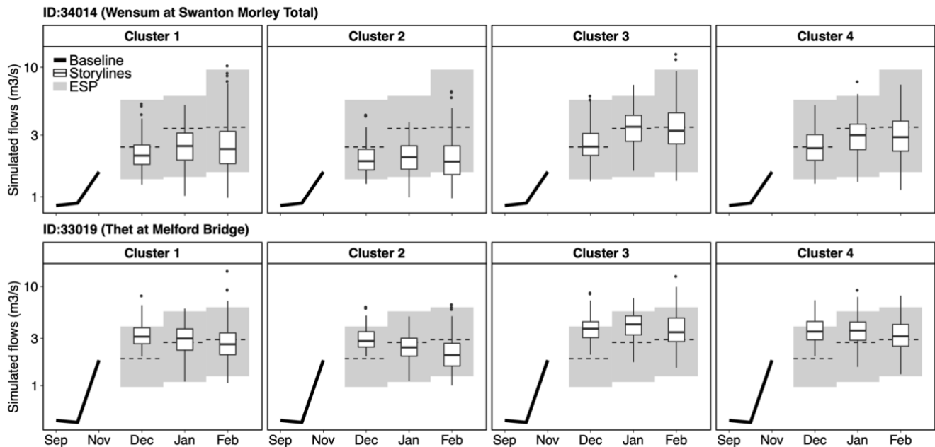
Figure 7 Simulated river flows at two example catchments for each circulation storyline over winter 2022/23. The shading indicates the range of outcomes obtained from the standard ESP method by assuming the repetition of historical years (1965-2017) and the dotted line is the mean of the ESP outcomes.
