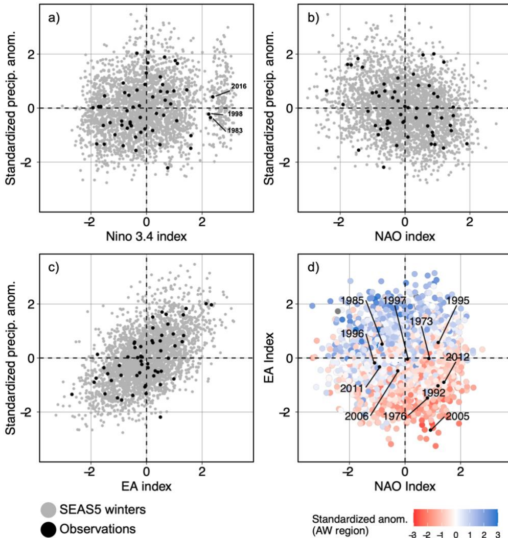
155 Figure 3: Relationship of a) Niño 3.4, b) NAO, and c) EA index with standardised rainfall anomalies in East Anglia for the SEAS5 winters (grey) and observed winters (black). Panel d) shows the NAO index and EA index for each SEAS5 winter together with the rainfall anomalies over East Anglia associated with each winter (colours). The cluster of strong El Niño hindcast winters in panel a) relate to hindcast winters issued prior to winters 2015/16, 1997/98 and 1982/83 (black dots in panel a), which were three of the strongest El Niño winters in the observations. Selected dry winters in the observations are shown in panel d) by the black dots and the year labels.
