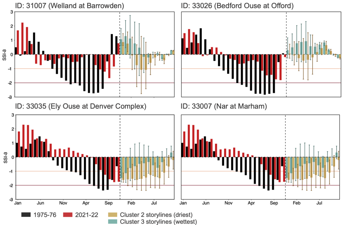
Figure 8: Standardised streamflow index accumulated at 3-months (SSI-3) over 2021-2022 and beyond following the driest and wettest circulation storyline at four example catchments compared with SSI-3 over 1975-1976. Spring to autumn 2023 is assumed to have 100% LTA rainfall.
