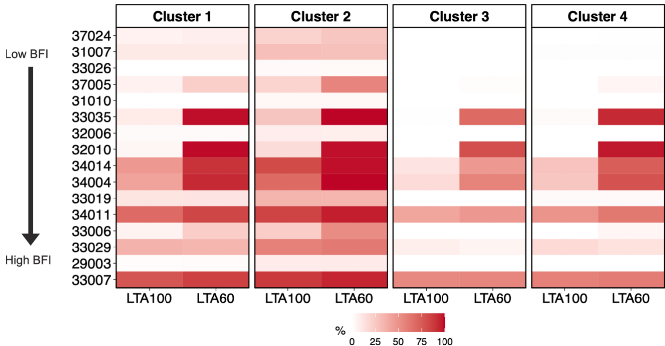
325 Figure 10: Likelihood of reaching SSI-3 below -1.5 from winter 2022/23 to autumn 2023 for each circulation storyline. In the LTA100 experiment, spring to autumn 2023 are assumed to have rainfall at 100% long term seasonal average whereas the LTA60 experiment assumes summer 2023 to receive 60% LTA rainfall with 100% LTA rainfall for the other seasons. Catchments are ordered by increasing baseflow index (BFI) from the top.
