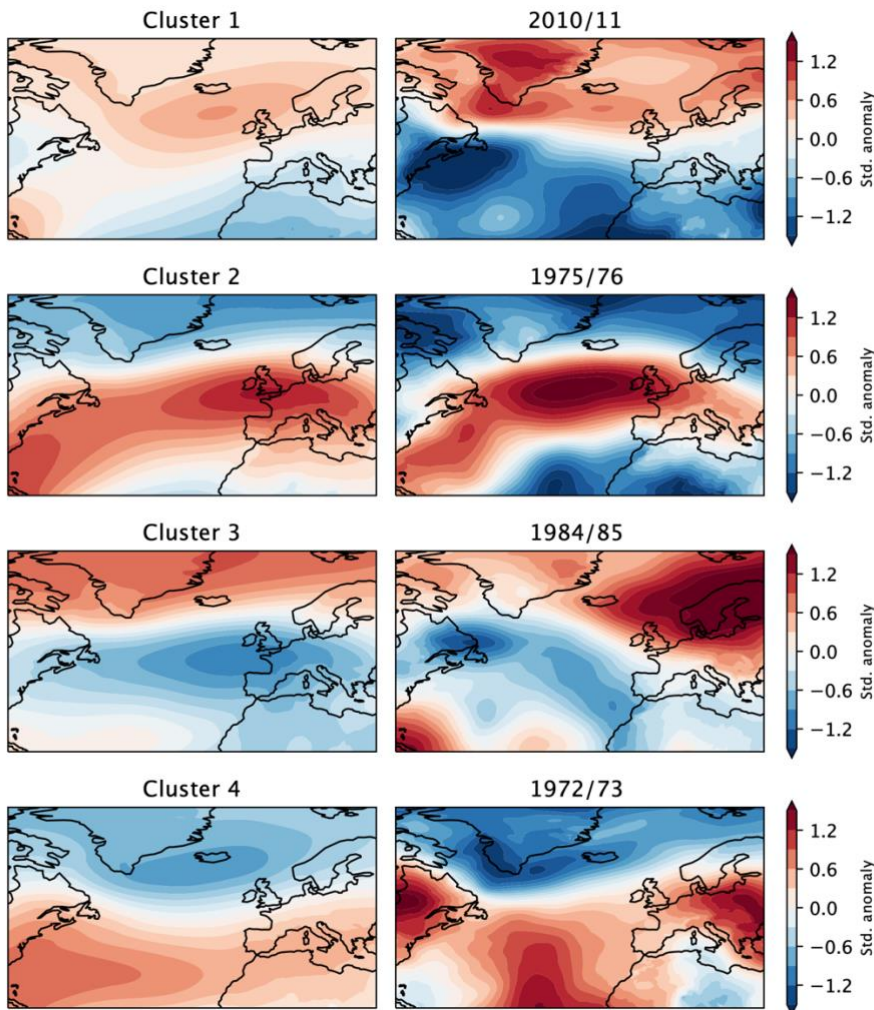
190 Figure 5: Composite mean sea level pressure (SLP) anomalies (relative to ERA5 1960-2015) for the four circulation storylines and SLP anomalies for selected dry winters from ERA5 associated with similar patterns for each cluster.
