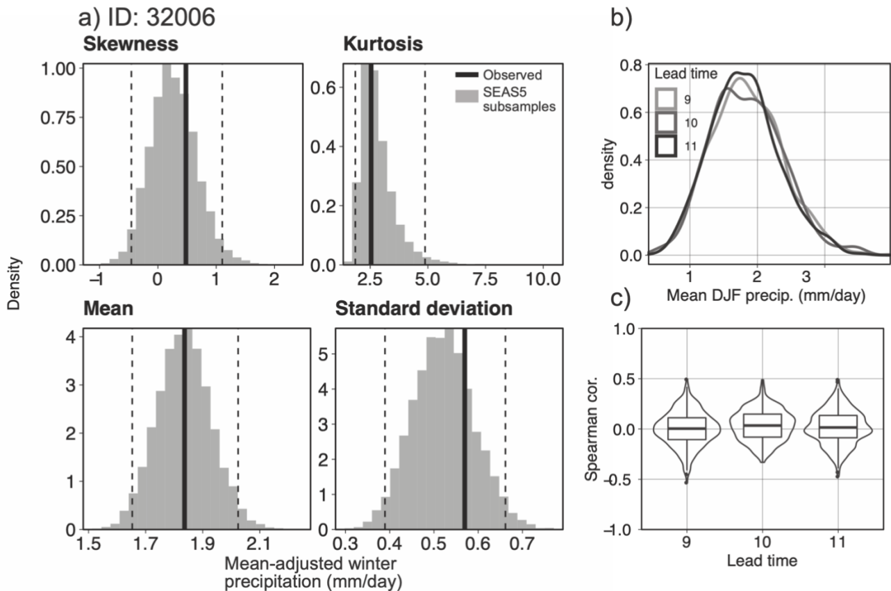
130 Figure 2: Example of the model fidelity test for one catchment (ID: 32006). a) The statistical moments of observed DJF rainfall and of 10,000 subsamples of the modelled rainfall in SEAS5. Hindcast winters are scaled to match the mean observed rainfall. b) Test for model stability and c) ensemble member independence across three lead times.
