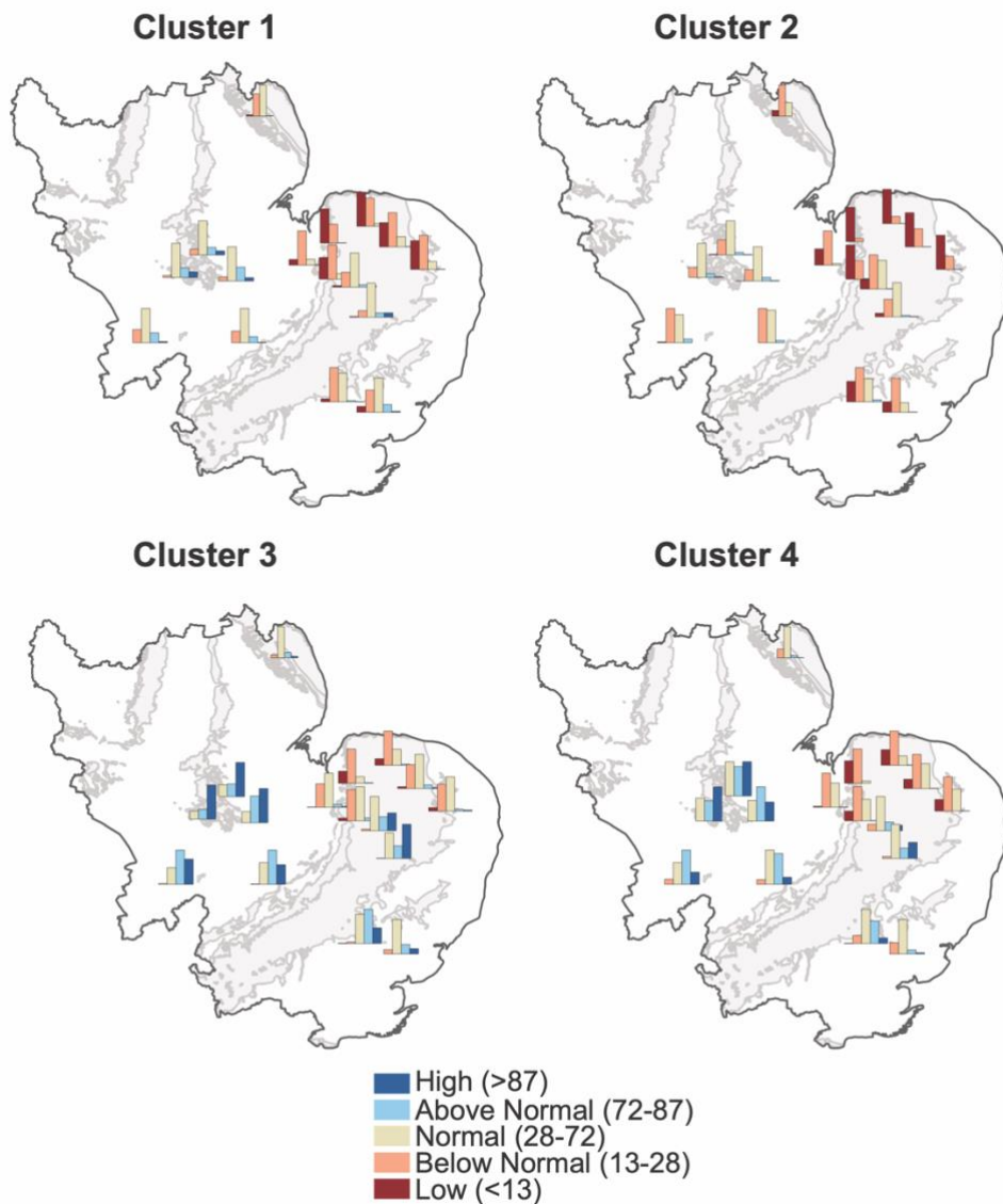
270 Figure 6: Outlook of river flows for each storyline represented in percentile terms relative to 1965-2015. Each storyline assume winter 2022/23 follows hindcast winters in one of the La Niña winter clusters. Individual plots show the distribution of hindcast
