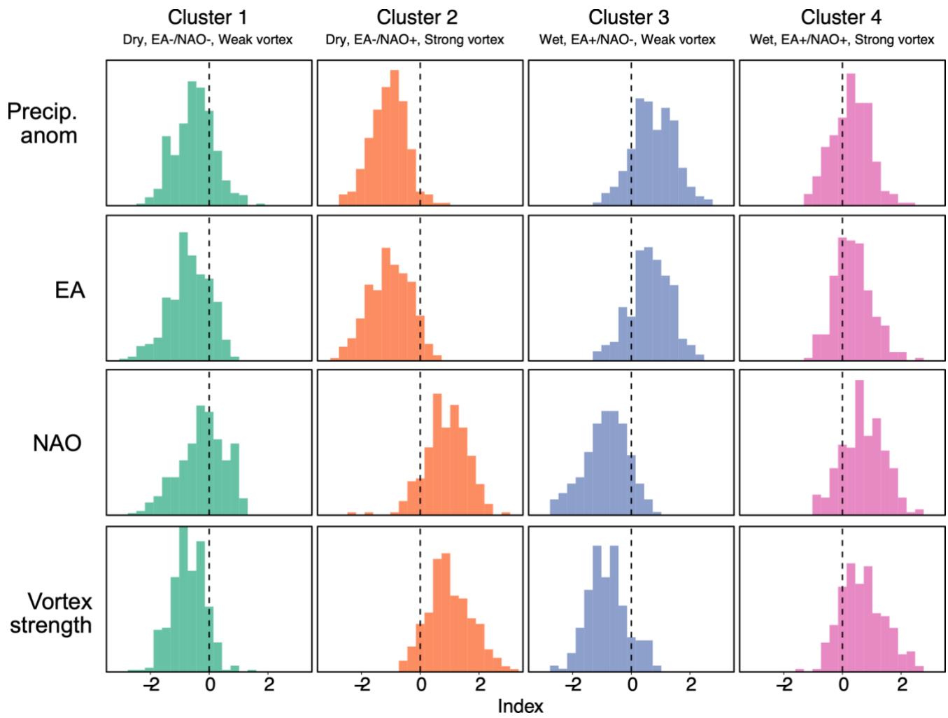
185 Figure 4: Winter clusters defined from hindcast winters with La Niña conditions using k-means clustering and the standardised rainfall anomalies and meteorological indices associated with each cluster.
