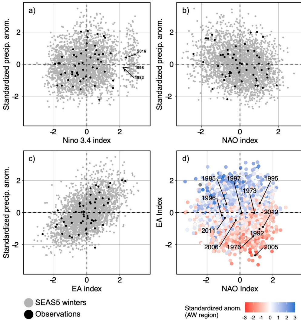
Figure 3: Relationship of a) Niño-3.4, b) NAO, and c) EA index with standardised rainfall anomalies in East Anglia for the SEAS5 winters (grey) and observed winters (black). Panel d) shows the NAO index and EA index for each SEAS5 winter together with the rainfall anomalies over East Anglia associated with each winter (colours). The cluster of strong El Niño hindcast winters in panel a) relate to hindcast winters issued prior to winters 2015/16, 1997/98 and 1982/83 (black dots in panel a), which were three of the strongest El Niño winters in the observations. Selected dry winters in the observations are shown in panel d) by the black dots and the year labels.
