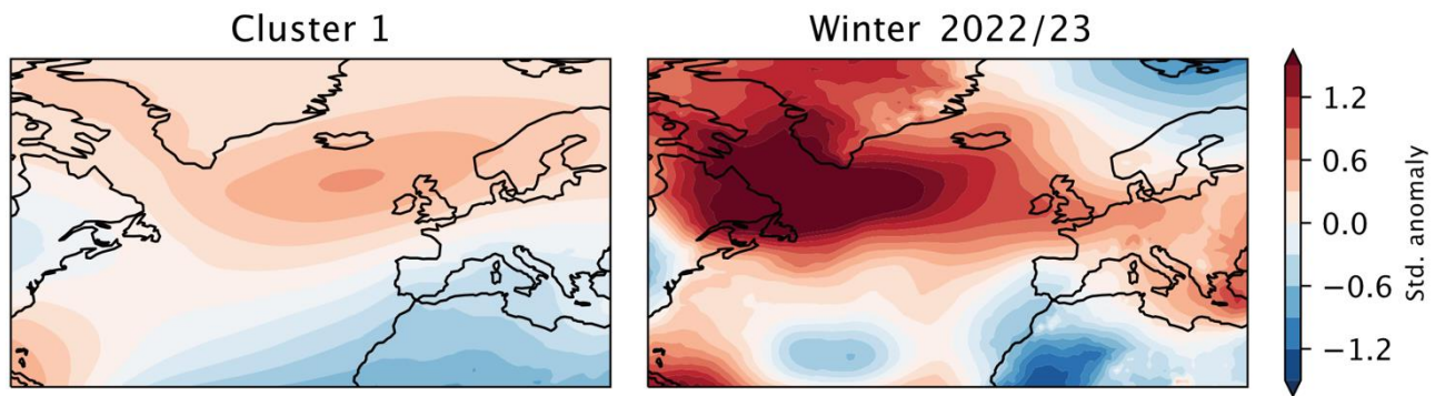
410 Figure 11 Composite mean sea level pressure anomalies for winters in cluster 1 of the SEAS5 winters (left) compared to mean sea level pressure anomalies over observed winter 2022/23 (right: data from ERA5)
