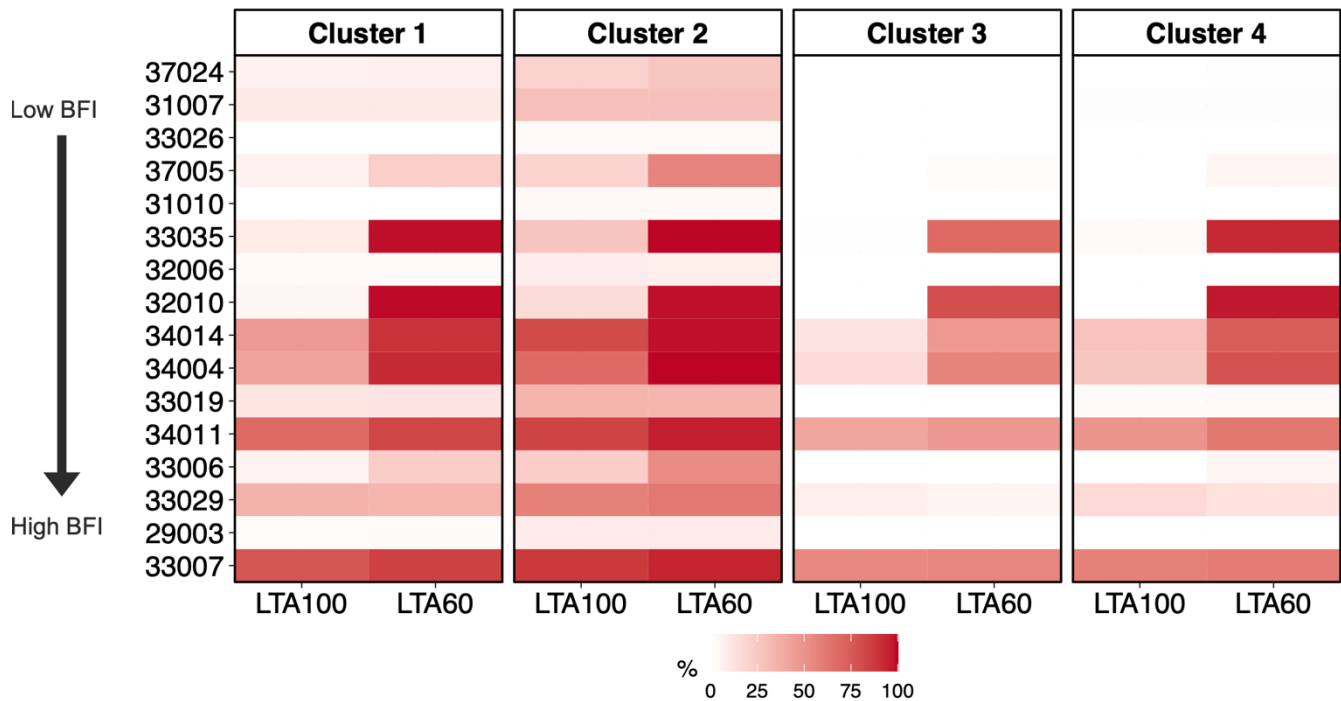
330 Figure 10: Likelihood of reaching SSI-3 below -1.5 from winter 2022/23 to autumn 2023- for each circulation storyline. In the LTA100 experiment, spring to autumn 2023 are assumed to have rainfall at 100% long term seasonal average whereas the LTA60 experiment assumes summer 2023 to receive 60% LTA rainfall with 100% LTA rainfall for the other seasons. Catchments are ordered by increasing baseflow index (BFI) from the top.
