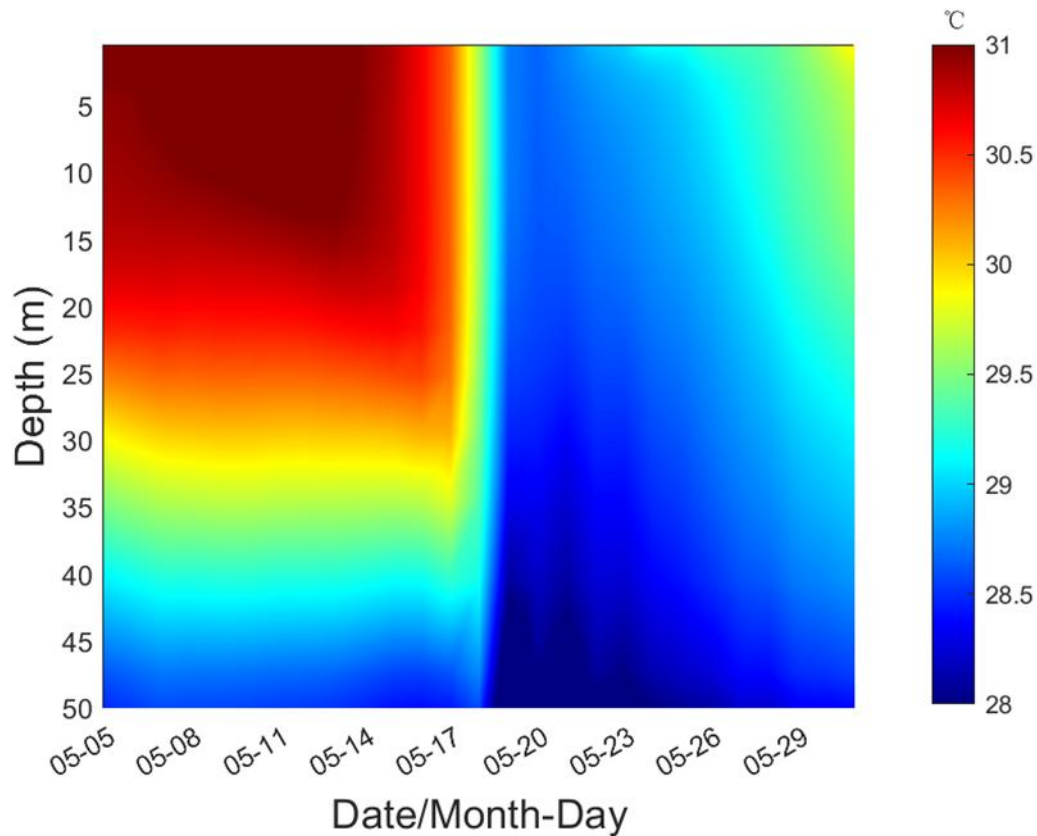
165 Figure 6: Time series of vertical water temperature from May 5 to 31 in Box A.
