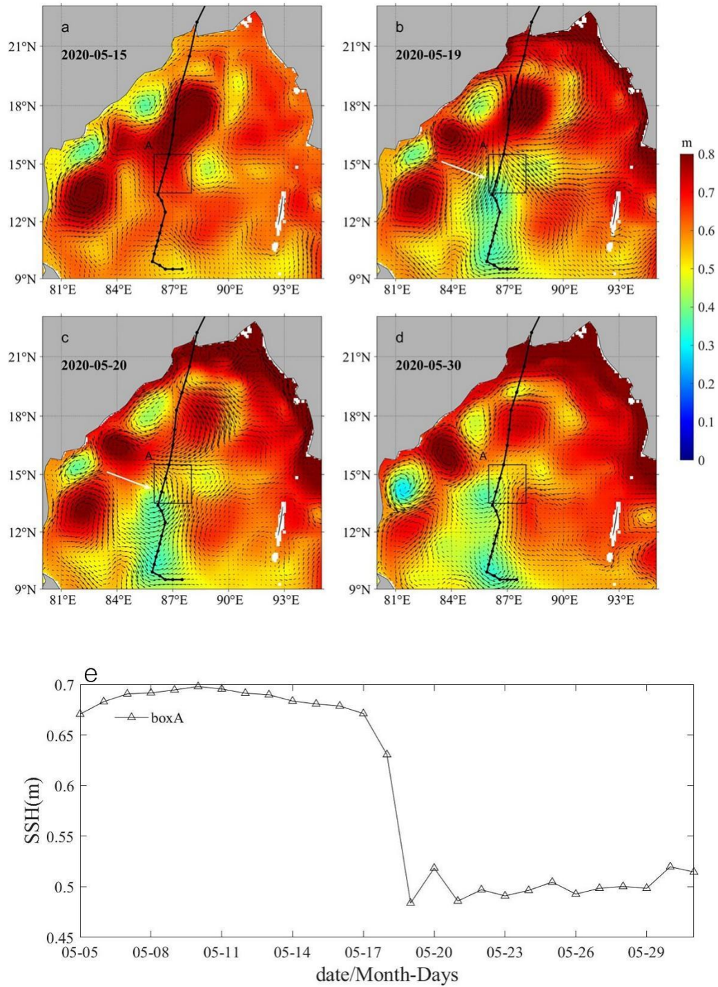
Figure 5: Sea surface current (unit in \text{m}\cdot\text{s}^{-1} ) on May 15 (a), May 19 (b), May 20 (c) and May 30 (d). Time series of SSH in Box A (e). The color bar represents the SSH (unit in m). The track of Amphan is marked by the black line.
