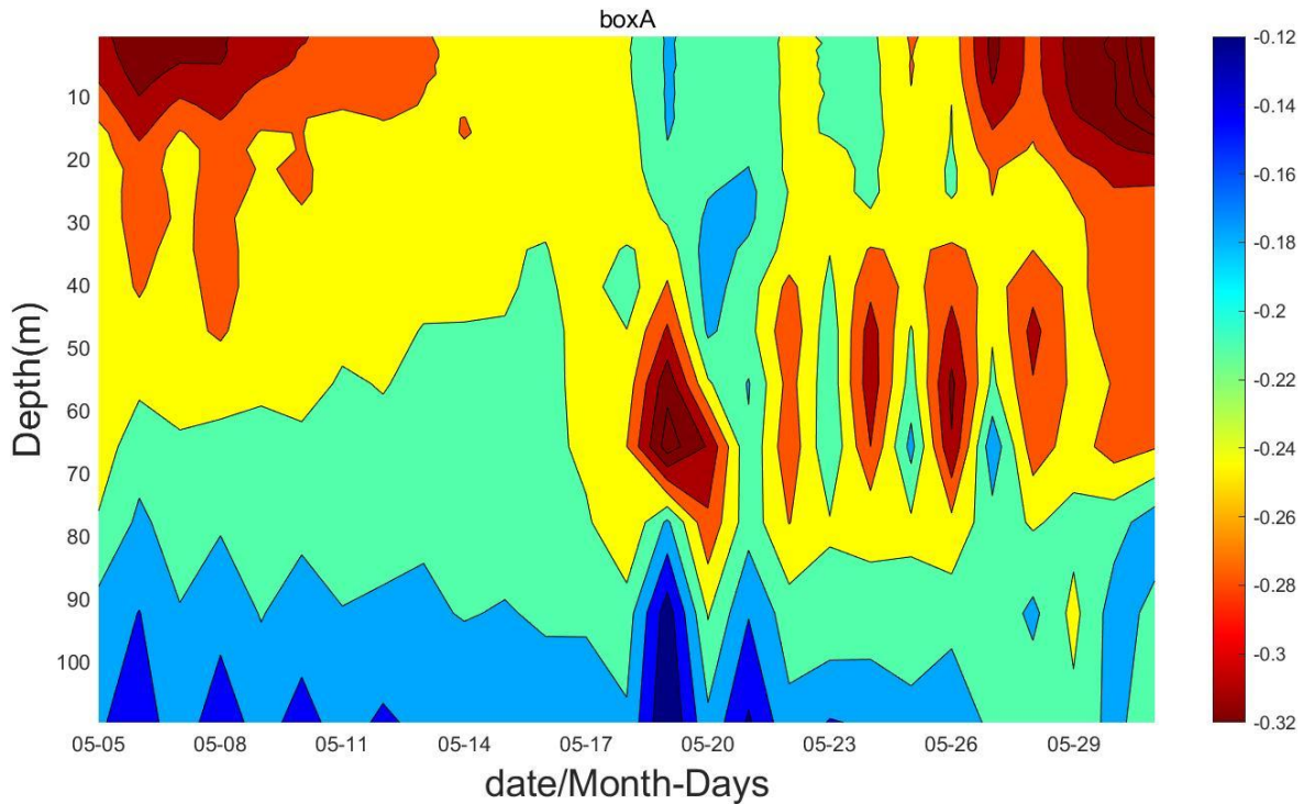
225 Figure 12: Time series of spatially averaged vorticity in Box A from May 5 to May 31.
