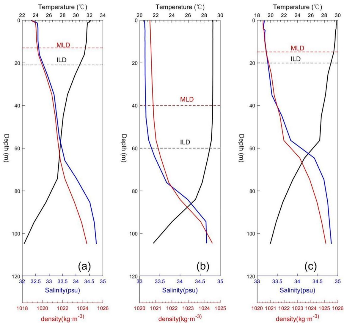
200 Figure 9: Barrier layer thickness calculated from Argo data in Box A on May 8 (a), 18 (b), and 28 (c).
