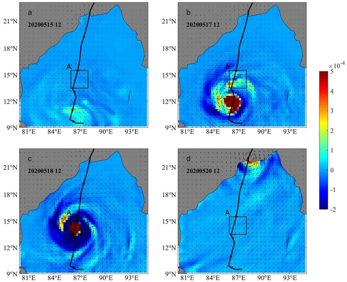
Figure 11: Surface wind speed (arrows) and EPV (colors) during the period time of the TC.
