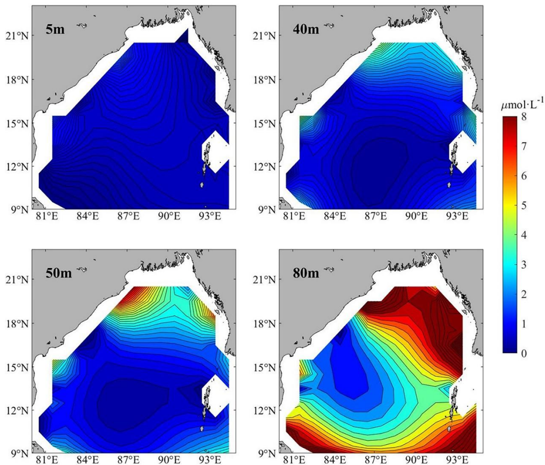
175 Figure 7: Distribution of nitrate concentration (unit in \mu\text{mol}\cdot\text{L}^{-1} ) in May from the WOA.
