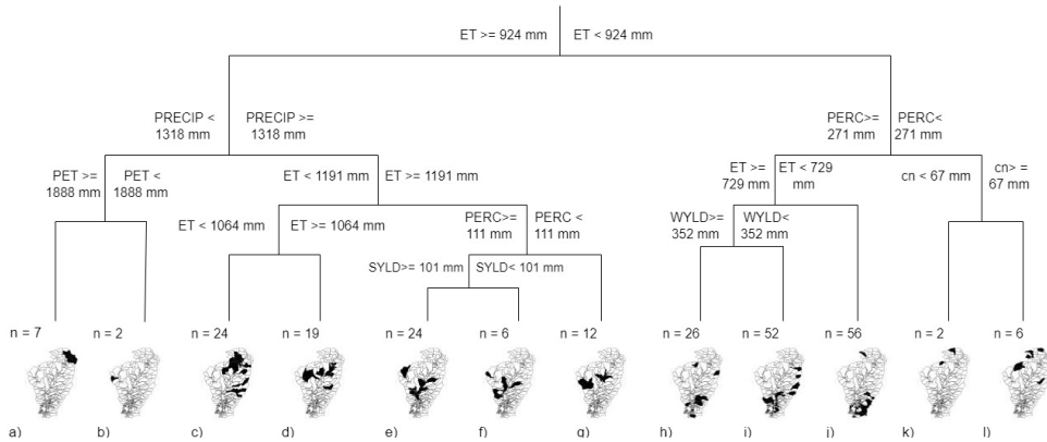
505 Figure 7 MVRT of hydroclimatic drivers of agricultural droughts at the Cesar River basin, and spatial distribution of the subbasins clustered at each leaf. Tree leaves are named from a to l and n indicates the number of subbasins clustered at each leaf.
