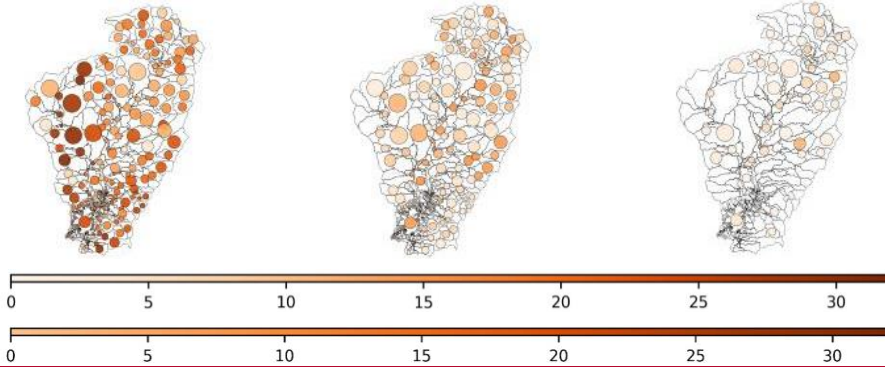
Figure 56 Months counted in the hydrological droughts category: a) moderate, b) severe and c) extreme.
