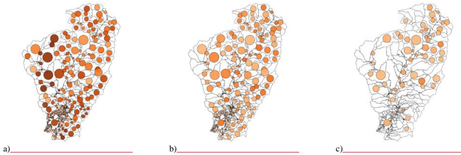
405 Figure 45 Months counted in each agricultural droughts category: a) moderate, b) severe and c) extreme. SMDI was not calculated in the wetland subbasins (i.e. hatched area).
