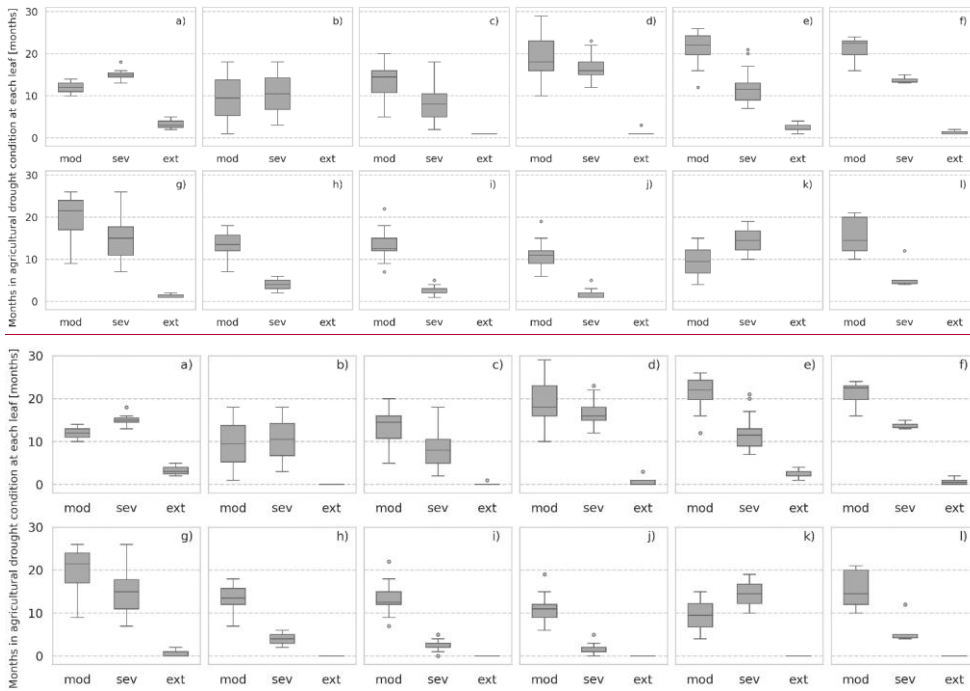
510 Figure 68 Number of months in agricultural drought categories (moderate, severe, extreme) at each leaf. Tree leaves are named from a to l .
