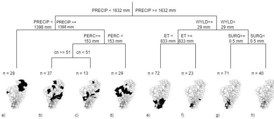
580 Figure 79 MVRT of hydroclimatic drivers of hydrological drought at the Cesar River basin, and spatial distribution of the subbasins clustered at each leaf. Tree leaves are named from a to h and n indicates the number of subbasins clustered at each leaf.
