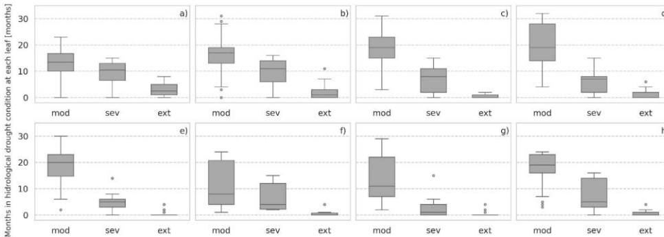
585 Figure 810 Months in agricultural-hydrological drought categories (moderate, severe, extreme) at each leaf. Tree leaves are named from a to h .
