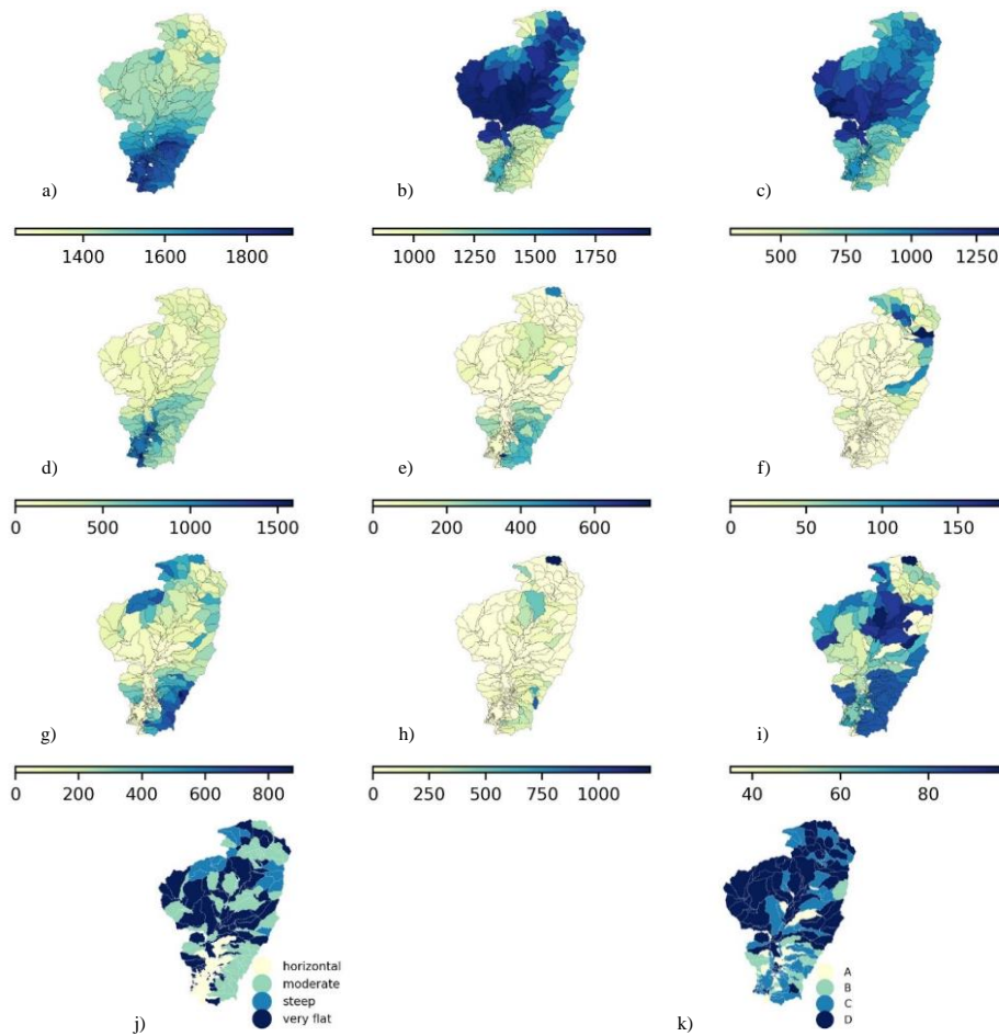
Figure 34 Average value of hydroclimatic parameters during the simulation period at each subbasin: a) precipitation in mm, b) potential evapotranspiration in mm, c) actual evapotranspiration in mm, d) percolation in mm, e) surface runoff in mm, f) groundwater contribution to streamflow in mm, g) water yield in mm, h) sediment yield in metric tons/ha, i) curve number, j) slope and k) soil type.
