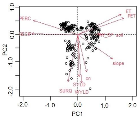
a) b) Figure 7 Loading factors of the eleven hydroclimatic parameters for the first three PCs (a) and the biplot of the first two PCs (b).
