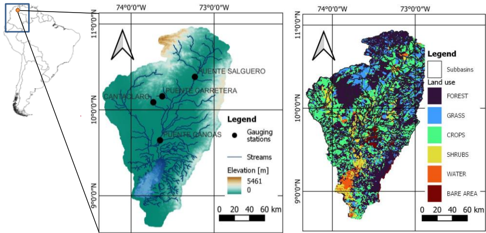
Figure 2 Cesar River basin topography and land use
