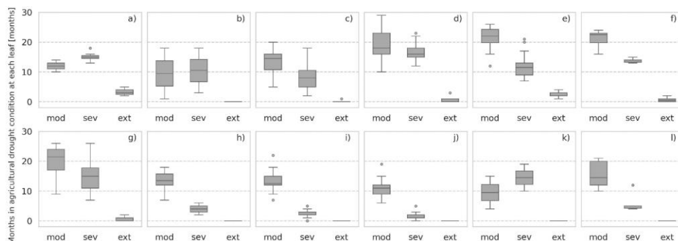
Figure 8 Figure 9 Number of months in agricultural drought categories (moderate, severe, extreme) at each leaf. Tree leaves are named from a to l. Number of months in agricultural drought categories (moderate, severe, extreme) at each leaf.
