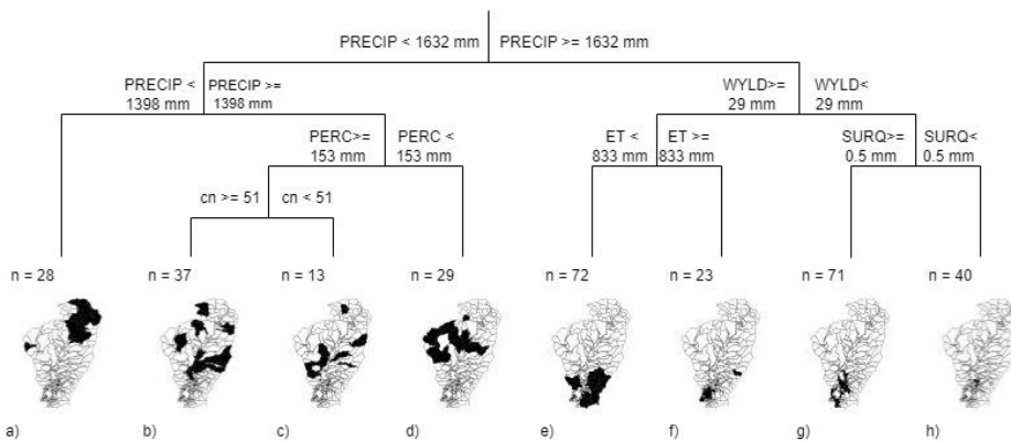
Figure 9 Figure 10 MVRT of hydroclimatic drivers of hydrological drought at the Cesar River basin, and spatial distribution of the subbasins clustered at each leaf. Tree leaves are named from a to h and n indicates the number of subbasins clustered at each leaf. MVRT of hydroclimatic drivers of hydrological drought at the Cesar River basin, and spatial distribution of the subbasins clustered at each leaf.
