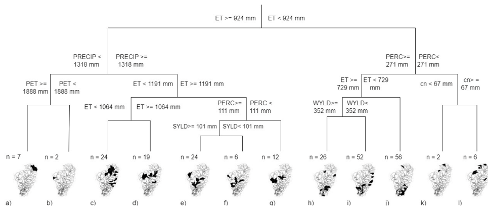
Figure 7 Figure 8 MVRT of hydroclimatic drivers of agricultural droughts at the Cesar River basin, and spatial distribution of the subbasins clustered at each leaf. Tree leaves are named from a to l and n indicates the number of subbasins clustered at each leaf. MVRT of hydroclimatic drivers of agricultural droughts at the Cesar River basin, and spatial distribution of the subbasins clustered at each leaf.
