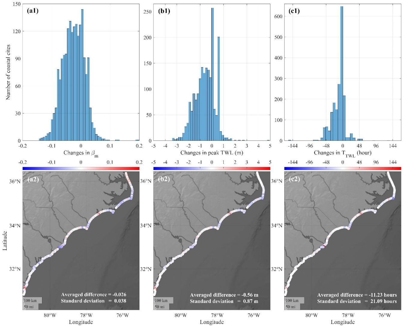
430 Figure 8. Histograms (top panels) and spatial distributions (bottom panels) of the differences of \beta_m , peak TWL , and T_{TWL} under pre- and post-Matthew conditions from Georgia to North Carolina coasts: a1, a2) \beta_m ; b1, b2) peak TWL ; c1, c2) T_{TWL} .
