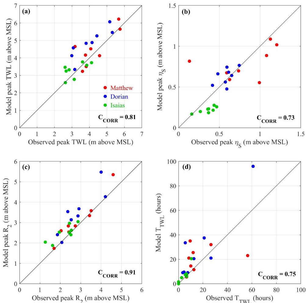
Figure 2. Model verification of (a) the peak TWL s, (b) the peak storm surge, (c) the peak wave runup, and (d) the maximum continuous duration of TWL \geq D_{base} ( T_{TWL} ) at eight NOAA tide gauges during the three historical hurricanes. The red, blue, and green points denote the data of hurricanes Matthew, Dorian, and Isaias, respectively. The corresponding correlation coefficients ( C_{CORR} ) are shown on the bottom-right corner in each panel.
