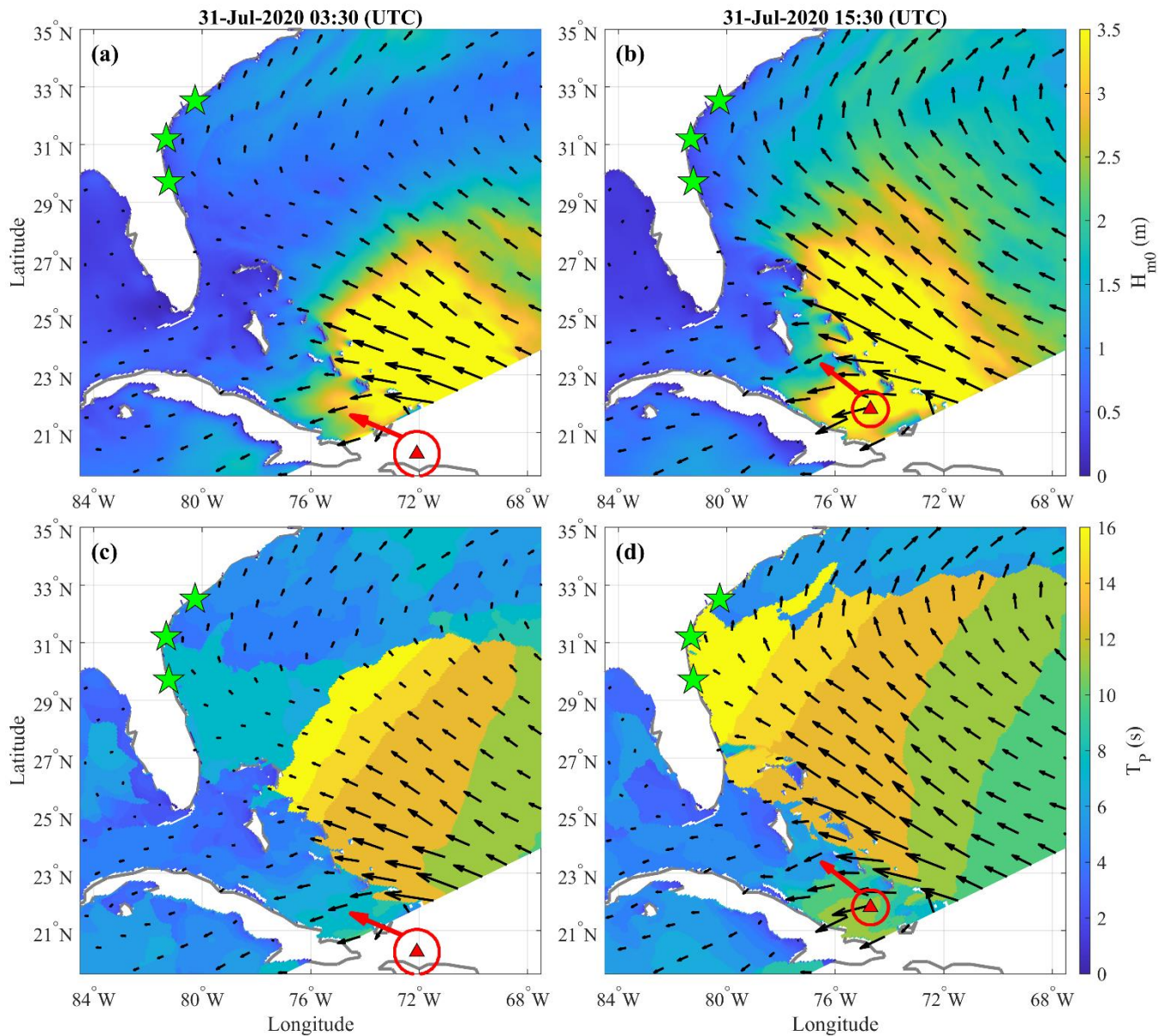
Figure 7. The propagation of the swells generated by Hurricane Isaias on its right-hand side. The green stars indicated the three selected barrier islands, i.e., Edisto Island, Sea Island, and the barrier island south of Matanzas Inlet (from North to South). The red triangles represented the eye of Isaias with the red circle denoting the instantaneous radius of maximum wind and the red arrow denoting the heading direction. The black arrows were the mean wave directions from COAWST simulation. The colormaps in panels (a) and (b) showed the distribution of H_{m0} at 03:30 UTC 31 July 2020 and 15:30 UTC 31 July 2020, respectively. The colormaps in panels (c) and (d) showed the distribution of T_p at 03:30 UTC 31 July 2020 and 15:30 UTC 31 July 2020, respectively.
