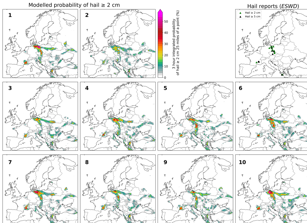
Figure 2. Probabilistic forecast of hail \geq 2 cm occurrence on 15 June 2019 at 12:00 UTC (initialized on 15 June 2019 at 00:00 UTC) for the individual ensemble members. Hail reports between 12:00 and 15:00 UTC are shown as triangles (green for hail \geq 2 cm but \leq 5 cm, black for hail \geq 5 cm) in the top-right panel.
