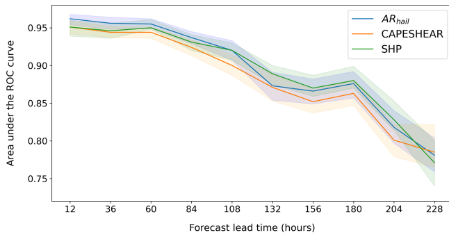
Figure 13. AUC depending on forecast lead time for AR_{\text{hail}} , CAPESHEAR and the significant hail parameter; 1000-member block bootstrap was performed to estimate 95 % AUC confidence intervals for each model (shaded).
